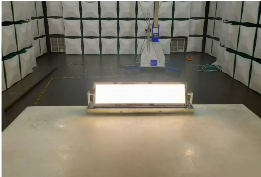
Radiated Disturbance below 1GHz
