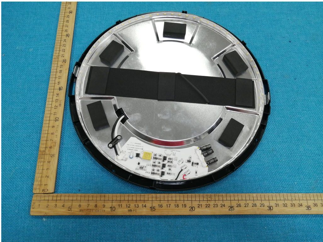
Model : PLU01R-1224T-950
