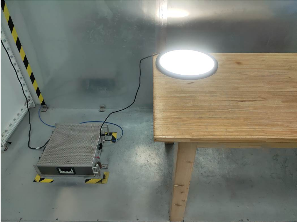
Photos of Conducted Emission Measurement
