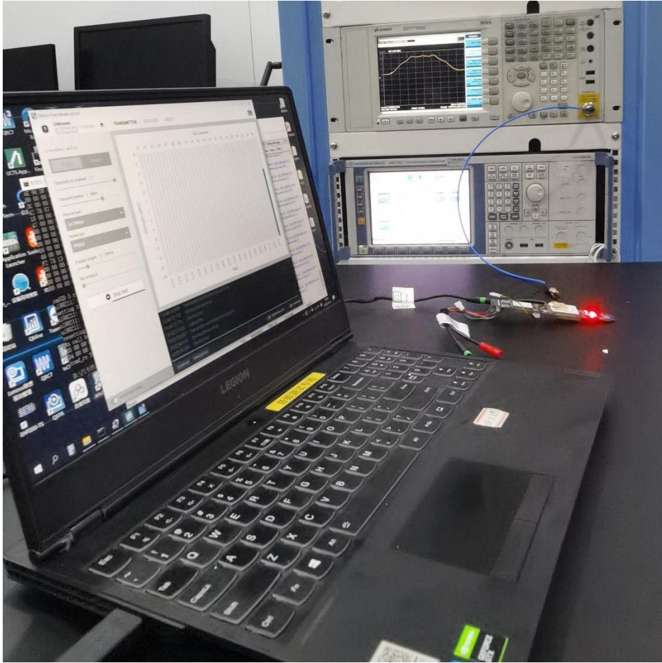
RF Conducted Test Setup
