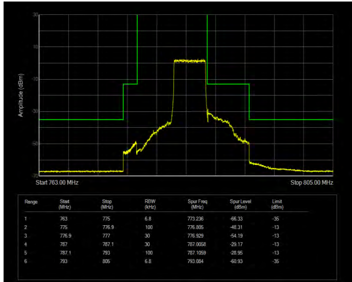
Band14 16QAM BW=10MHz Channel=23330 RB Size=50 Position=#0
