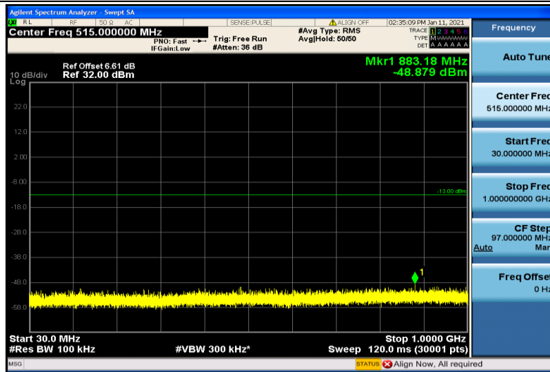
Band25-20MHz-16QAM-26590-1RB#0-30~1000MHz
