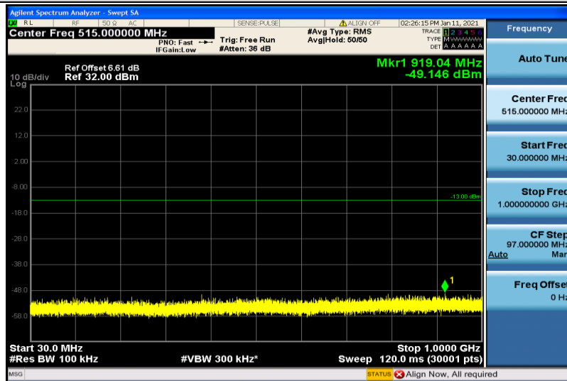
Band25-15MHz-QPSK-26365-1RB#0-30~1000MHz
