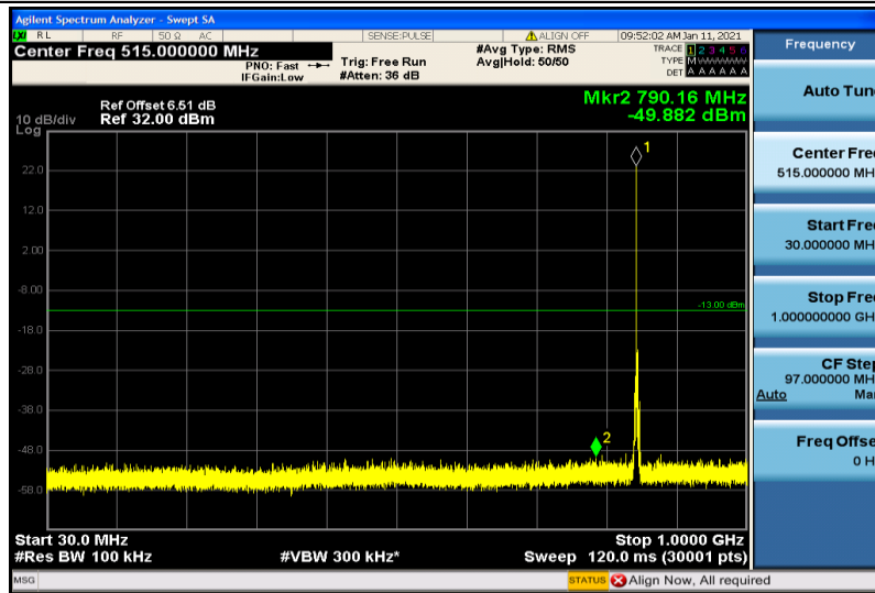
Band26-3MHz-16QAM-27025-1RB#0-30~1000MHz
