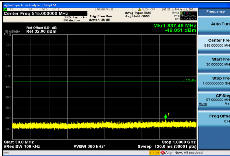
Band25-10MHz-16QAM-26640-1RB#0-30~1000MHz
