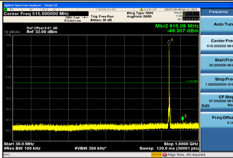
Band26-5MHz-16QAM-27015-1RB#0-30~1000MHz
