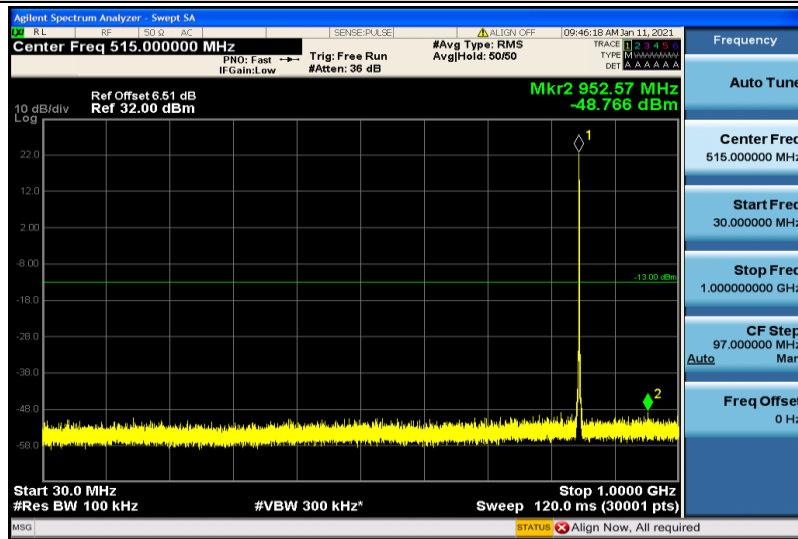
Band26-1.4MHz-QPSK-27033-1RB#0-30~1000MHz
