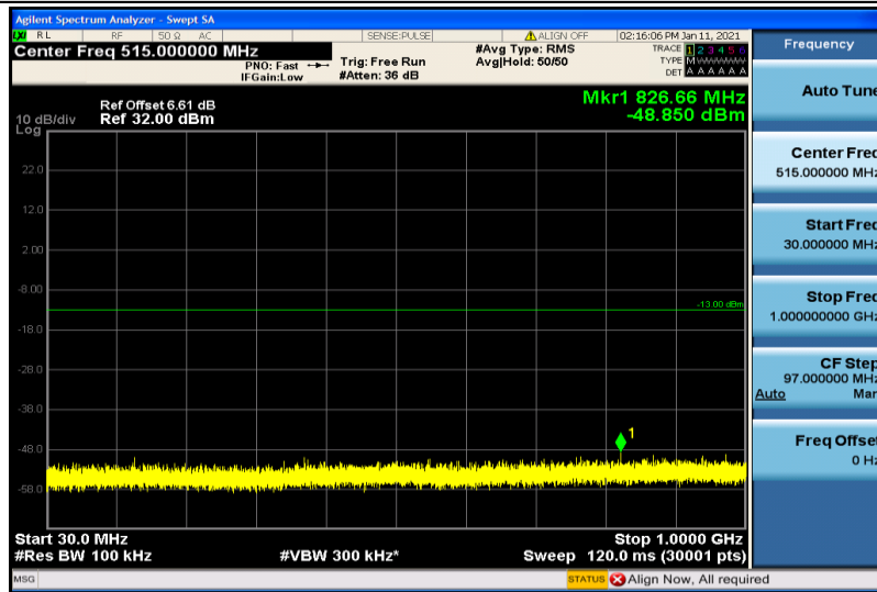
Band25-5MHz-16QAM-26665-1RB#0-30~1000MHz
