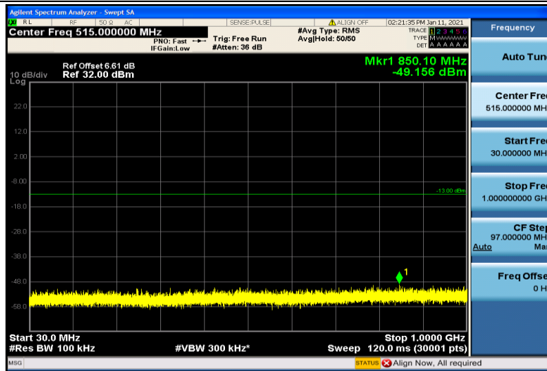
Band25-10MHz-QPSK-26640-1RB#0-30~1000MHz
