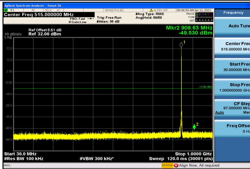
Band26-1.4MHz-16QAM-27033-1RB#0-30~1000MHz
