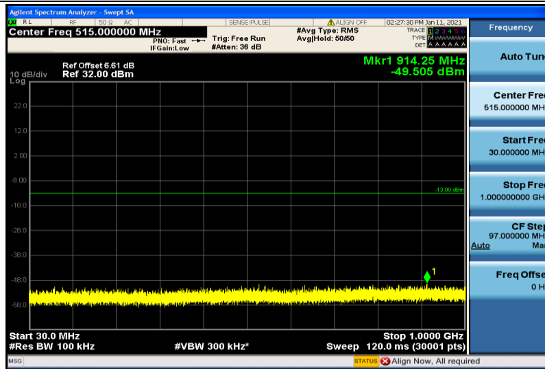
Band25-15MHz-QPSK-26615-1RB#0-30~1000MHz
