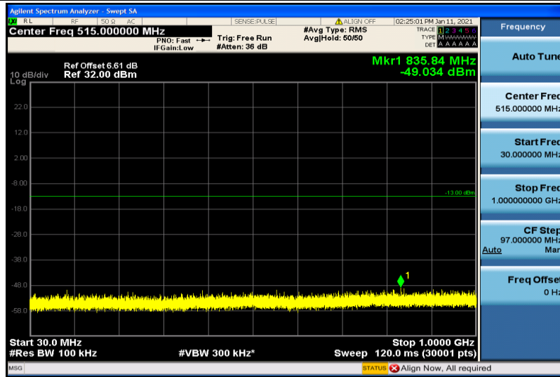
Band25-15MHz-QPSK-26115-1RB#0-30~1000MHz
