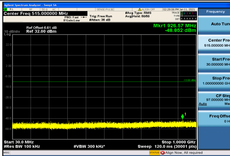
Band25-15MHz-16QAM-26615-1RB#0-30~1000MHz
