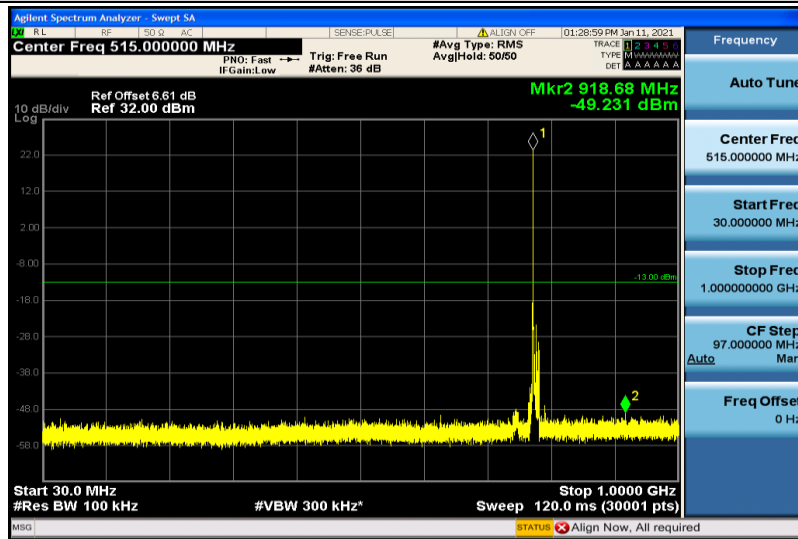
Band13-10MHz-16QAM-23230-1RB#0-30~1000MHz
