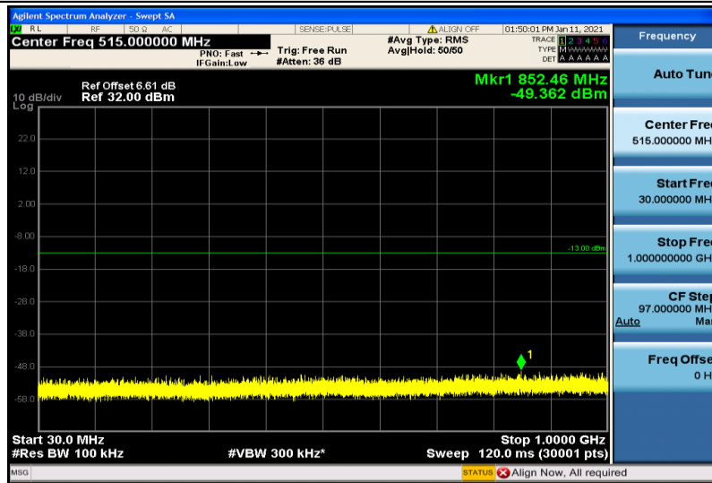
Band25-1.4MHz-16QAM-26683-1RB#0-30~1000MHz
