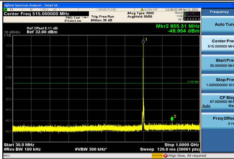
Band12-3MHz-QPSK-23095-1RB#0-30~1000MHz
