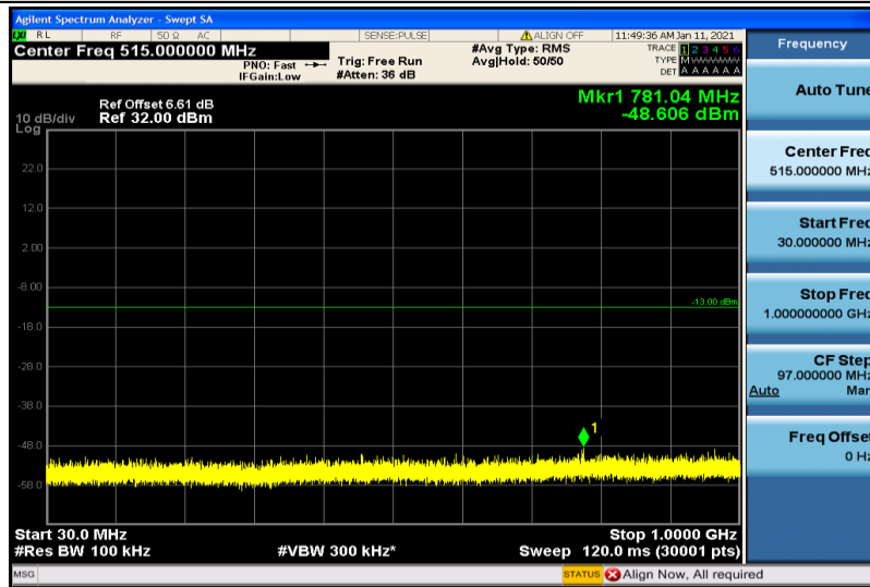
Band2-10MHz-QPSK-18900-1RB#0-30~1000MHz
