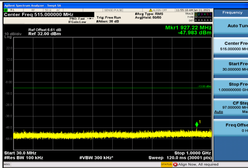
Band2-15MHz-16QAM-18900-1RB#0-30~1000MHz
