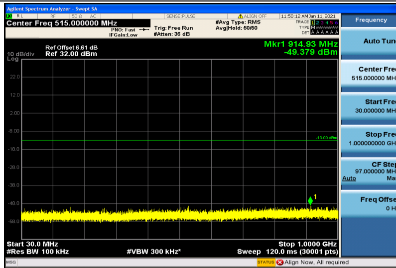
Band2-10MHz-16QAM-18900-1RB#0-30~1000MHz
