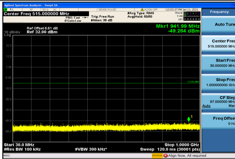
Band4-1.4MHz-QPSK-20175-1RB#0-30~1000MHz
