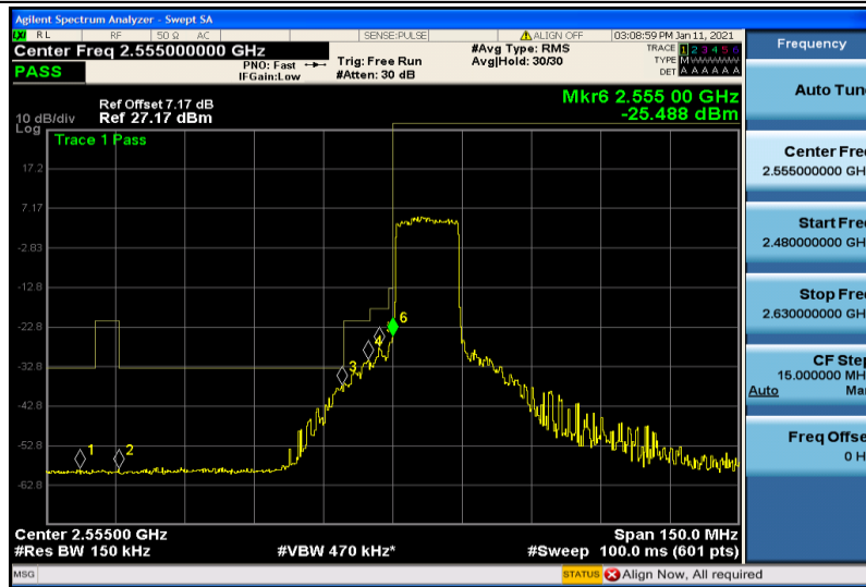
Band41-15MHz-QPSK-40315-75RB#0
