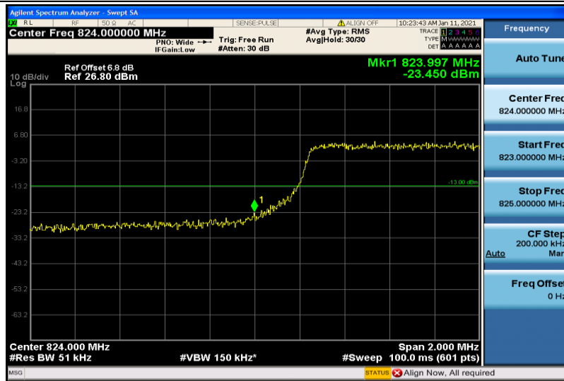
Band26-5MHz-16QAM-26815-25RB#0
