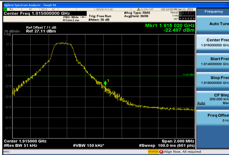
Band25-5MHz-QPSK-26665-1RB#24
