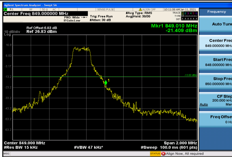
Band26-1.4MHz-16QAM-27033-1RB#5
