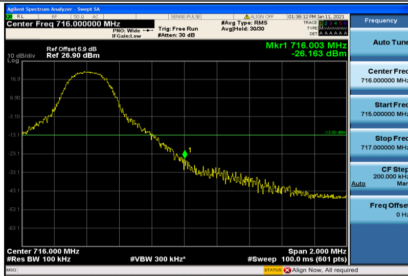
Band17-10MHz-QPSK-23800-1RB#49
