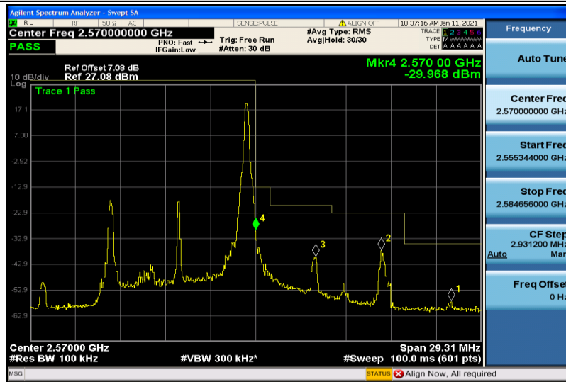
Band7-10MHz-16QAM-21400-1RB#49
