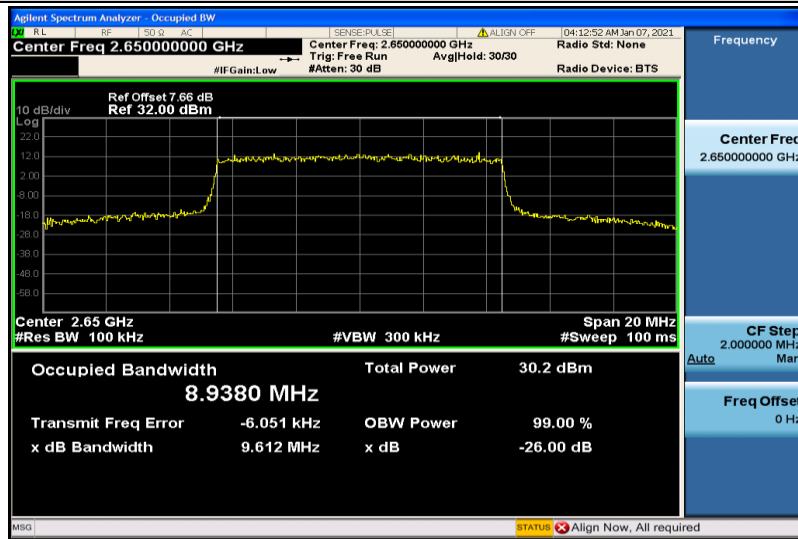
Band41-10MHz-16QAM-41190-50RB#0-8.9380
