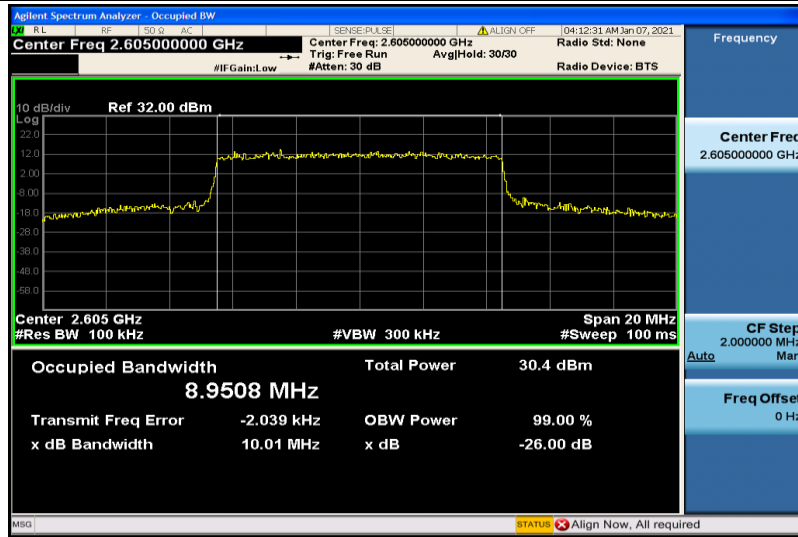
Band41-10MHz-16QAM-40740-50RB#0-8.9508
