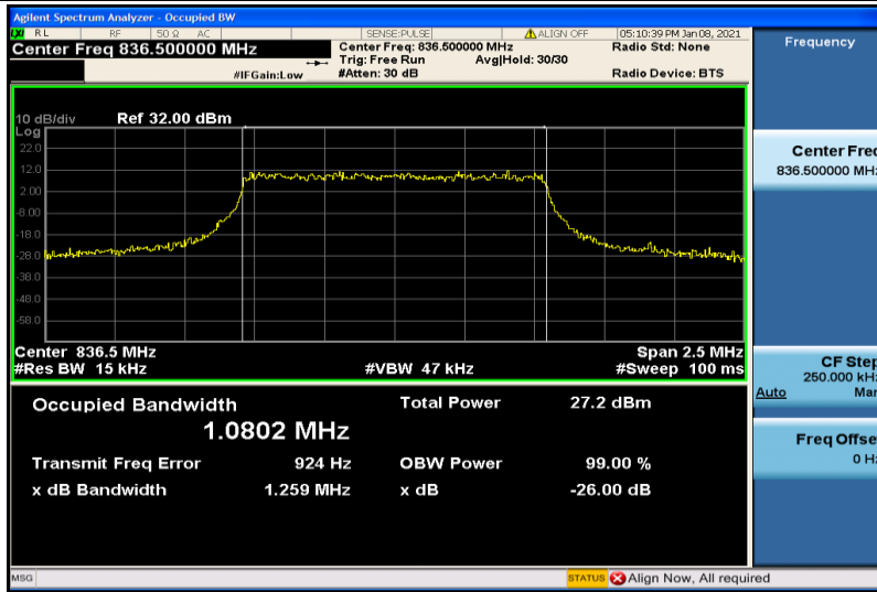
Band26-1.4MHz-16QAM-26915-6RB#0-1.0802
