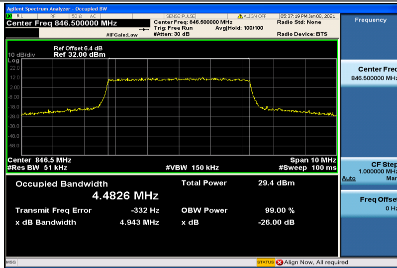
Band26-5MHz-QPSK-27015-25RB#0-4.4826
