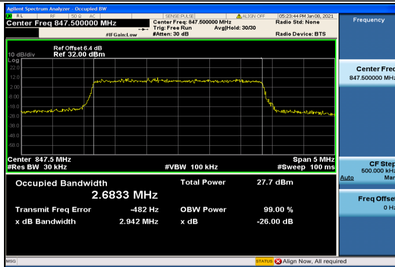
Band26-3MHz-16QAM-27025-15RB#0-2.6833
