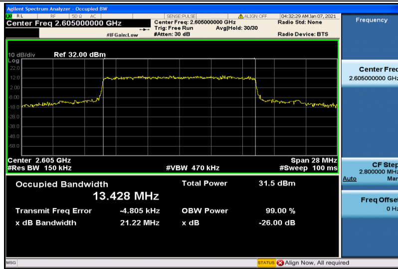
Band41-15MHz-QPSK-40740-75RB#0-13.428
