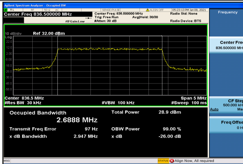
Band26-3MHz-QPSK-26915-15RB#0-2.6888
