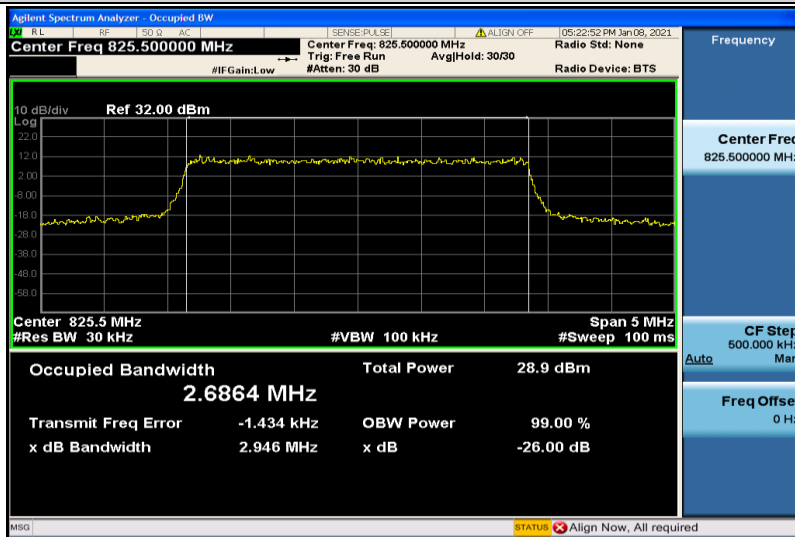
Band26-3MHz-QPSK-26805-15RB#0-2.6864
