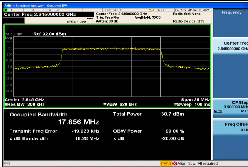
Band41-20MHz-16QAM-41140-100RB#0-17.856
