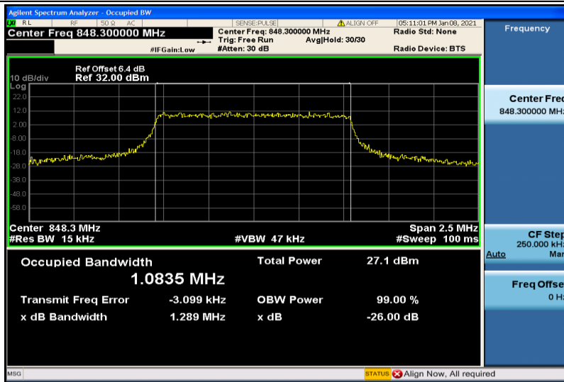
Band26-1.4MHz-16QAM-27033-6RB#0-1.0835
