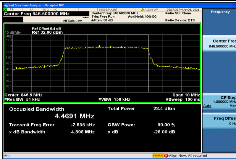
Band26-5MHz-16QAM-27015-25RB#0-4.4691
