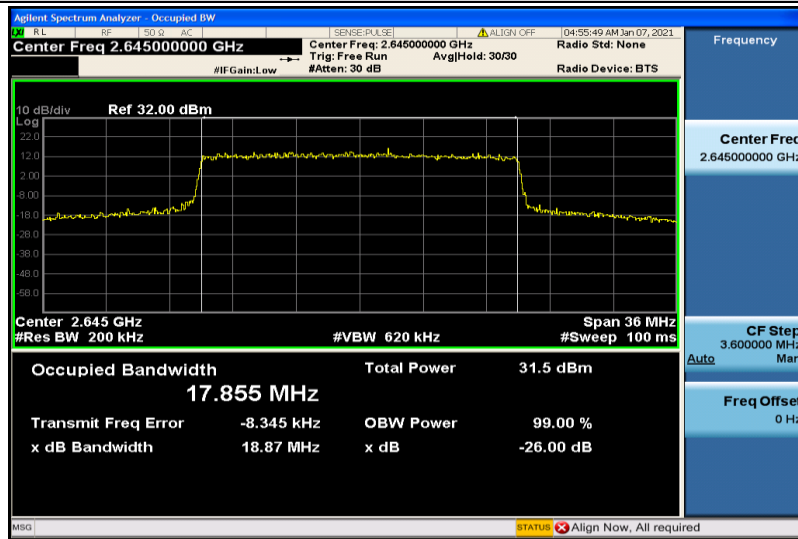
Band41-20MHz-QPSK-41140-100RB#0-17.855
