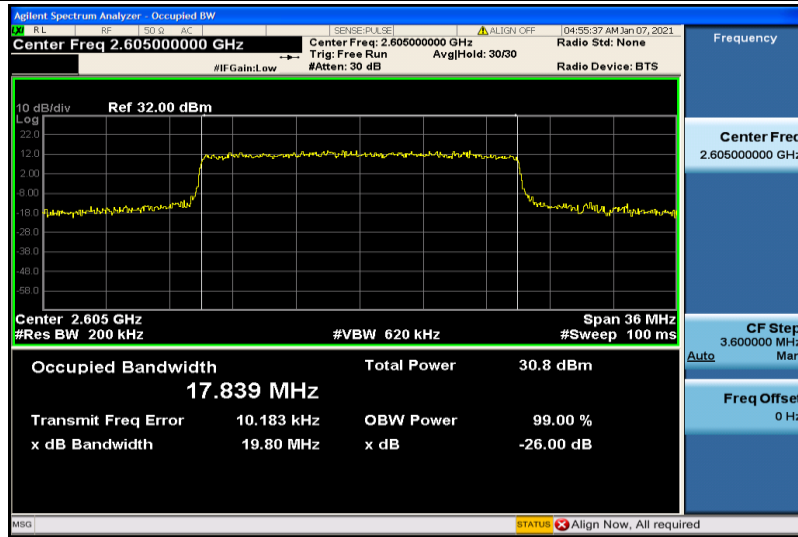
Band41-20MHz-16QAM-40740-100RB#0-17.839
