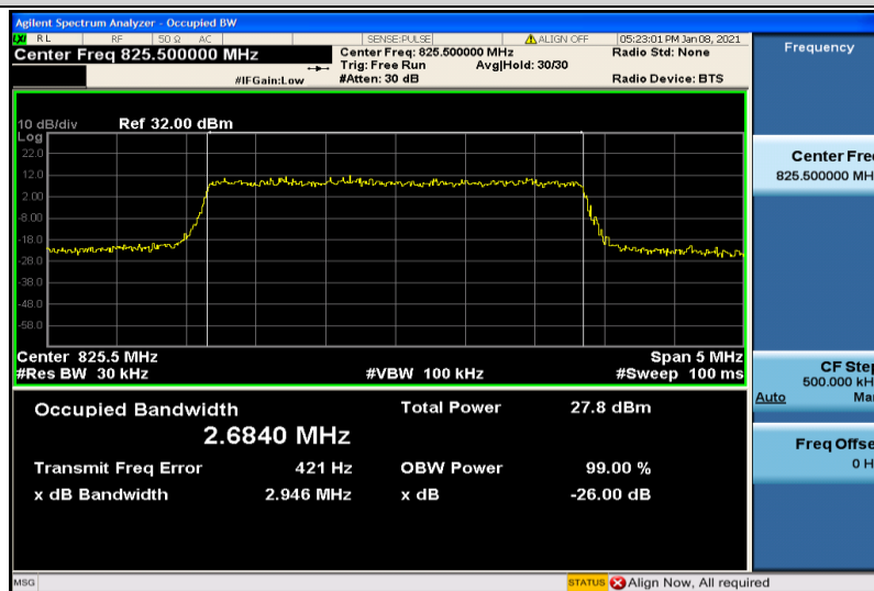
Band26-3MHz-16QAM-26805-15RB#0-2.6840
