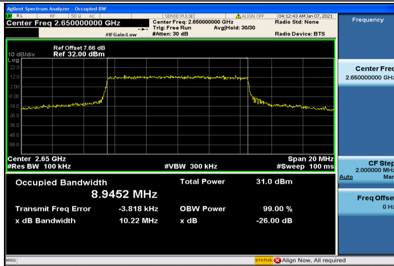
Band41-10MHz-QPSK-41190-50RB#0-8.9452
