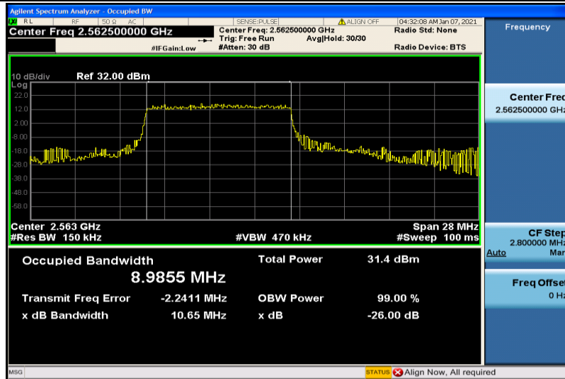
Band41-15MHz-QPSK-40315-75RB#0-8.9855
