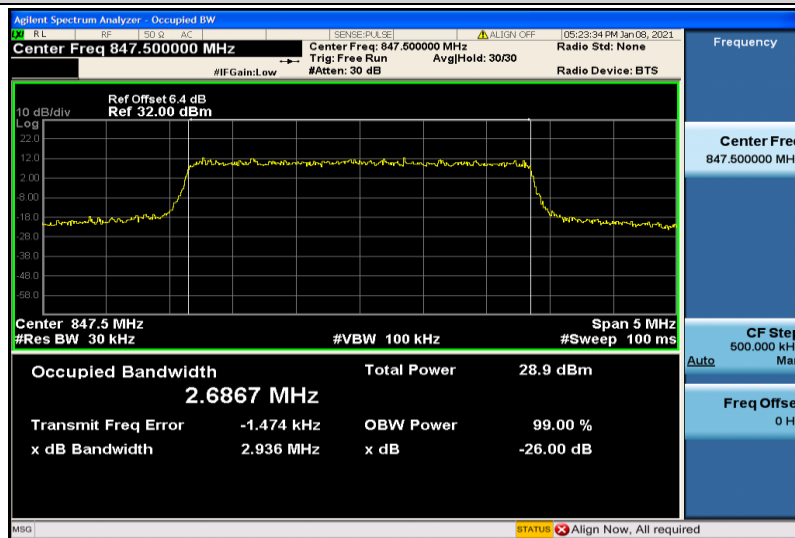
Band26-3MHz-QPSK-27025-15RB#0-2.6867
