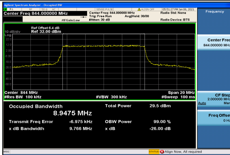
Band26-10MHz-QPSK-26990-50RB#0-8.9475
