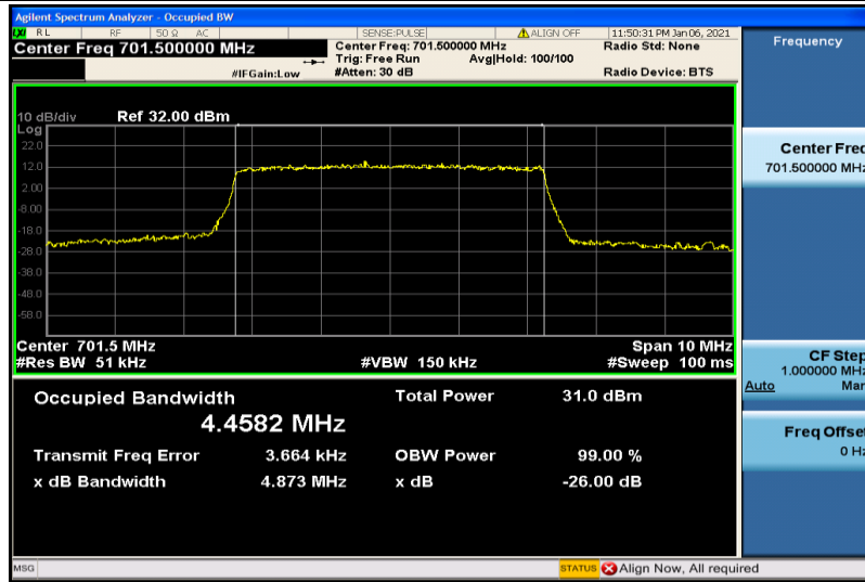
Band12-5MHz-QPSK-23035-25RB#0-4.4582
