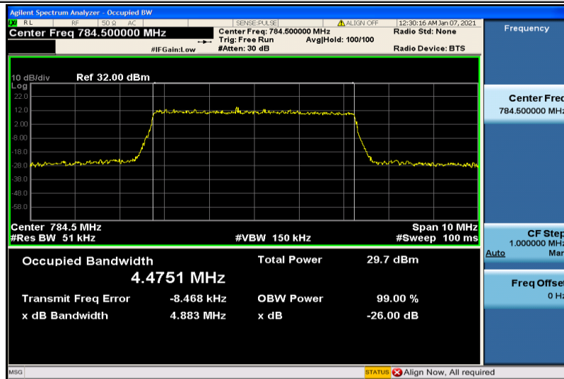
Band13-5MHz-16QAM-23255-25RB#0-4.4751
