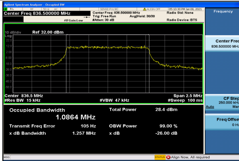
Band26-1.4MHz-QPSK-26915-6RB#0-1.0864
