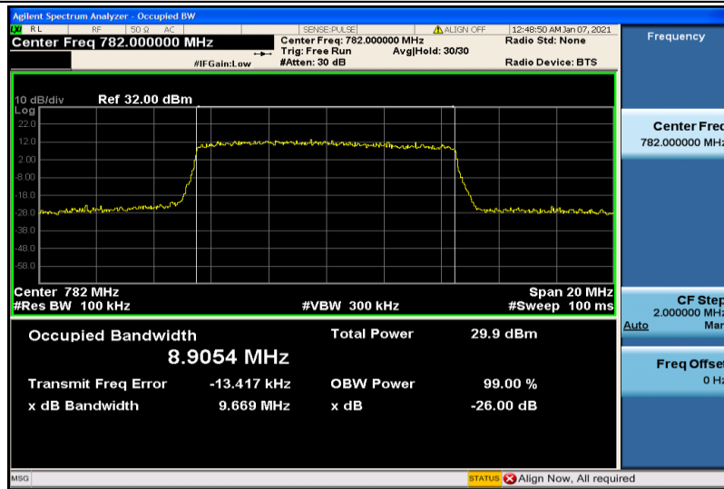
Band13-10MHz-16QAM-23230-50RB#0-8.9054
