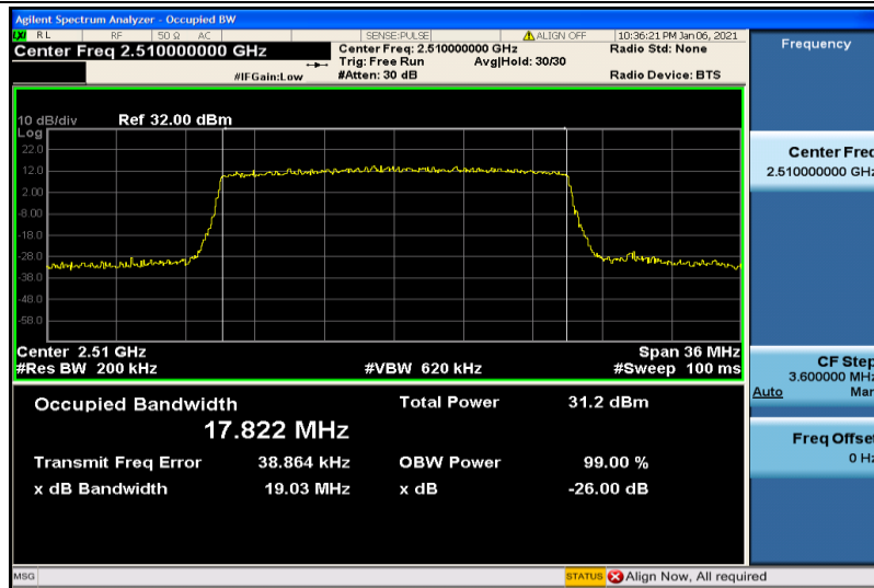
Band7-20MHz-16QAM-20850-100RB#0-17.822
