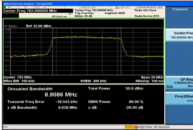
Band13-10MHz-QPSK-23230-50RB#0-8.9086
