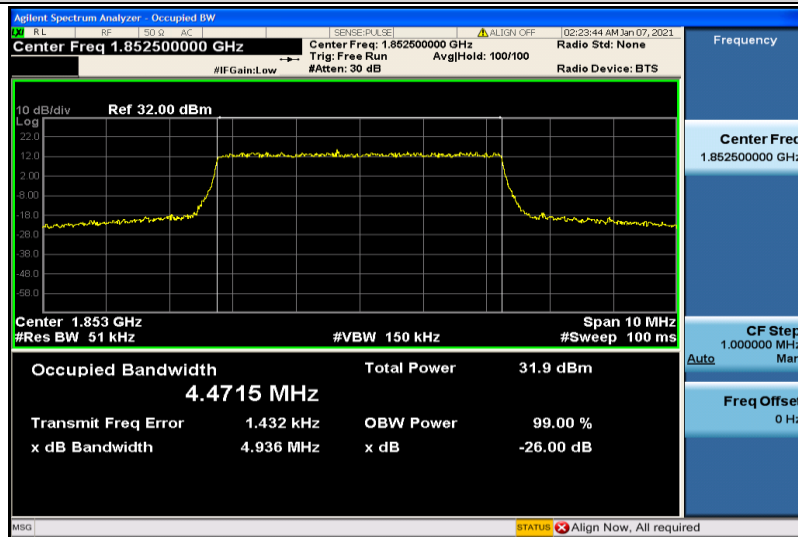
Band25-5MHz-QPSK-26065-25RB#0-4.4715
