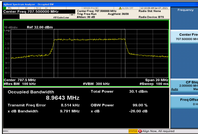
Band12-10MHz-16QAM-23095-50RB#0-8.9643
