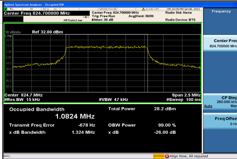
Band26-1.4MHz-QPSK-26797-6RB#0-1.0824
