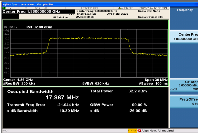
Band25-20MHz-QPSK-26140-100RB#0-17.867
