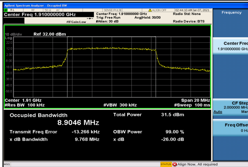
Band25-10MHz-QPSK-26640-50RB#0-8.9046
