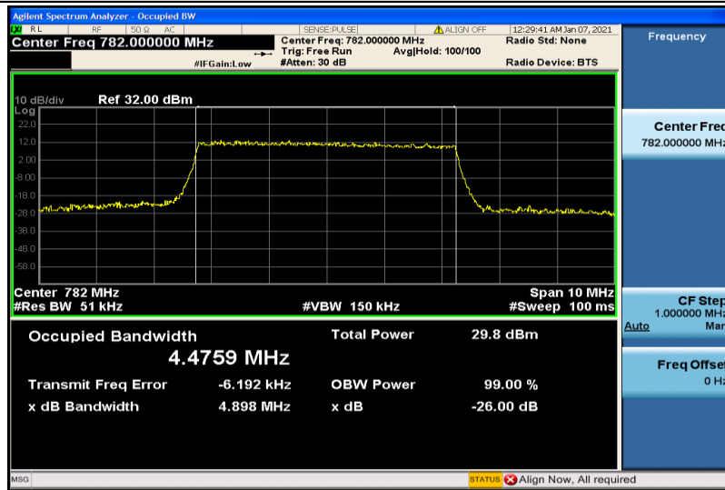
Band13-5MHz-16QAM-23230-25RB#0-4.4759
