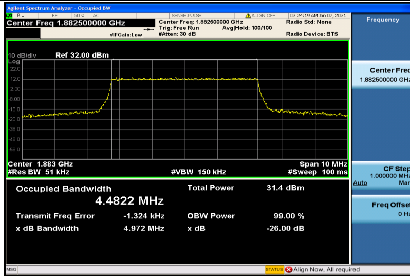
Band25-5MHz-QPSK-26365-25RB#0-4.4822
