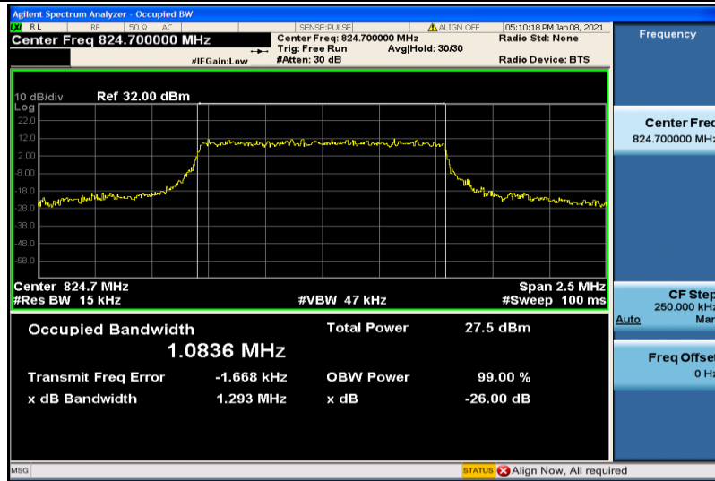
Band26-1.4MHz-16QAM-26797-6RB#0-1.0836
