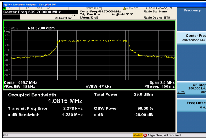
Band12-1.4MHz-16QAM-23017-6RB#0-1.0815
