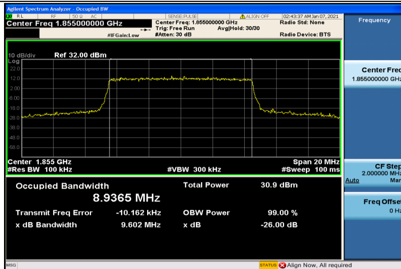
Band25-10MHz-16QAM-26090-50RB#0-8.9365
