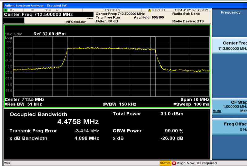
Band12-5MHz-QPSK-23155-25RB#0-4.4758
