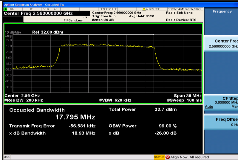
Band7-20MHz-QPSK-21350-100RB#0-17.795
