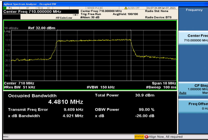
Band17-5MHz-QPSK-23790-25RB#0-4.4810
