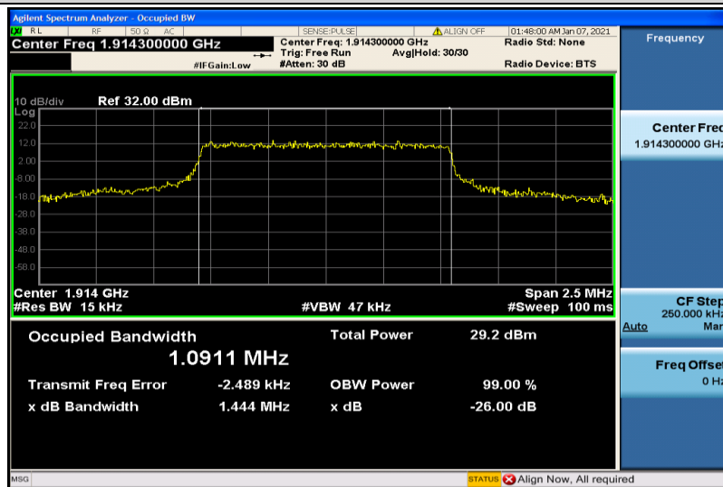
Band25-1.4MHz-16QAM-26683-6RB#0-1.0911
