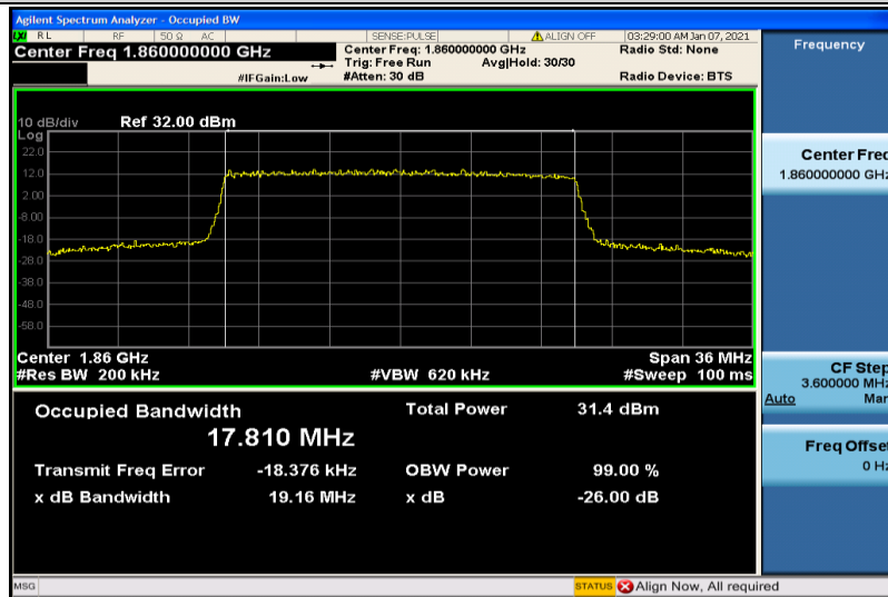
Band25-20MHz-16QAM-26140-100RB#0-17.810
