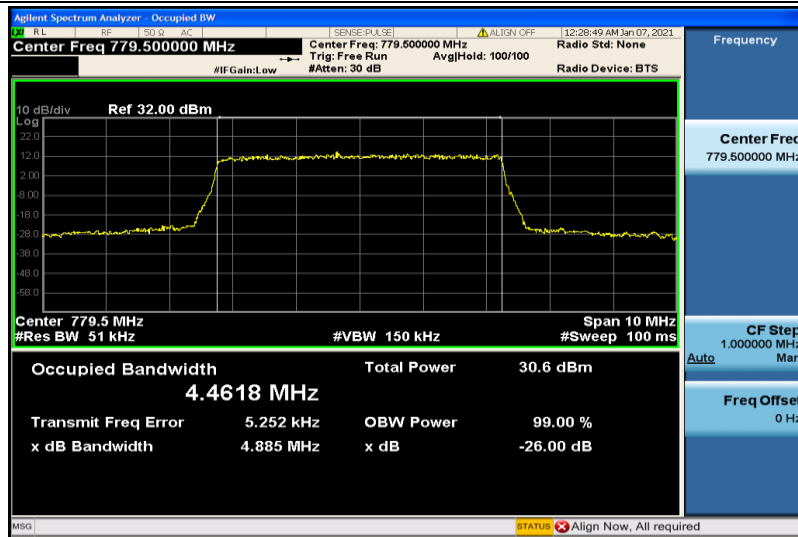
Band13-5MHz-QPSK-23205-25RB#0-4.4618
