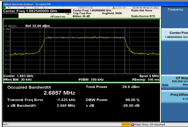
Band25-3MHz-16QAM-26365-15RB#0-2.6857
