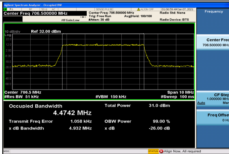
Band17-5MHz-QPSK-23755-25RB#0-4.4742
