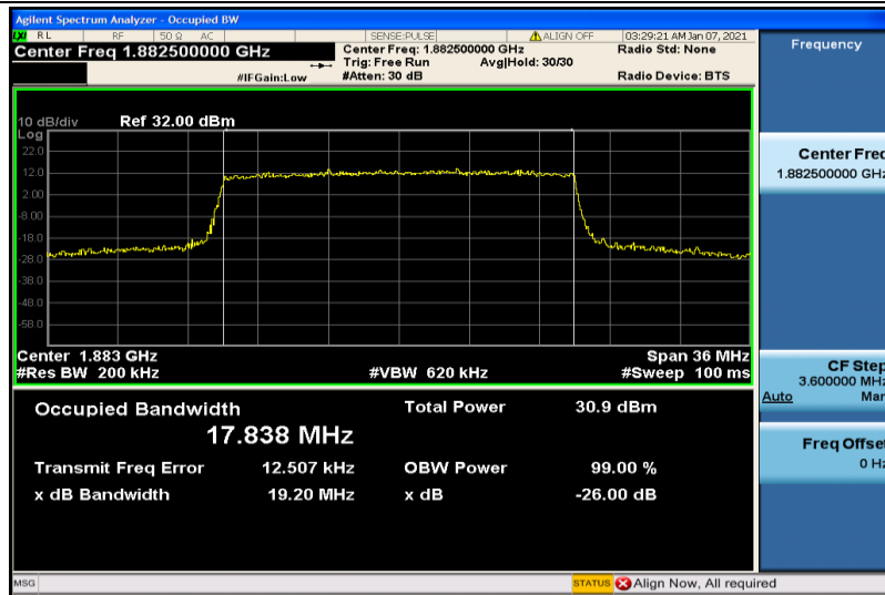
Band25-20MHz-16QAM-26365-100RB#0-17.838
