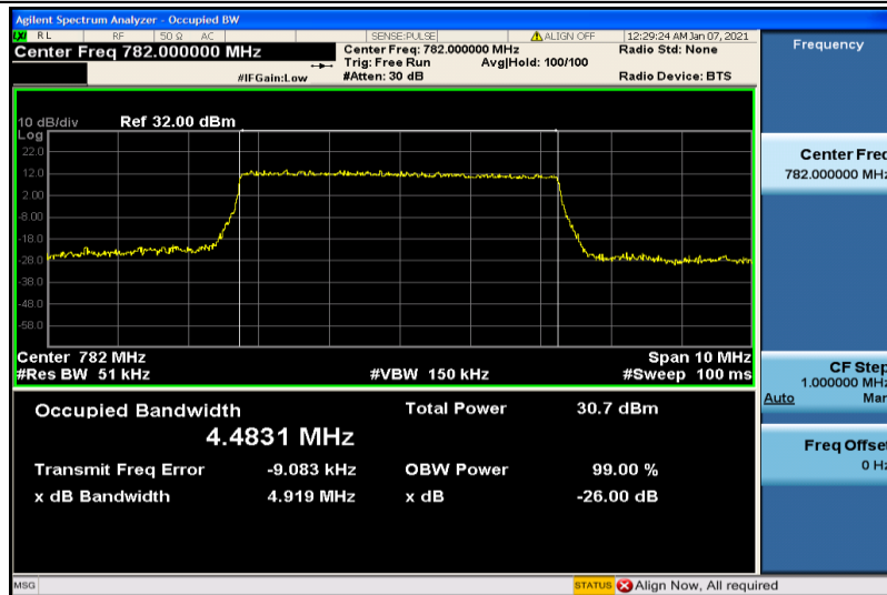
Band13-5MHz-QPSK-23230-25RB#0-4.4831
