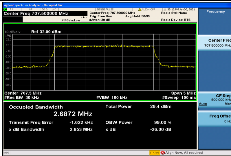
Band12-3MHz-16QAM-23095-15RB#0-2.6872
