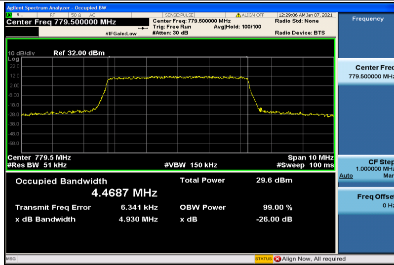
Band13-5MHz-16QAM-23205-25RB#0-4.4687
