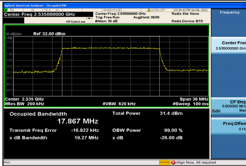
Band7-20MHz-16QAM-21100-100RB#0-17.867
