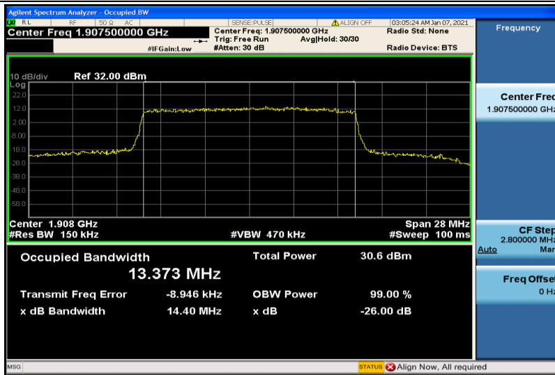
Band25-15MHz-16QAM-26615-75RB#0-13.373
