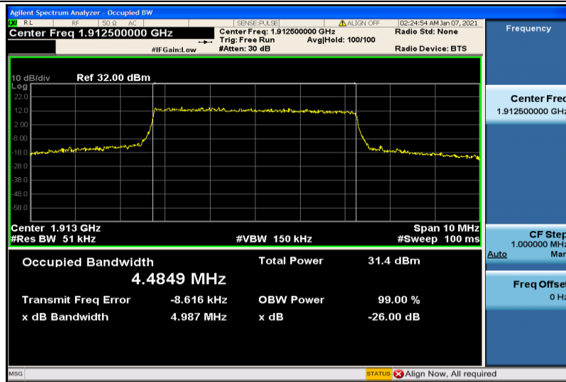
Band25-5MHz-QPSK-26665-25RB#0-4.4849
