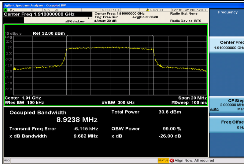
Band25-10MHz-16QAM-26640-50RB#0-8.9238
