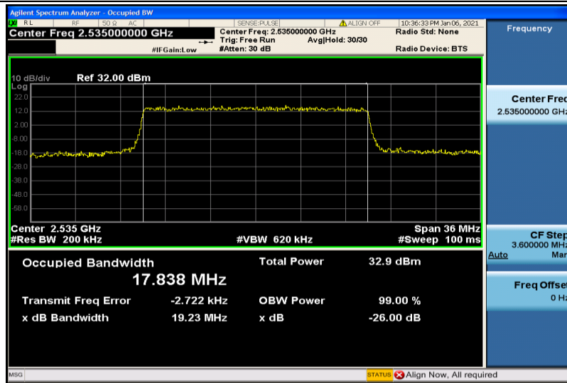
Band7-20MHz-QPSK-21100-100RB#0-17.838
