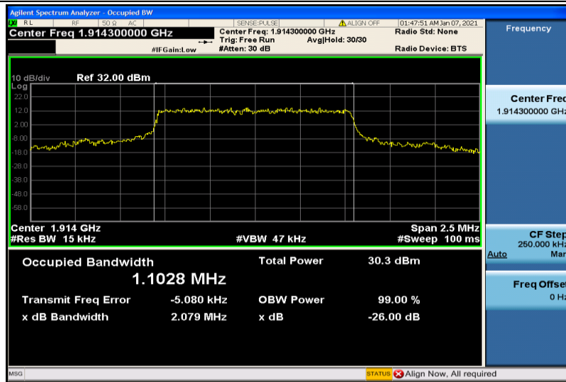
Band25-1.4MHz-QPSK-26683-6RB#0-1.1028
