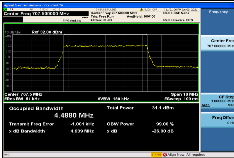
Band12-5MHz-QPSK-23095-25RB#0-4.4880
