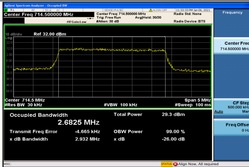
Band12-3MHz-16QAM-23165-15RB#0-2.6825
