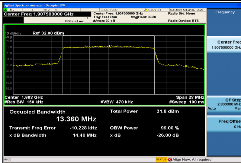
Band25-15MHz-QPSK-26615-75RB#0-13.360
