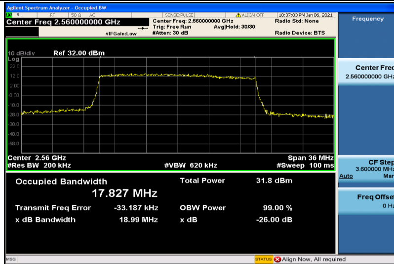
Band7-20MHz-16QAM-21350-100RB#0-17.827
