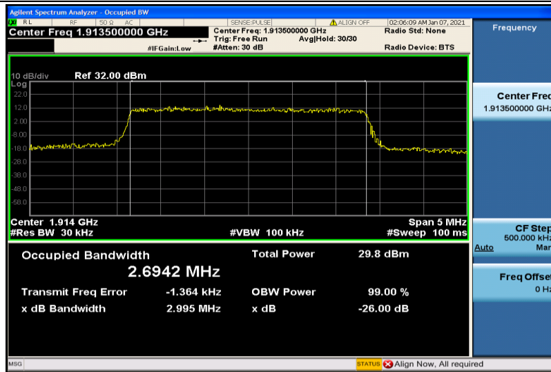
Band25-3MHz-16QAM-26675-15RB#0-2.6942
