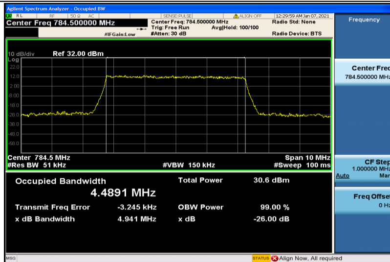
Band13-5MHz-QPSK-23255-25RB#0-4.4891
