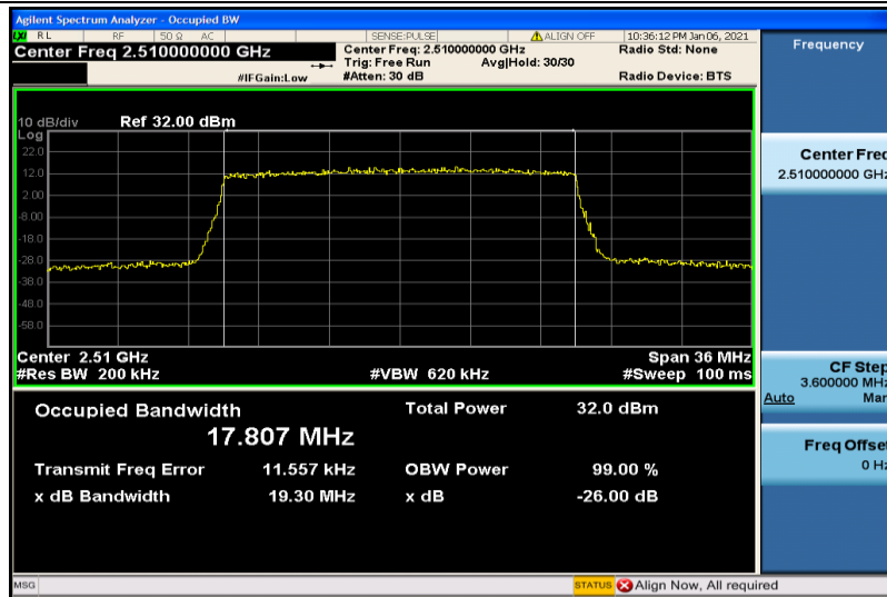
Band7-20MHz-QPSK-20850-100RB#0-17.807
