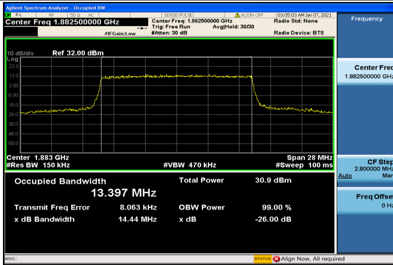
Band25-15MHz-16QAM-26365-75RB#0-13.397
