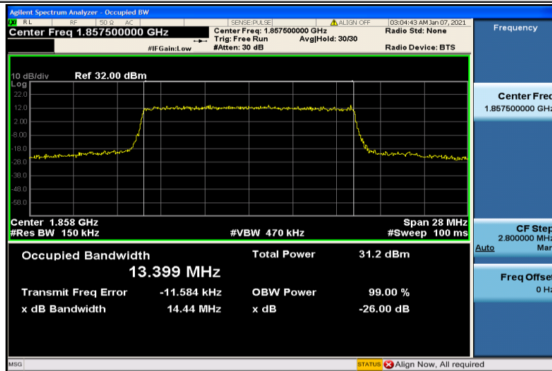
Band25-15MHz-16QAM-26115-75RB#0-13.399
