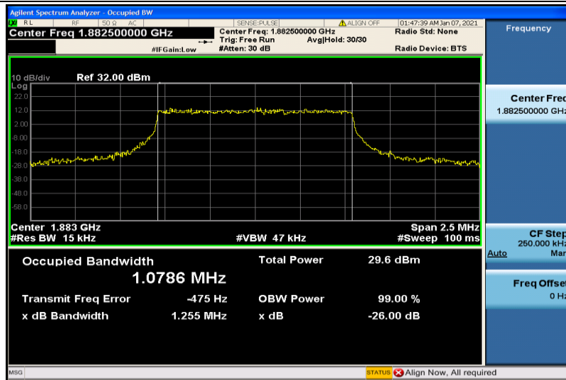
Band25-1.4MHz-16QAM-26365-6RB#0-1.0786
