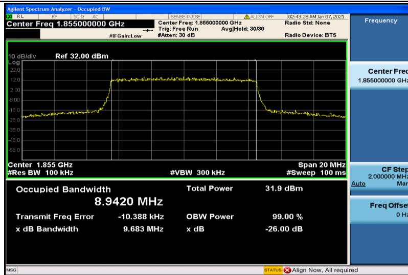
Band25-10MHz-QPSK-26090-50RB#0-8.9420
