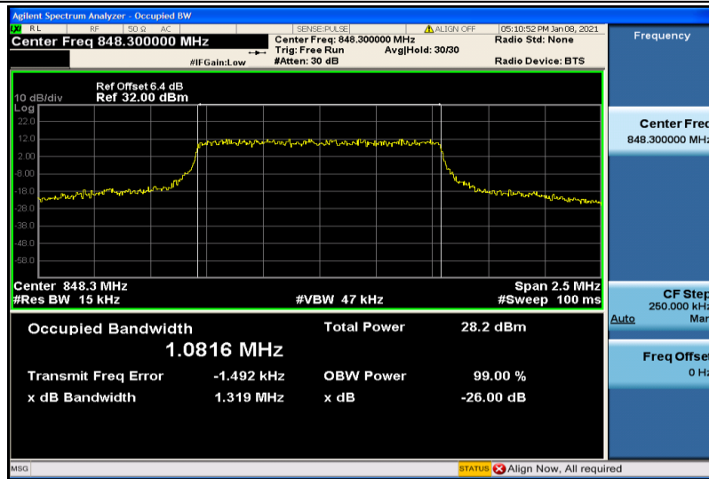
Band26-1.4MHz-QPSK-27033-6RB#0-1.0816
