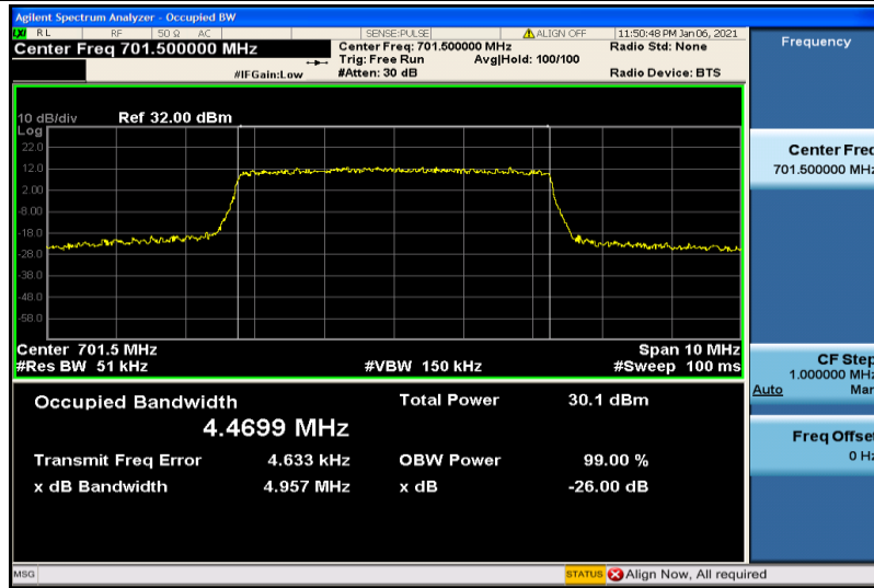
Band12-5MHz-16QAM-23035-25RB#0-4.4699
