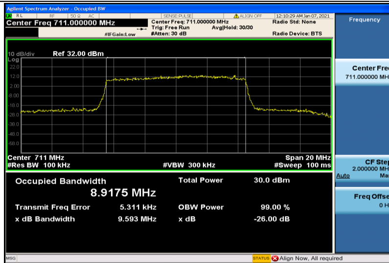
Band12-10MHz-16QAM-23130-50RB#0-8.9175
