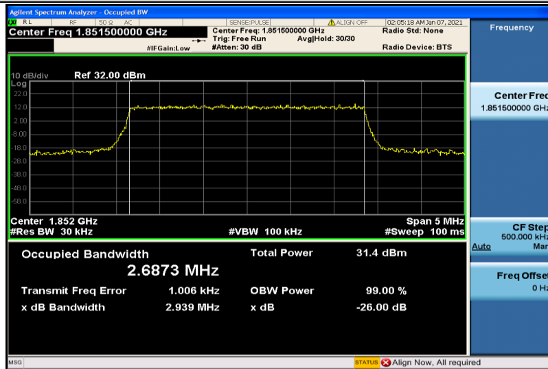
Band25-3MHz-QPSK-26055-15RB#0-2.6873
