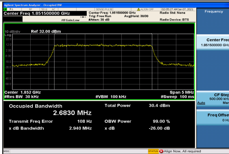
Band25-3MHz-16QAM-26055-15RB#0-2.6830
