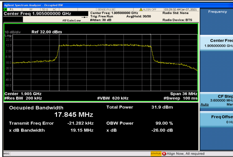
Band25-20MHz-QPSK-26590-100RB#0-17.845
