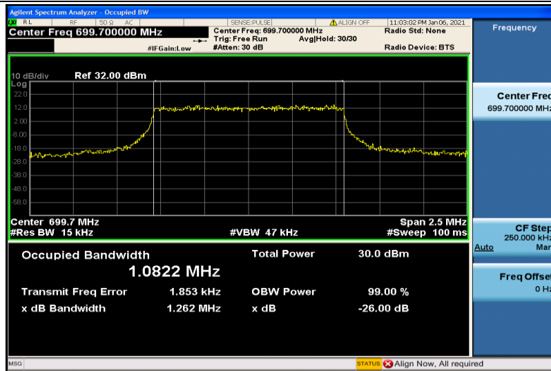
Band12-1.4MHz-QPSK-23017-6RB#0-1.0822
