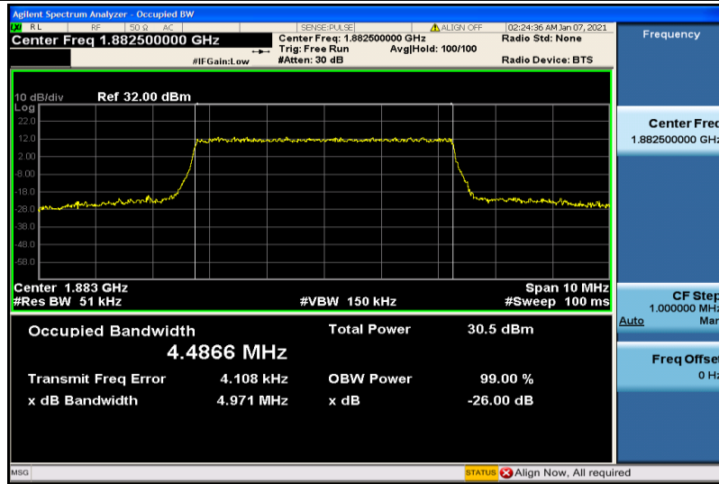
Band25-5MHz-16QAM-26365-25RB#0-4.4866
