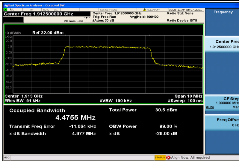
Band25-5MHz-16QAM-26665-25RB#0-4.4755
