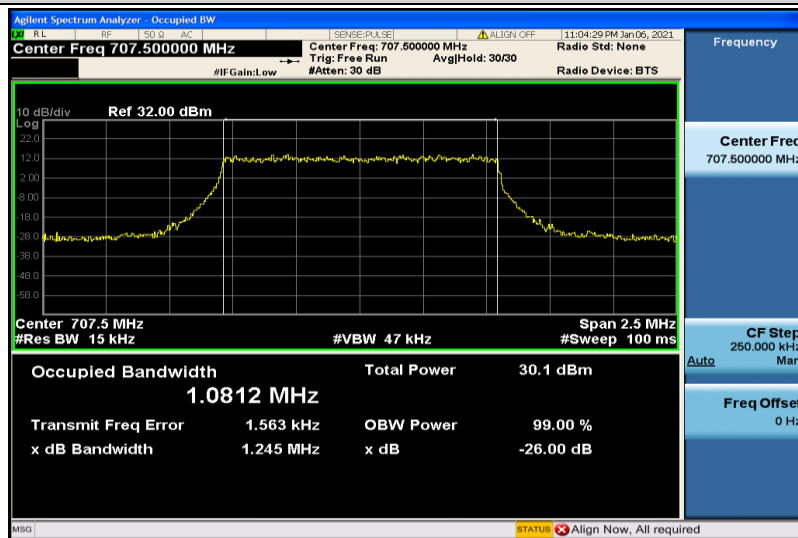
Band12-1.4MHz-QPSK-23095-6RB#0-1.0812
