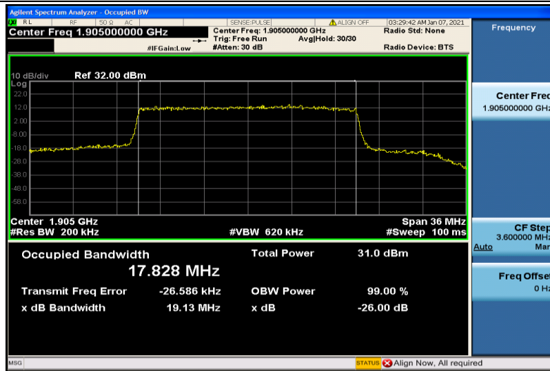
Band25-20MHz-16QAM-26590-100RB#0-17.828
