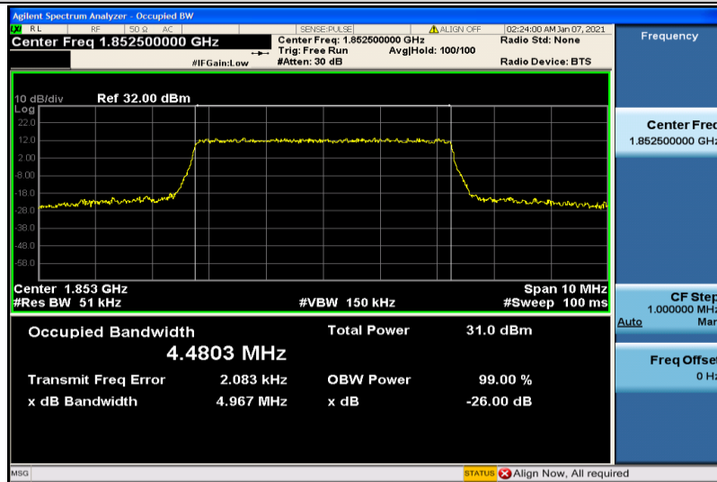
Band25-5MHz-16QAM-26065-25RB#0-4.4803
