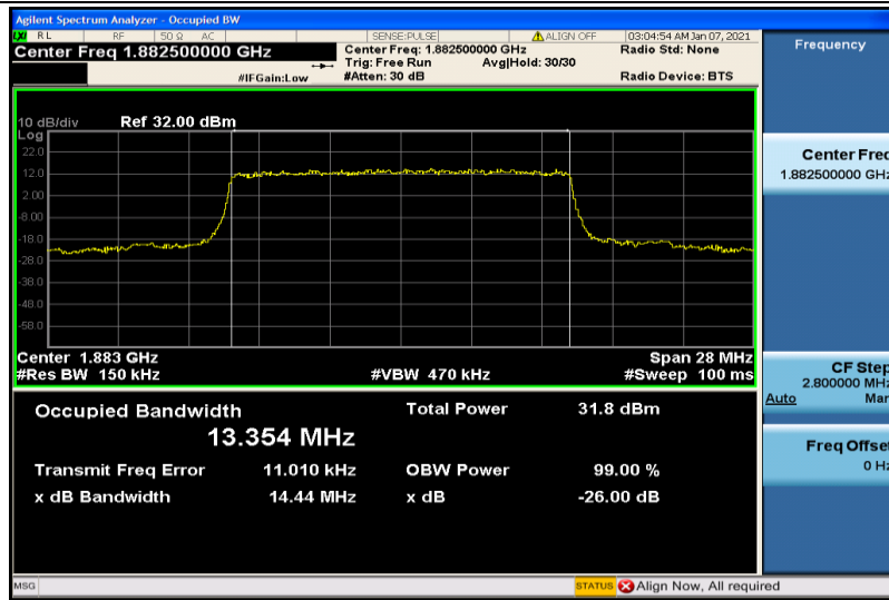
Band25-15MHz-QPSK-26365-75RB#0-13.354
