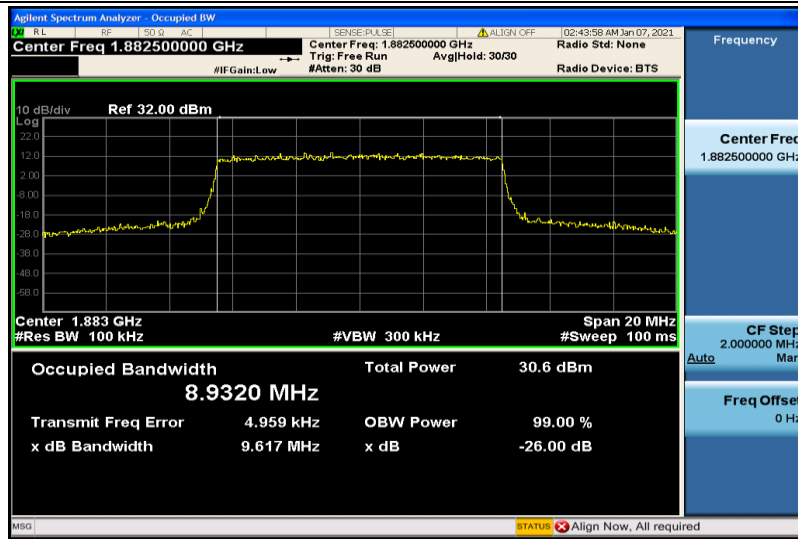
Band25-10MHz-16QAM-26365-50RB#0-8.9320
