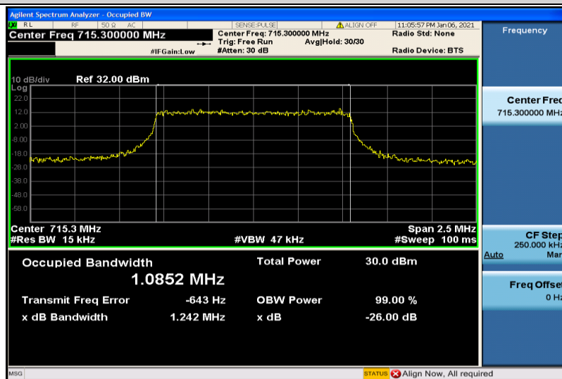
Band12-1.4MHz-QPSK-23173-6RB#0-1.0852
