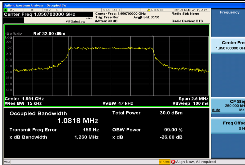
Band2-1.4MHz-16QAM-18607-6RB#0-1.0818
