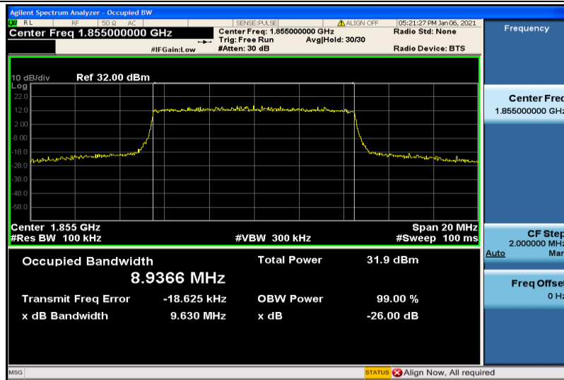
Band2-10MHz-QPSK-18650-50RB#0-8.9366
