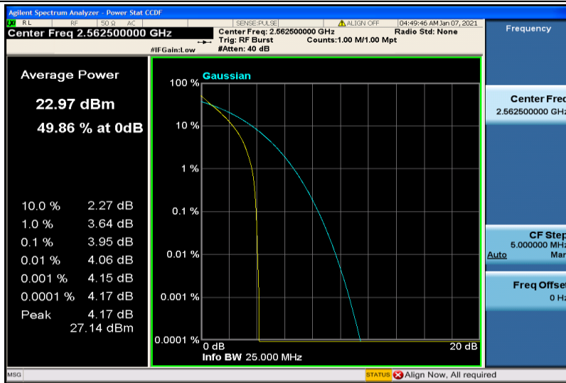
Band41-15MHz-QPSK-40315-1RB#0
