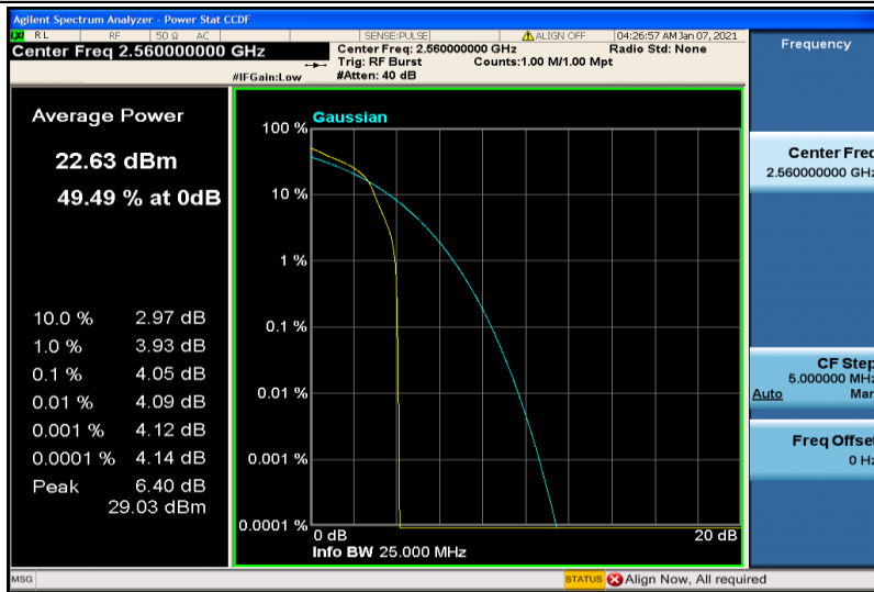
Band41-10MHz-16QAM-40290-1RB#0
