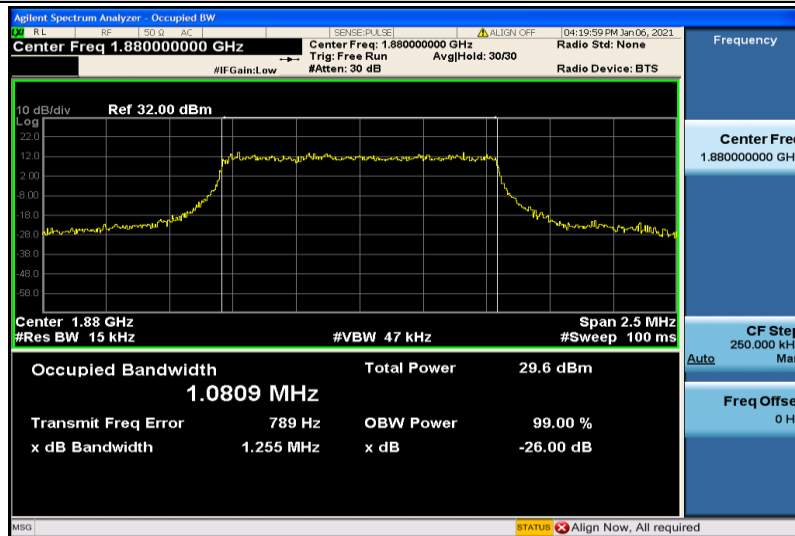
Band2-1.4MHz-16QAM-18900-6RB#0-1.0809
