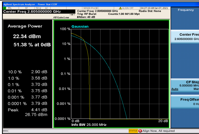
Band41-10MHz-16QAM-40740-1RB#0
