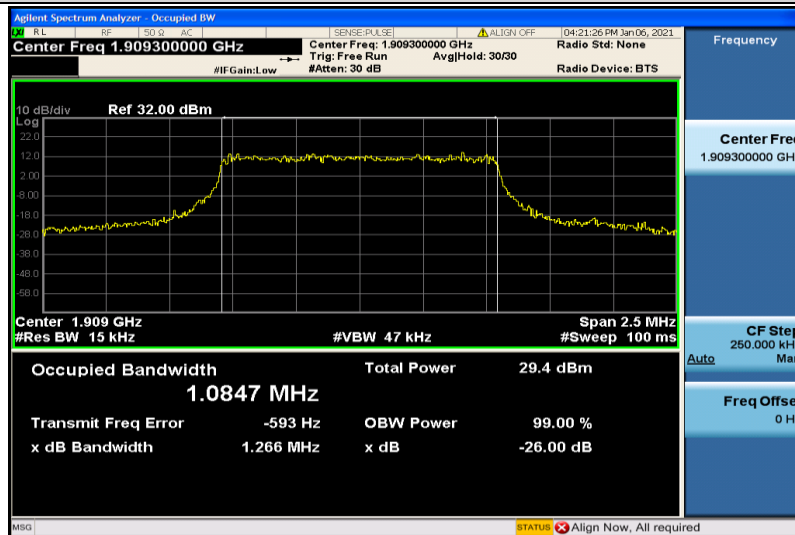
Band2-1.4MHz-16QAM-19193-6RB#0-1.0847
