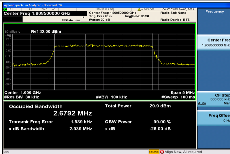
Band2-3MHz-16QAM-19185-15RB#0-2.6792
