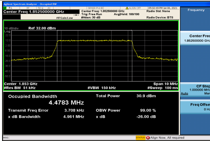
Band2-5MHz-16QAM-18625-25RB#0-4.4783
