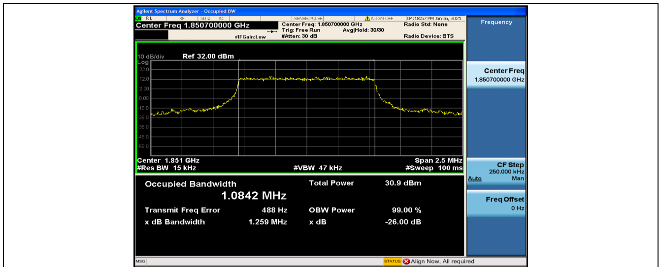
Band2-1.4MHz-QPSK-18607-6RB#0-1.0842
