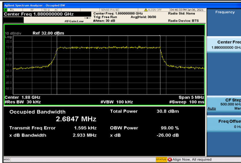
Band2-3MHz-QPSK-18900-15RB#0-2.6847
