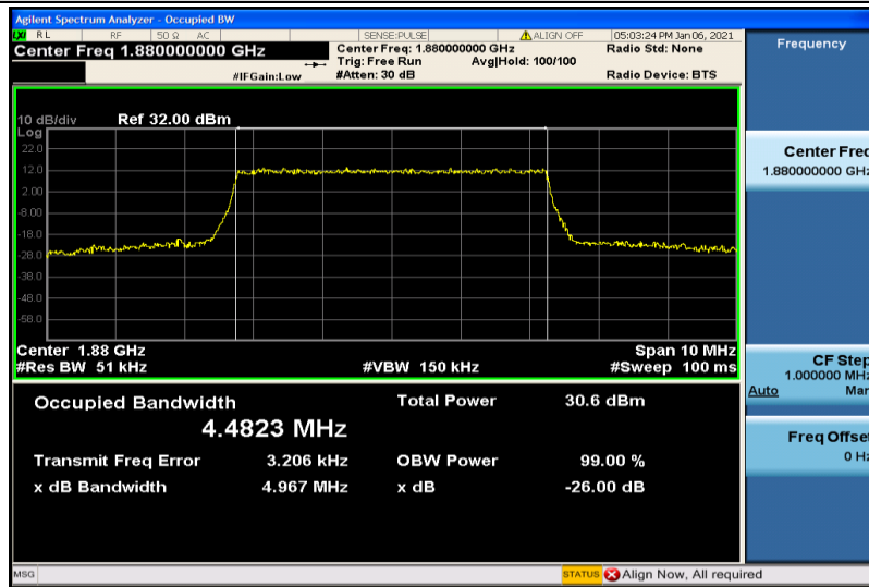
Band2-5MHz-16QAM-18900-25RB#0-4.4823
