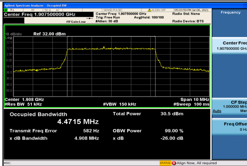
Band2-5MHz-16QAM-19175-25RB#0-4.4715
