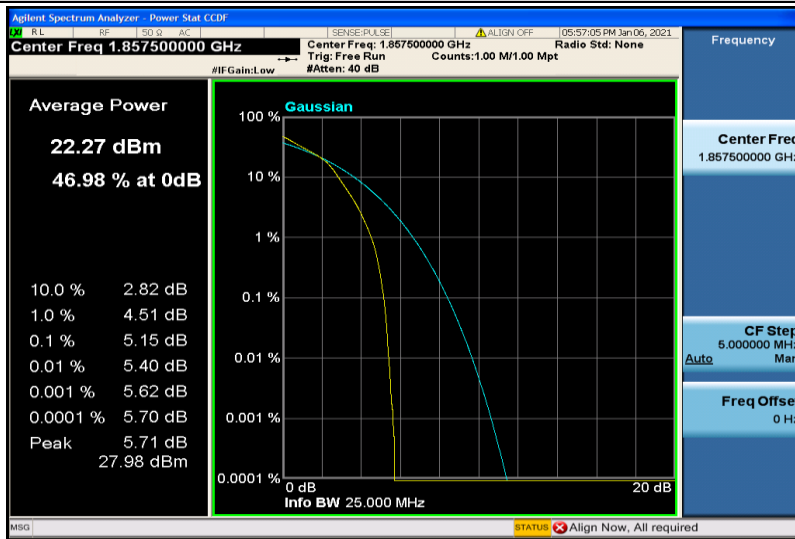
Band2-15MHz-16QAM-18675-5RB#0
