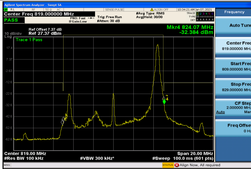
Band26-10MHz-16QAM-26740-1RB#49
