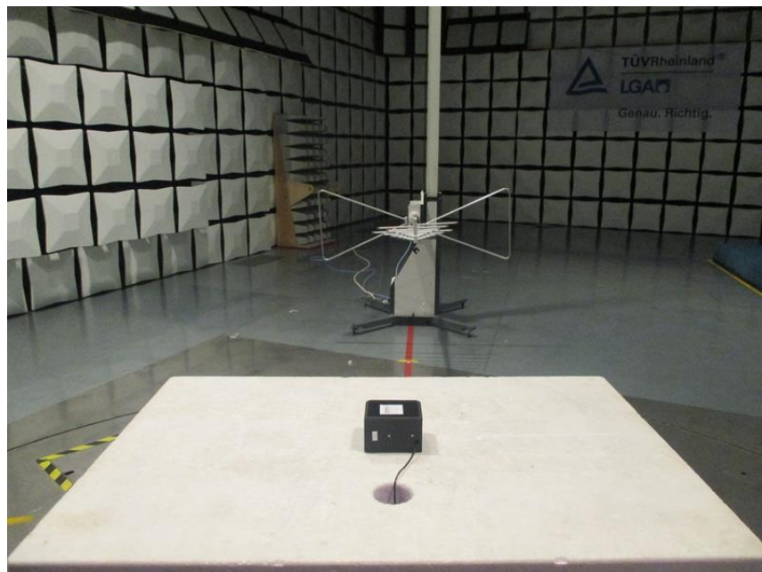
Bild / Picture 6: Test Setup: Radiated Measurements (30 MHz - 1 GHz)
