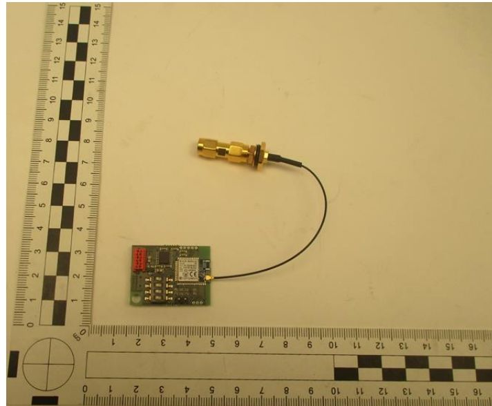
Bild / Picture 4: Conducted Secondary device
