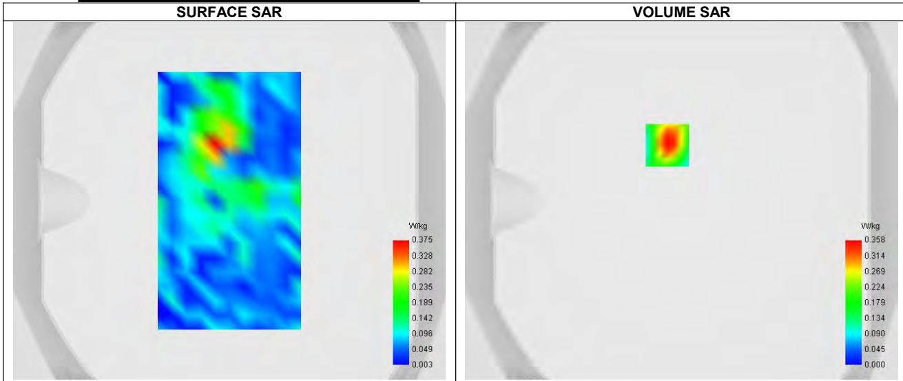
Maximum location: X=-8.00, Y=31.00 ; SAR Peak: 0.91 W/kg
