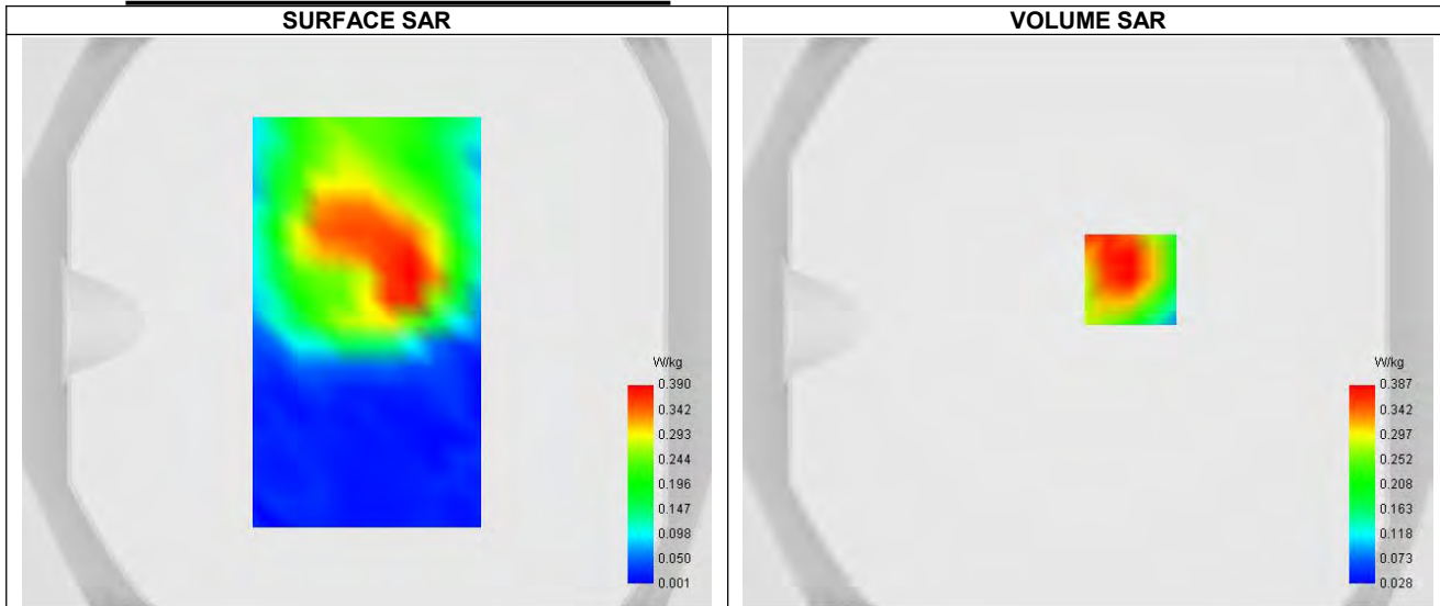
Maximum location: X=15.00, Y=15.00 ; SAR Peak: 0.59 W/kg
