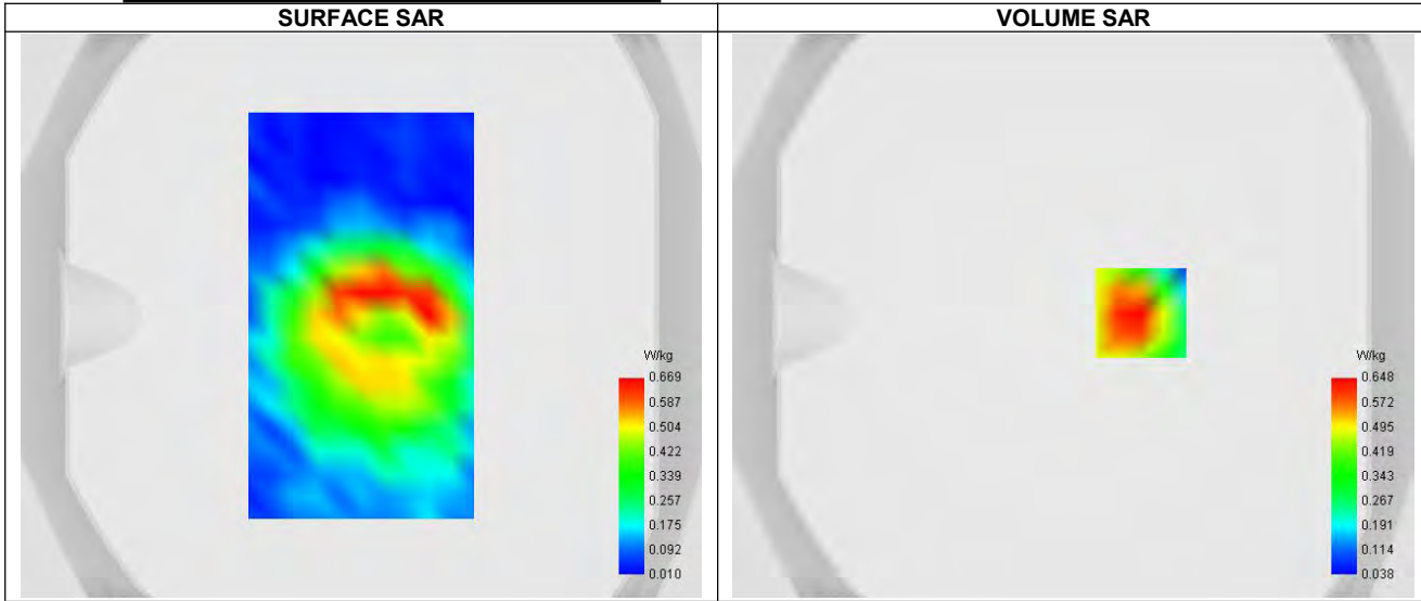
Maximum location: X=24.00, Y=1.00 ; SAR Peak: 1.14 W/kg
