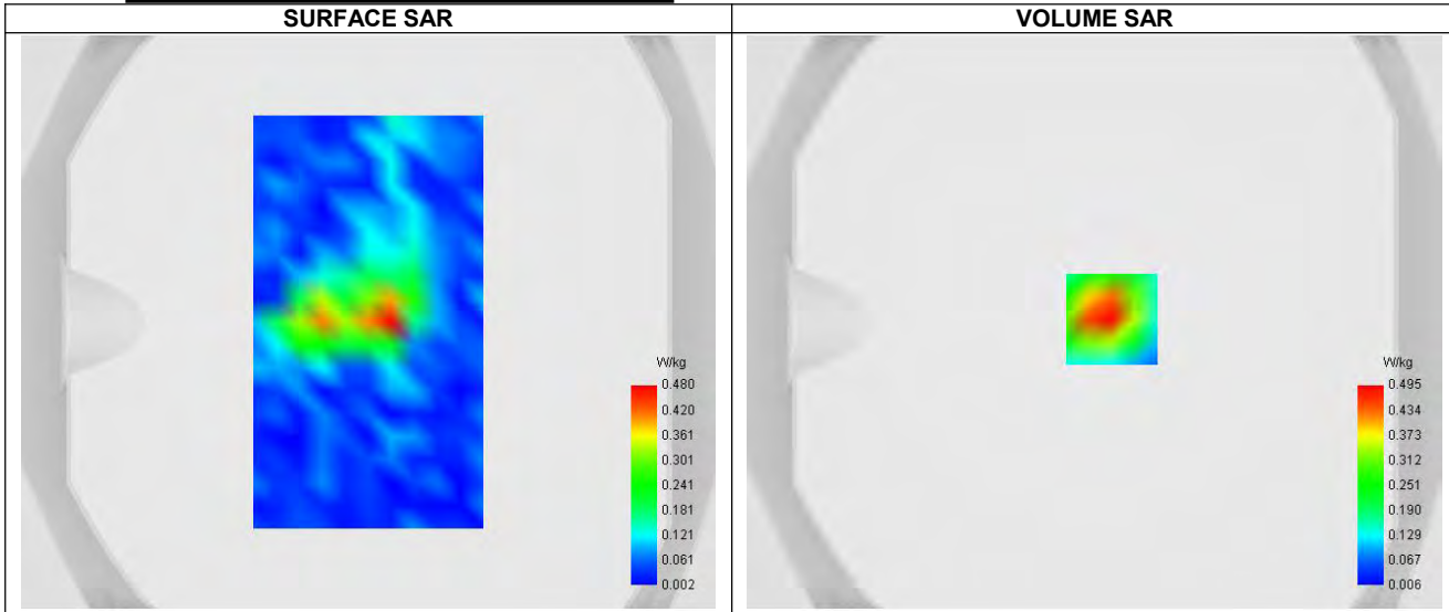
Maximum location: X=6.00, Y=1.00 ; SAR Peak: 0.96 W/kg
