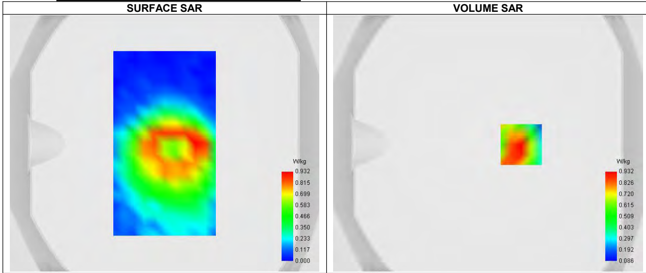
Maximum location: X=26.00, Y=-1.00 ; SAR Peak: 1.49 W/kg
