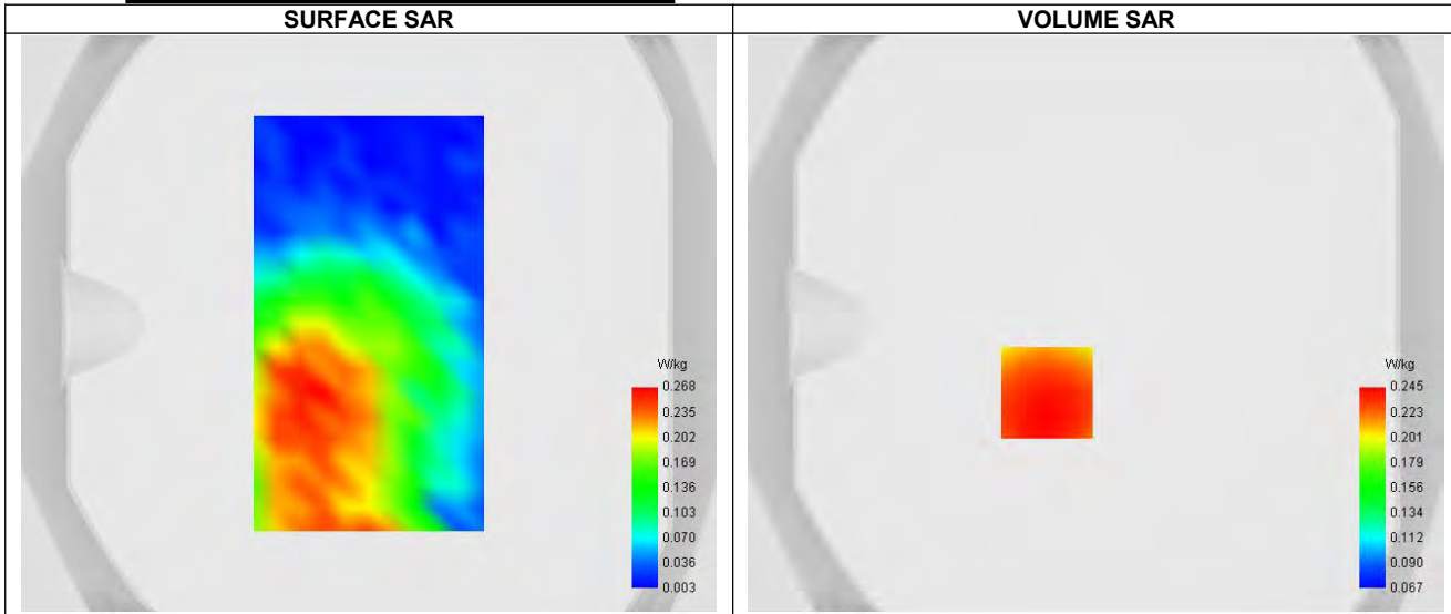
Maximum location: X=-17.00, Y=-24.00 ; SAR Peak: 0.30 W/kg
