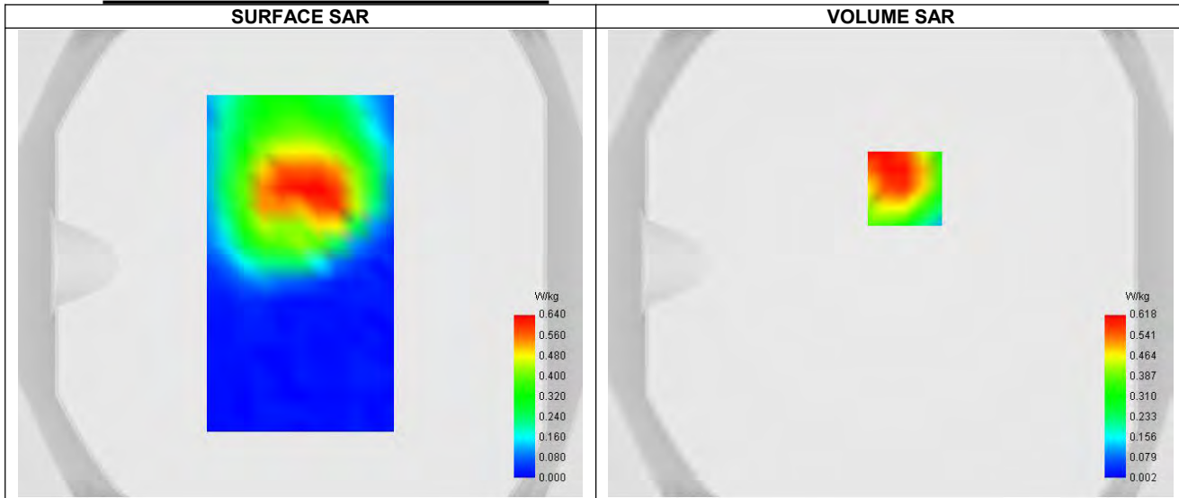
Maximum location: X=6.00, Y=32.00 ; SAR Peak: 1.00 W/kg
