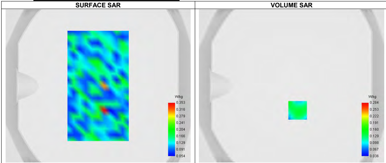
Maximum location: X=8.00, Y=-32.00 ; SAR Peak: 0.20 W/kg
