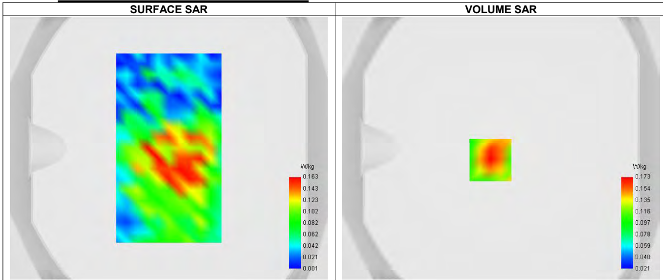
Maximum location: X=-8.00, Y=-9.00 ; SAR Peak: 0.32 W/kg
