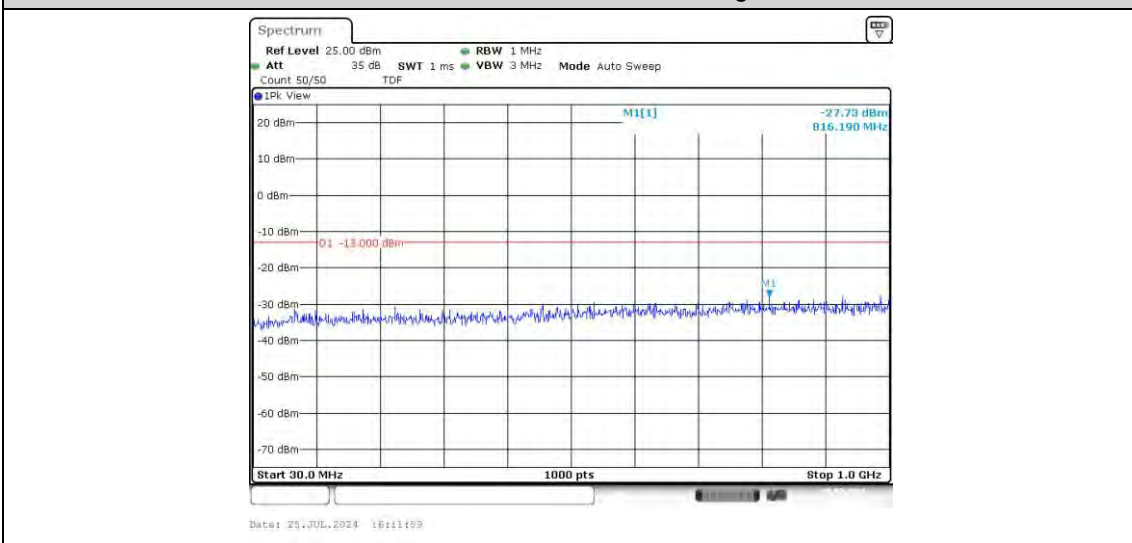
Band66-1.4MHz-16QAM-132322-1RB#0-Range2:1000~10000MHz
