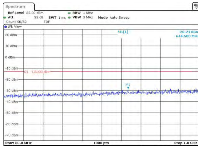
Band66-1.4MHz-QPSK-132322-1RB#0-Range1:30~1000MHz
