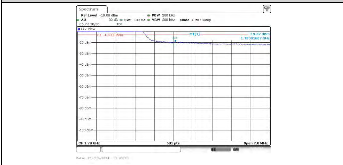
Band66-10MHz-16QAM-132022-50RB#0
