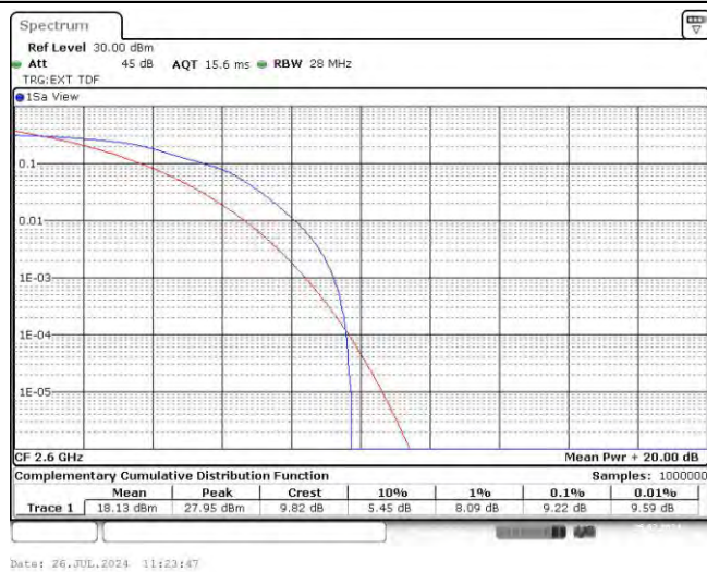
Band41-10MHz-16QAM-41540-50RB#0
