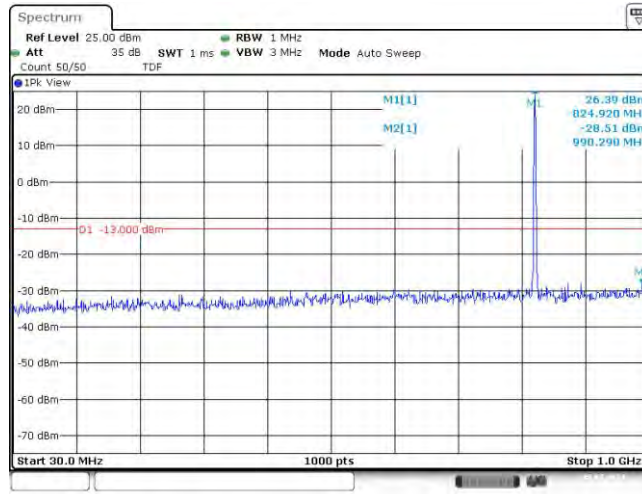
Band26-1.4MHz-QPSK-26797-6RB#0-Range1:30~1000MHz
