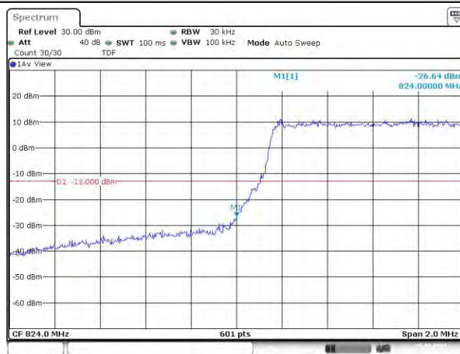
Band26-1.4MHz-16QAM-26797-6RB#0
