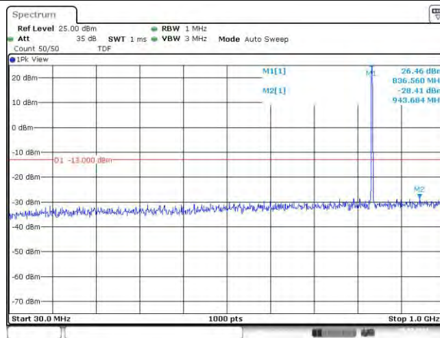
Band26-1.4MHz-QPSK-26915-6RB#0-Range1:30~1000MHz
