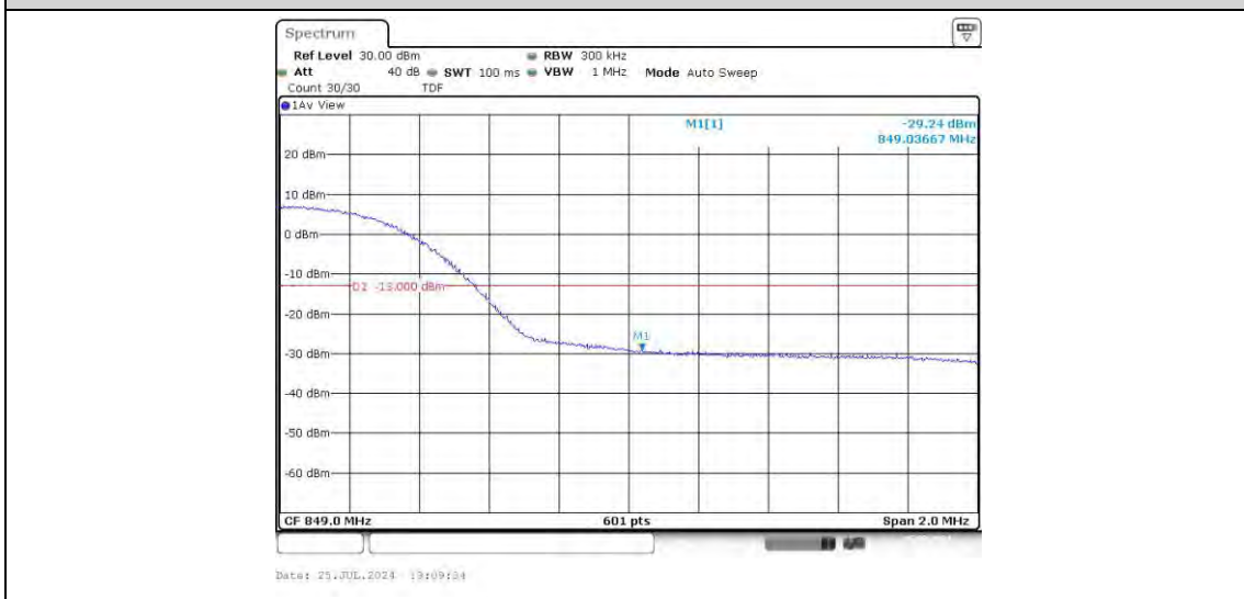
Band26-15MHz-16QAM-26865-75RB#0
