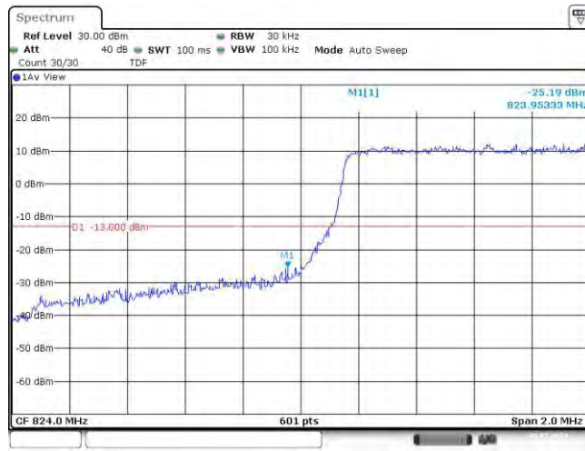
Band26-1.4MHz-QPSK-26797-6RB#0
