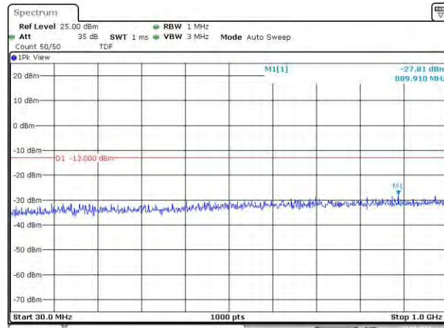
Band25-1.4MHz-QPSK-26047-1RB#0-Range1:30~1000MHz
