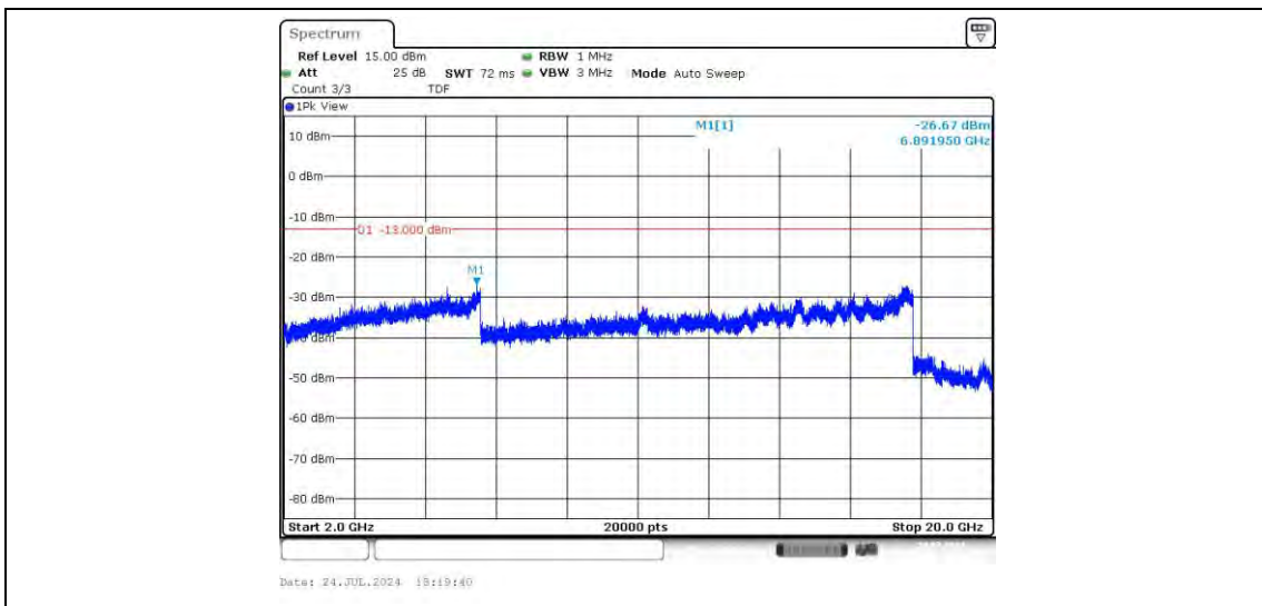
Band25-1.4MHz-QPSK-26365-1RB#0-Range1:30~1000MHz
