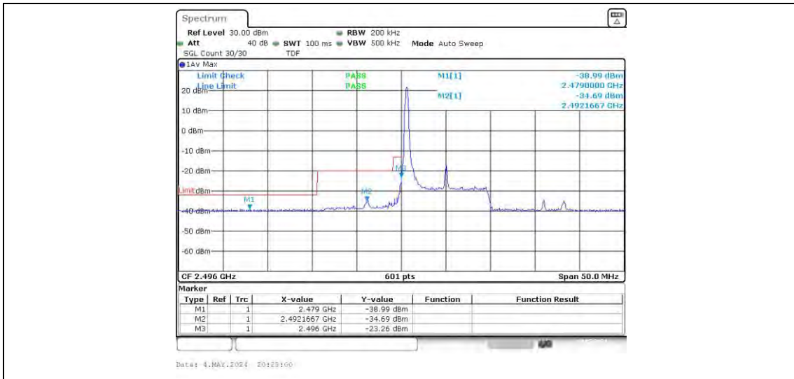
Band41-10MHz-QPSK-39700-1RB#49
