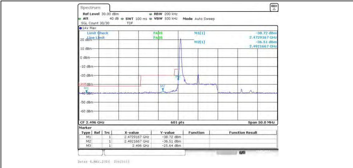
Band41-10MHz-16QAM-39700-1RB#49
