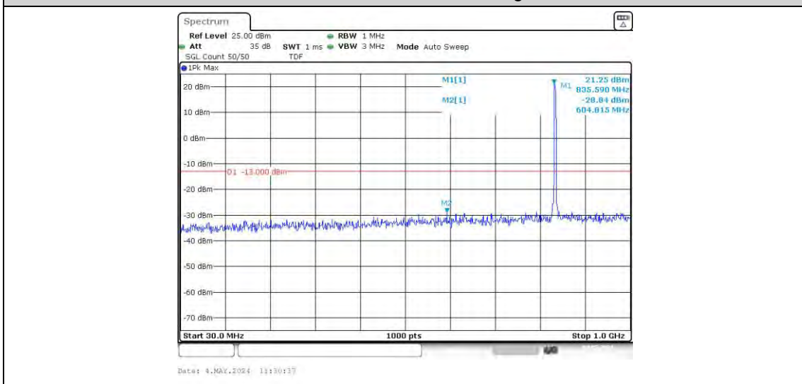
Band26-3MHz-16QAM-26915-15RB#0-Range2: 1000~10000MHz
