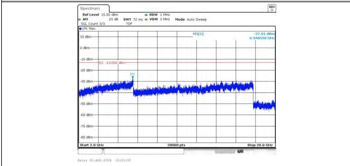
Band25-20MHz-16QAM-26590-100RB#0-Range3:2000~20000MHz
