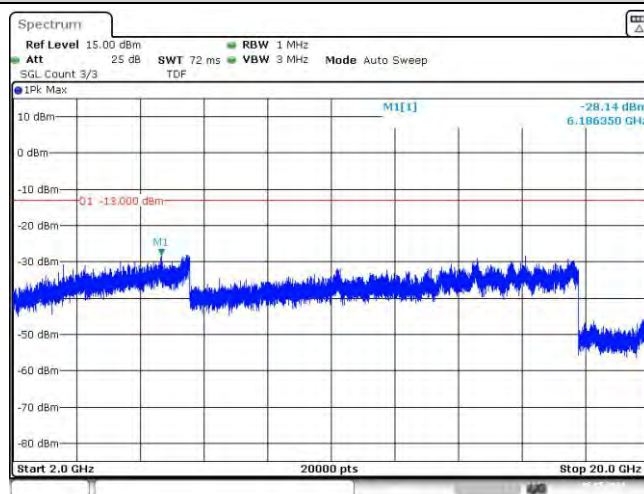
Band4-1.4MHz-QPSK-19957-6RB#0-Range3:2000~20000MHz
