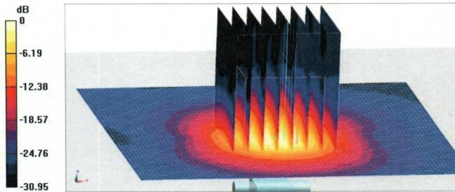
0 dB = 19.0 W/kg = 12.79 dBW/kg
