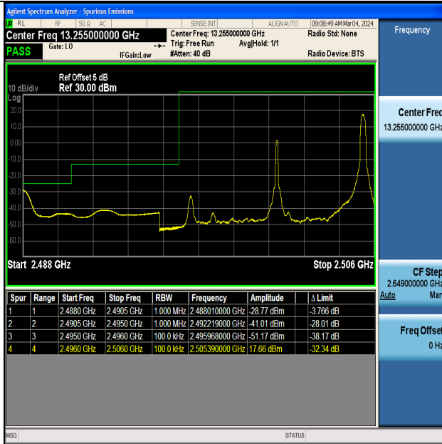
Band41_10MHz_QPSK_39700_1RB#49
