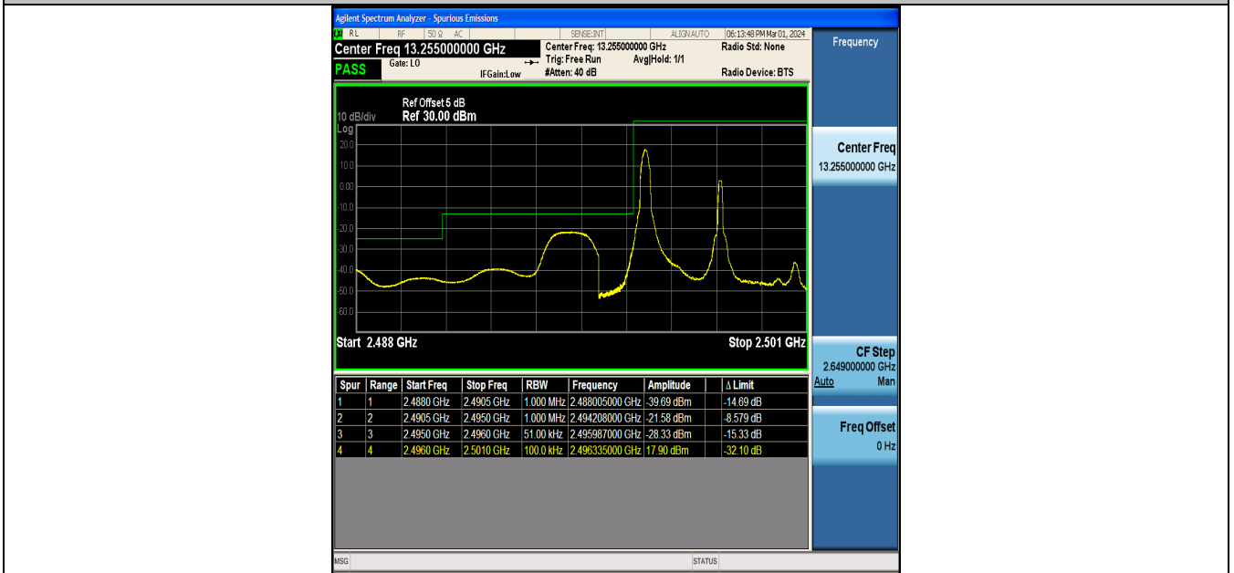
Band41_5MHz_16QAM_39675_1RB#0
