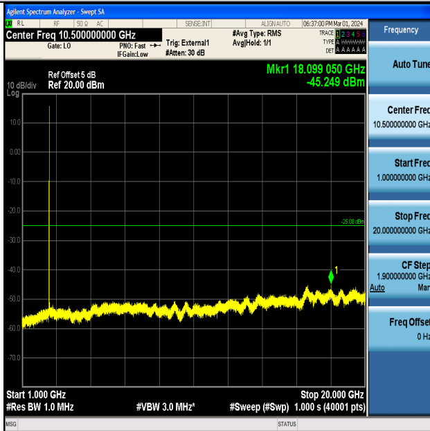
Band41_5MHz_QPSK_39675_1RB#0_1000~20000_1000~20000
