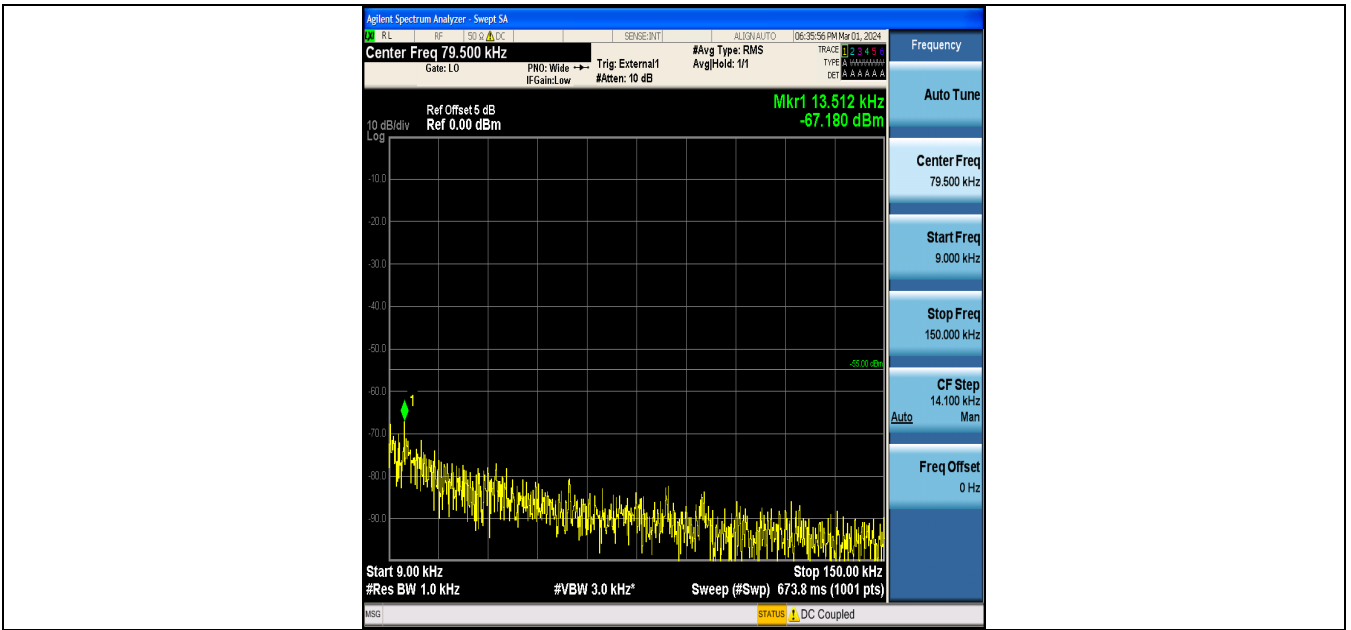
Band41_5MHz_QPSK_39675_1RB#0_0.009~0.15_0.009~0.15
