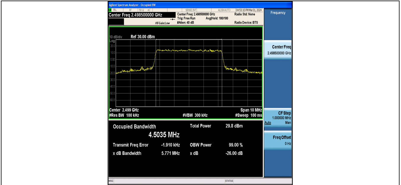
Band41-5MHz-QPSK-39675-25RB#0-PASS
