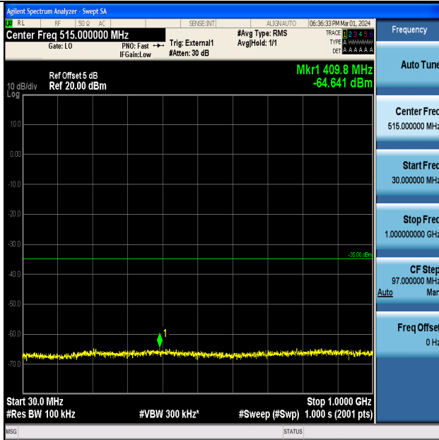
Band41_5MHz_QPSK_39675_1RB#0_30~1000_30~1000
