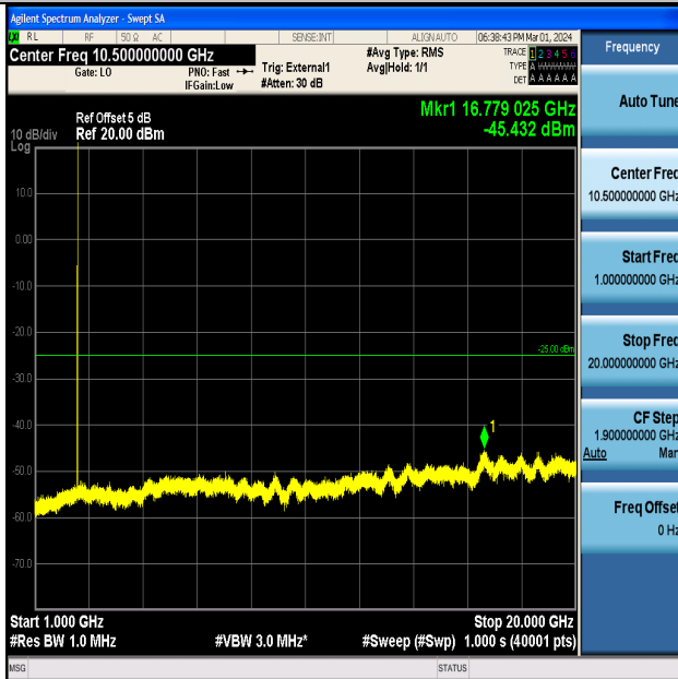
Band41_5MHz_16QAM_39675_1RB#0_1000~20000_1000~20000
