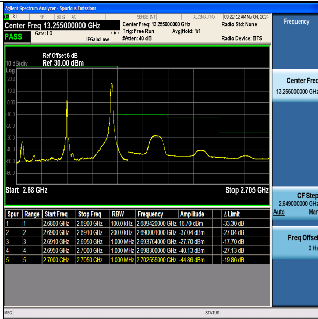
Band41_10MHz_16QAM_41540_1RB#49
