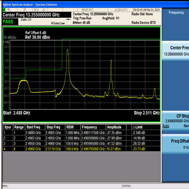
Band41_15MHz_16QAM_39725_1RB#0
