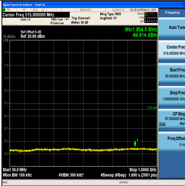
Band41_5MHz_16QAM_39675_1RB#0_30~1000_30~1000
