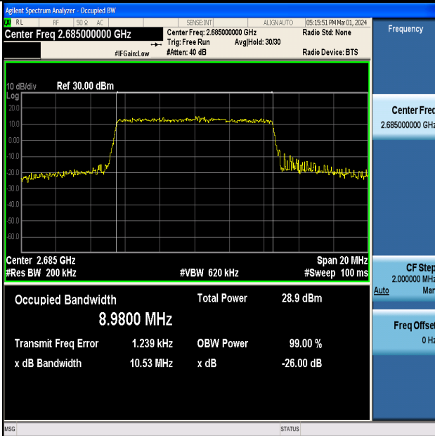
Band41-10MHz-16QAM-41540-50RB#0-PASS
