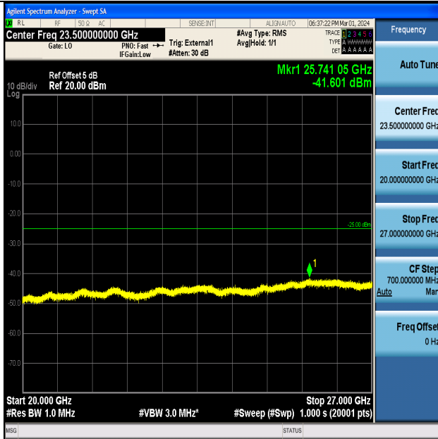
Band41_5MHz_QPSK_39675_1RB#0_20000~27000_20000~27000
