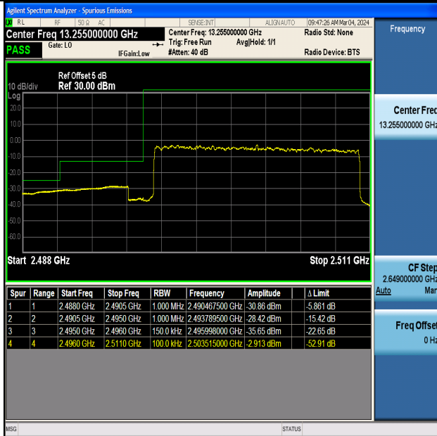
Band41_15MHz_16QAM_39725_75RB#0
