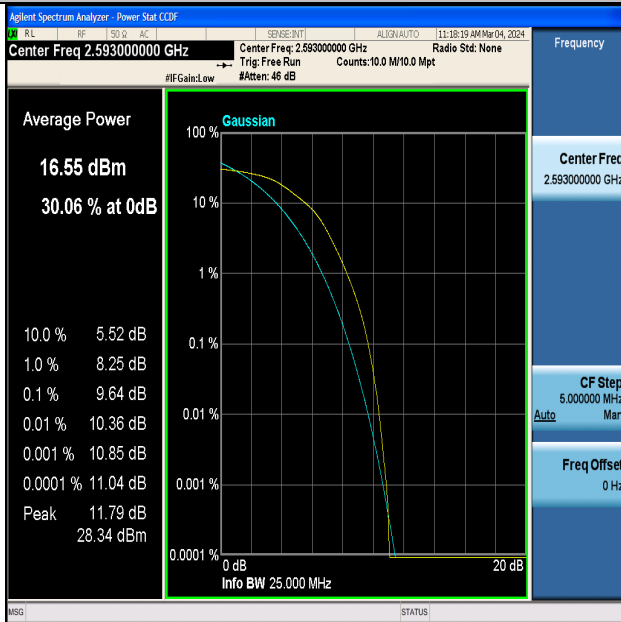
Band41-20MHz-16QAM-40620-100RB#0-PASS
