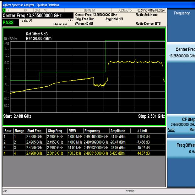
Band41_5MHz_QPSK_39675_25RB#0
