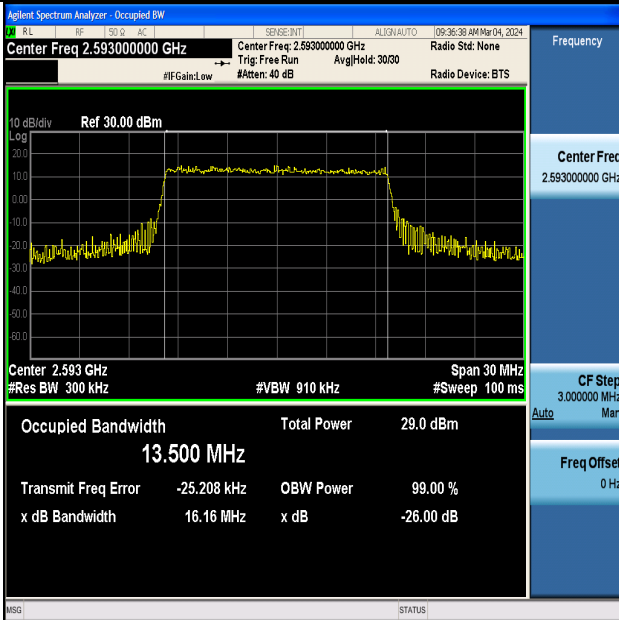
Band41-15MHz-16QAM-40620-75RB#0-PASS
