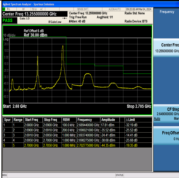
Band41_10MHz_QPSK_41540_1RB#49
