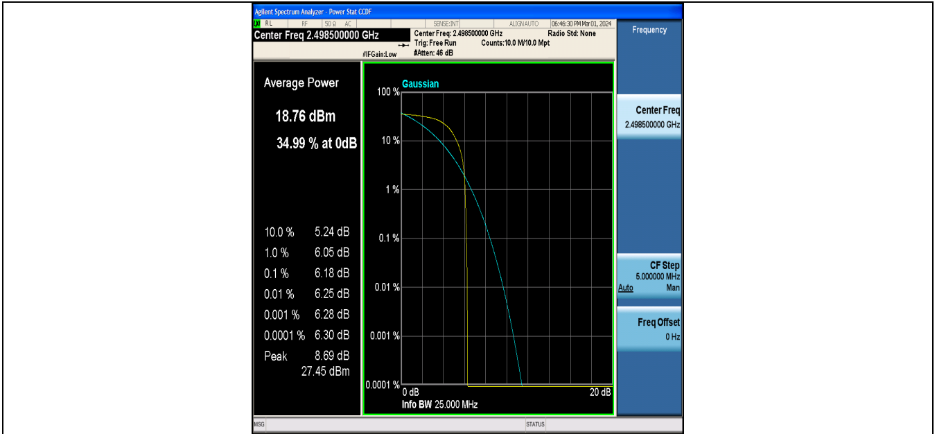
Band41-5MHz-QPSK-39675-1RB#0-PASS
