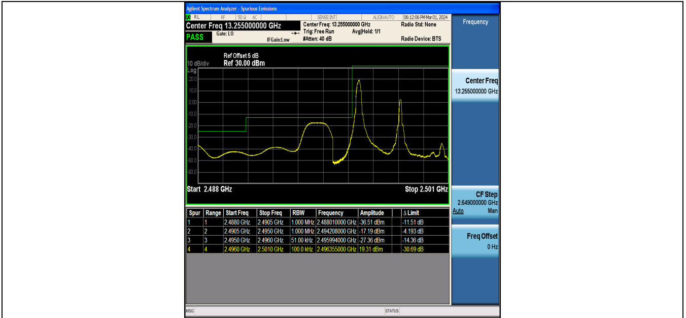
Band41_5MHz_QPSK_39675_1RB#0
