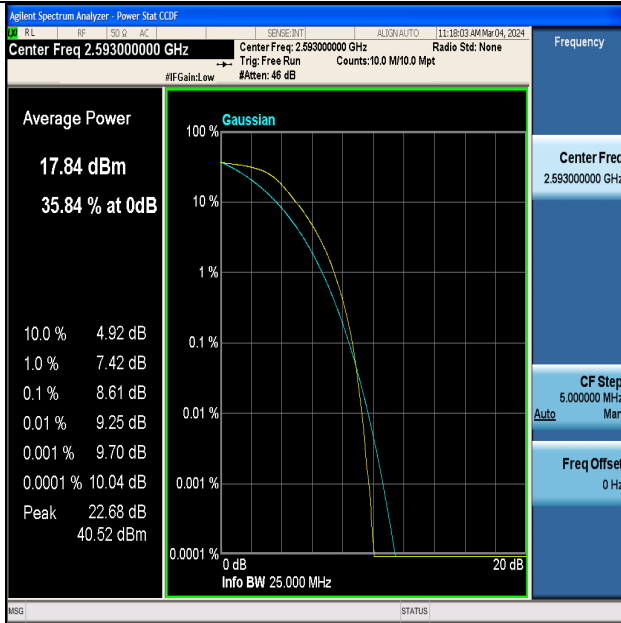
Band41-20MHz-QPSK-40620-100RB#0-PASS
