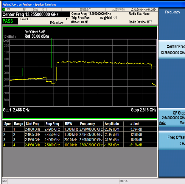
Band41_20MHz_QPSK_39750_100RB#0
