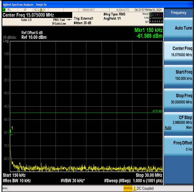
Band41_5MHz_16QAM_39675_1RB#0_0.15~30_0.15~30
