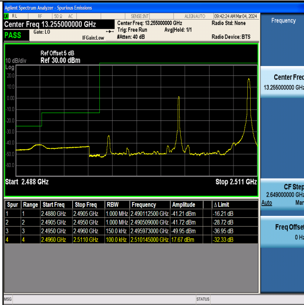
Band41_15MHz_QPSK_39725_1RB#74
