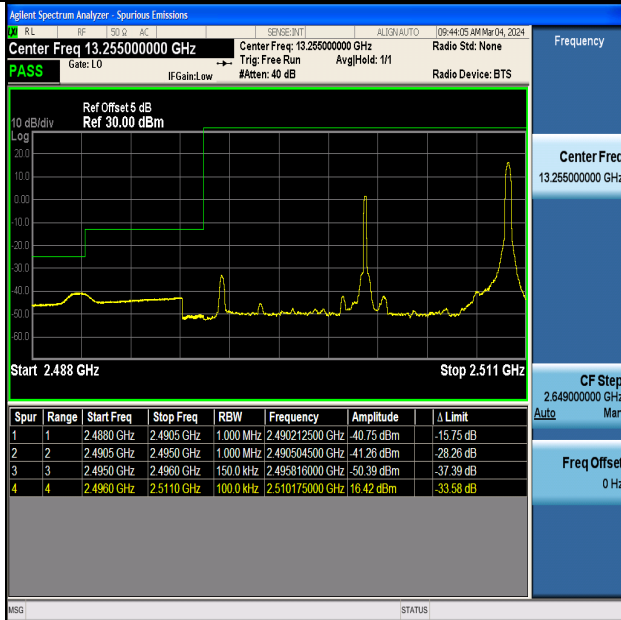
Band41_15MHz_16QAM_39725_1RB#74
