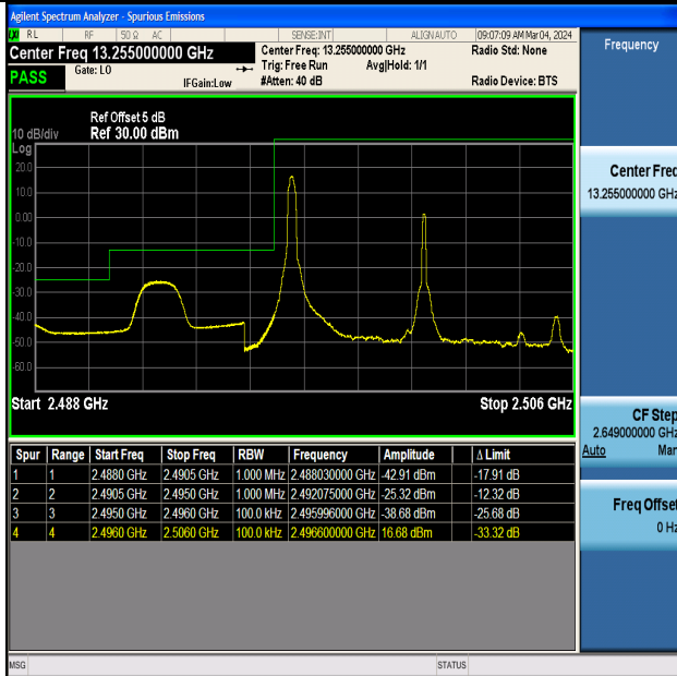
Band41_10MHz_16QAM_39700_1RB#0
