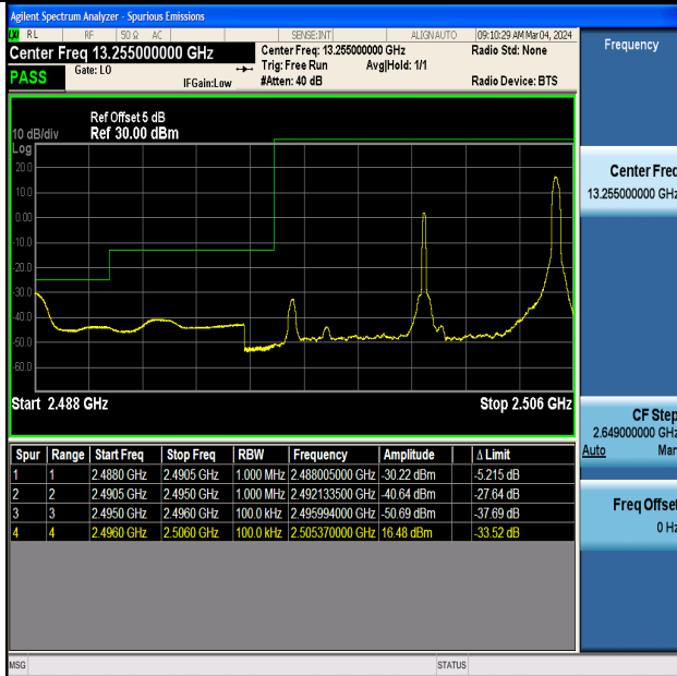
Band41_10MHz_16QAM_39700_1RB#49
