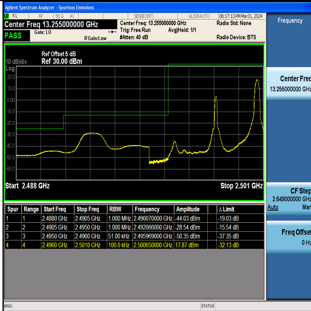
Band41_5MHz_16QAM_39675_1RB#24
