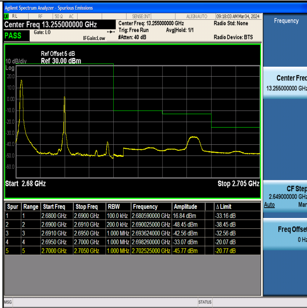
Band41_10MHz_16QAM_41540_1RB#0
