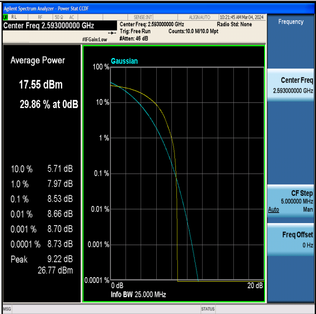
Band41-15MHz-16QAM-40620-1RB#0-PASS
