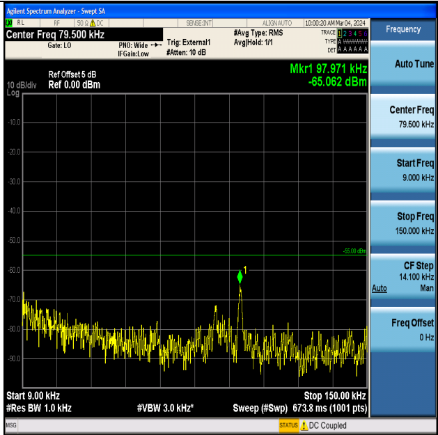
Band41_15MHz_QPSK_39725_1RB#0_0.009~0.15_0.009~0.15
