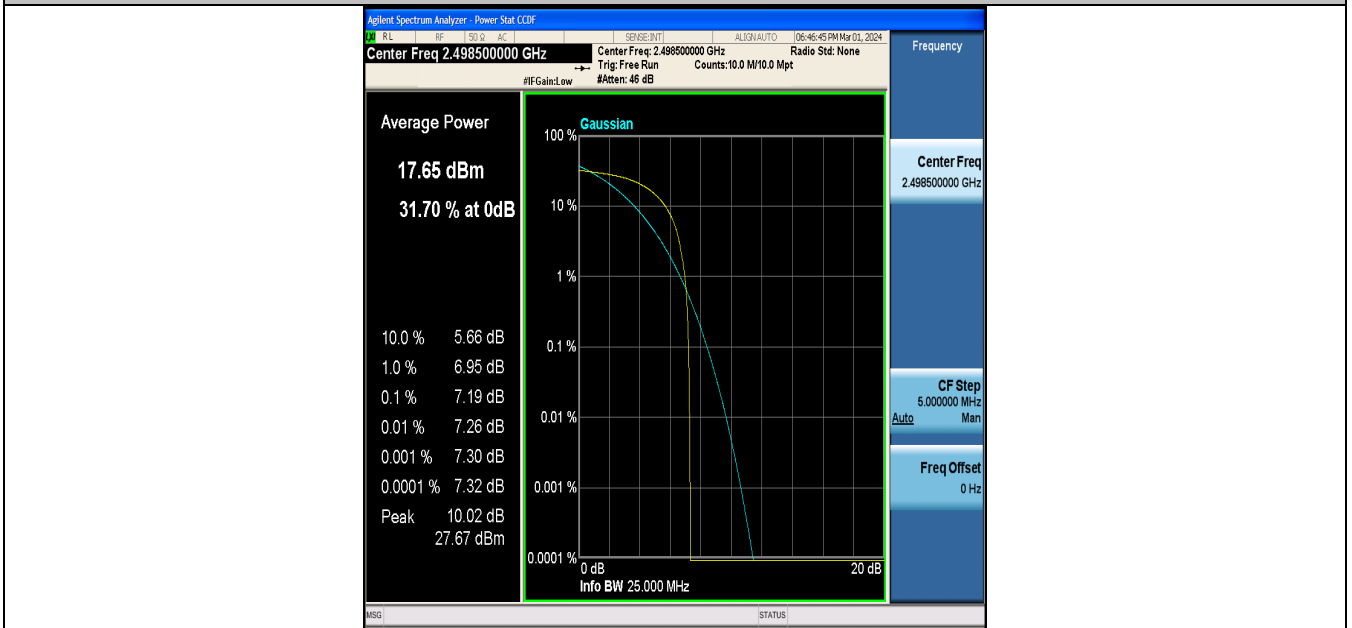
Band41-5MHz-16QAM-39675-1RB#0-PASS
