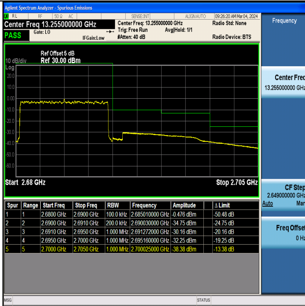
Band41_10MHz_16QAM_41540_50RB#0
