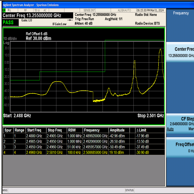
Band41_5MHz_QPSK_39675_1RB#24
