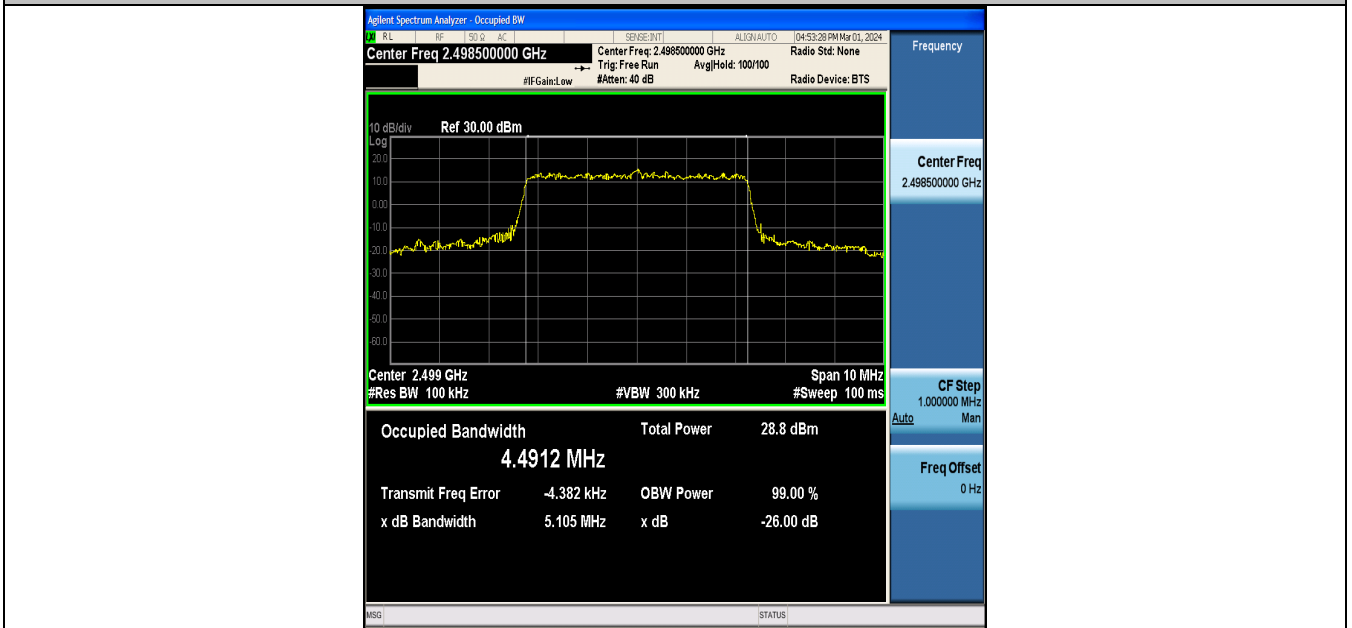
Band41-5MHz-16QAM-39675-25RB#0-PASS
