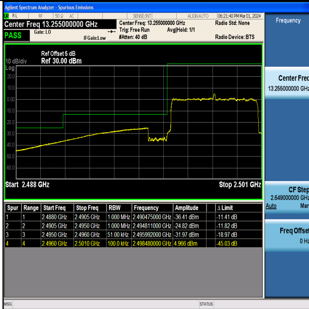
Band41_5MHz_16QAM_39675_25RB#0
