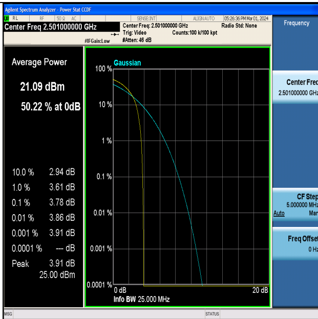
Band41-10MHz-16QAM-39700-1RB#0-PASS
