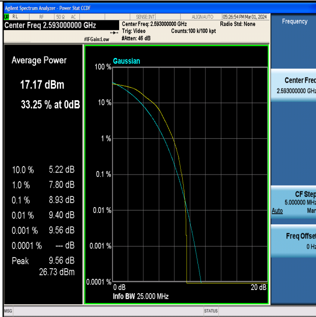
Band41-10MHz-16QAM-40620-50RB#0-PASS
