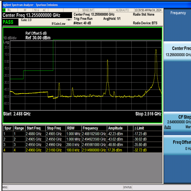
Band41_20MHz_16QAM_39750_1RB#99
