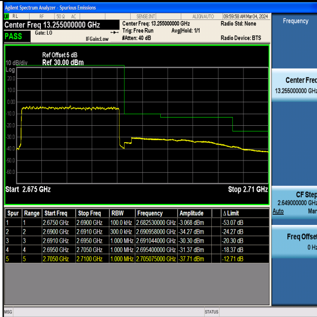
Band41_15MHz_16QAM_41515_75RB#0
