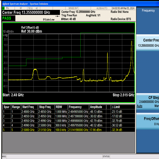
Band7_15MHz_16QAM_20825_1RB#74
