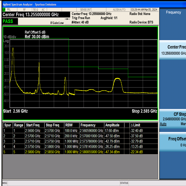
Band7_10MHz_16QAM_21400_1RB#0
