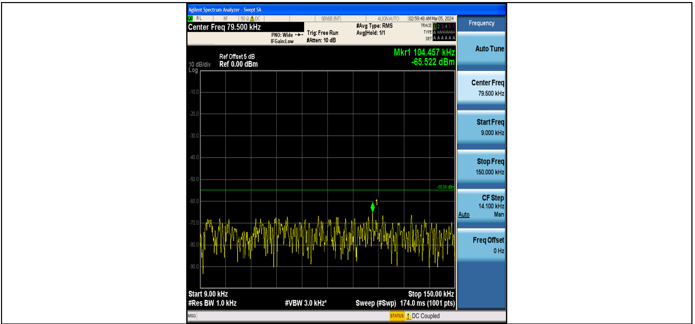
Band7_5MHz_QPSK_20775_1RB#0_0.009~0.15_0.009~0.15
