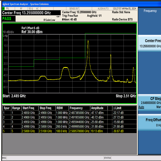
Band7_10MHz_QPSK_20800_1RB#0
