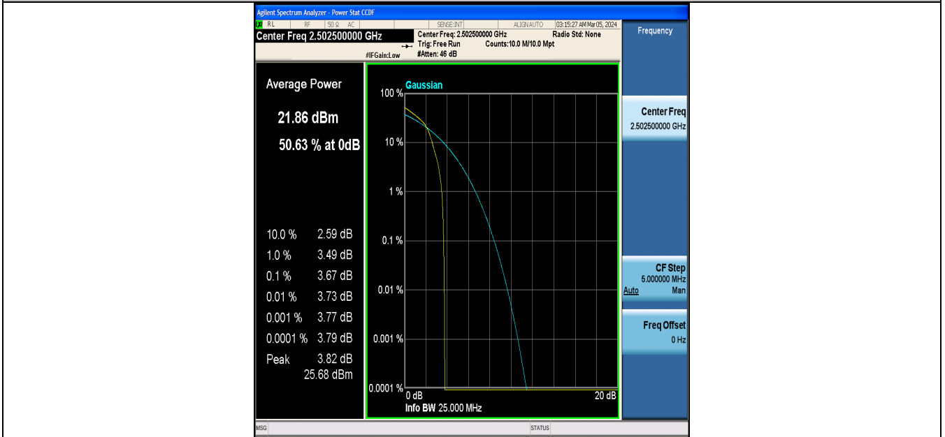
Band7-5MHz-16QAM-20775-1RB#0-PASS
