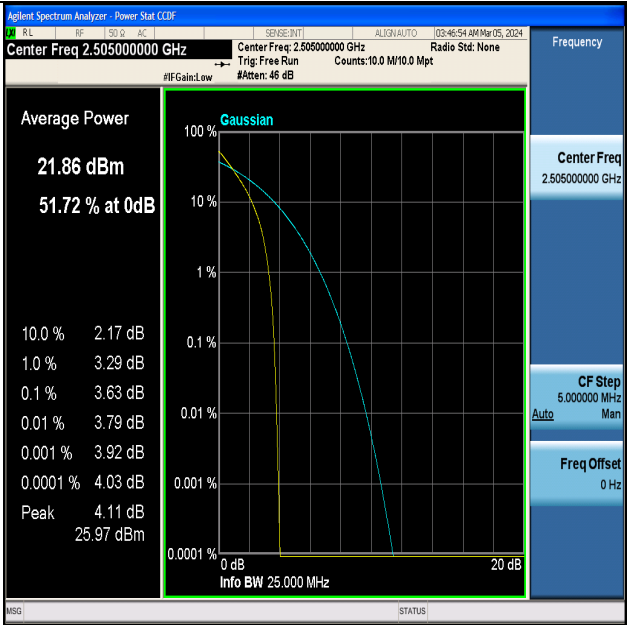
Band7-10MHz-QPSK-20800-50RB#0-PASS
