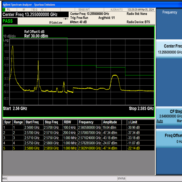
Band7_10MHz_QPSK_21400_1RB#0
