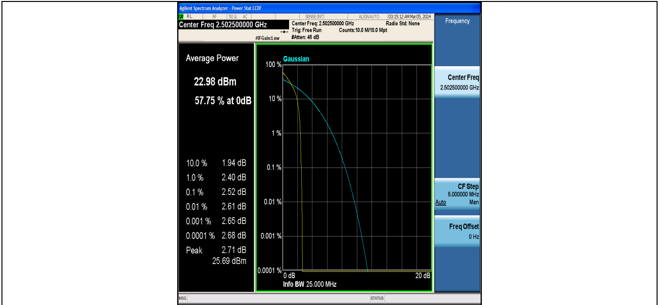
Band7-5MHz-QPSK-20775-1RB#0-PASS
