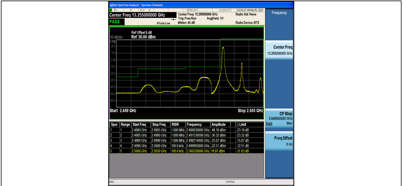
Band7_5MHz_QPSK_20775_1RB#0
