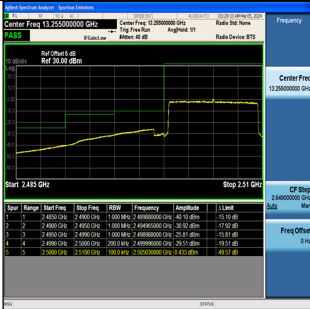
Band7_10MHz_16QAM_20800_50RB#0
