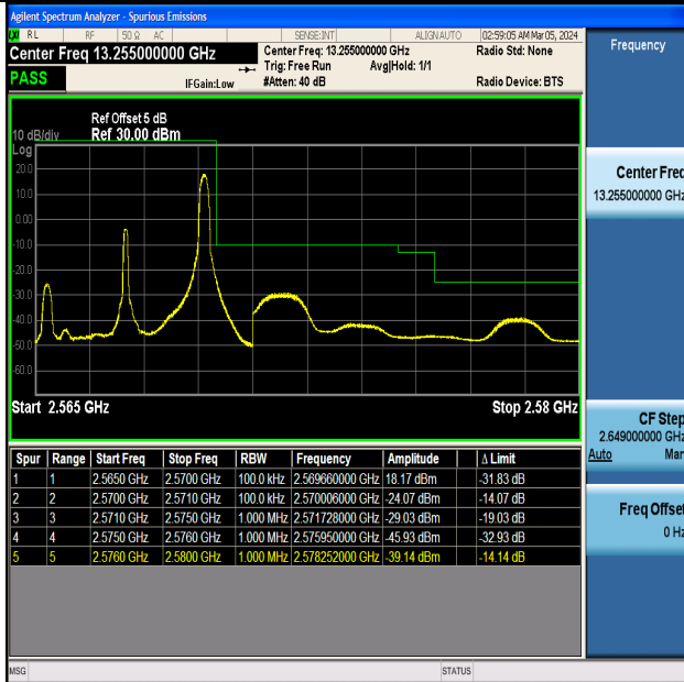
Band7_5MHz_16QAM_21425_1RB#24
