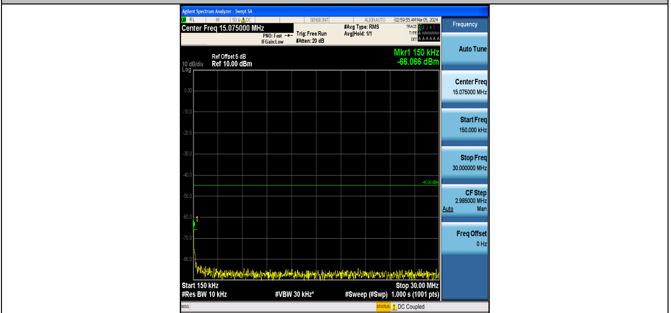
Band7_5MHz_QPSK_20775_1RB#0_0.15~30_0.15~30
