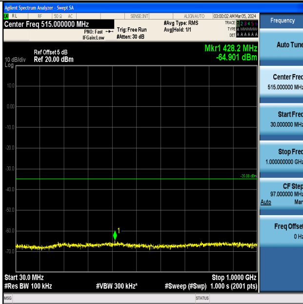
Band7_5MHz_QPSK_20775_1RB#0_30~1000_30~1000
