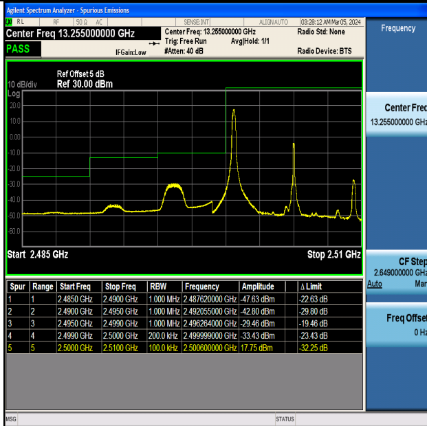
Band7_10MHz_16QAM_20800_1RB#0
