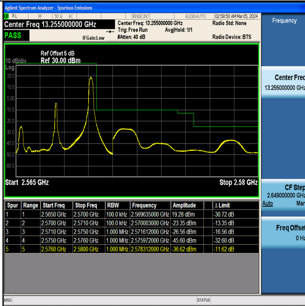
Band7_5MHz_QPSK_21425_1RB#24
