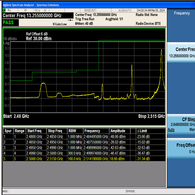
Band7_15MHz_QPSK_20825_1RB#74
