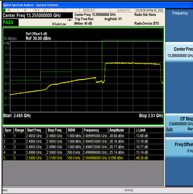
Band7_10MHz_QPSK_20800_50RB#0
