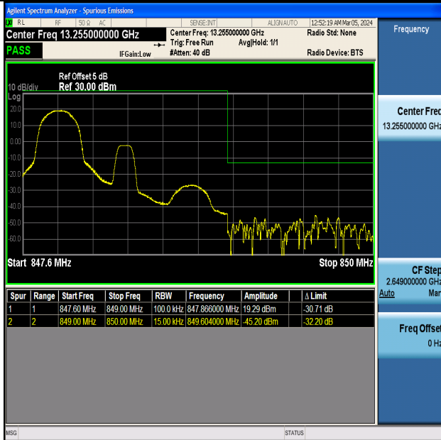
Band5_1.4MHz_16QAM_20643_1RB#0
