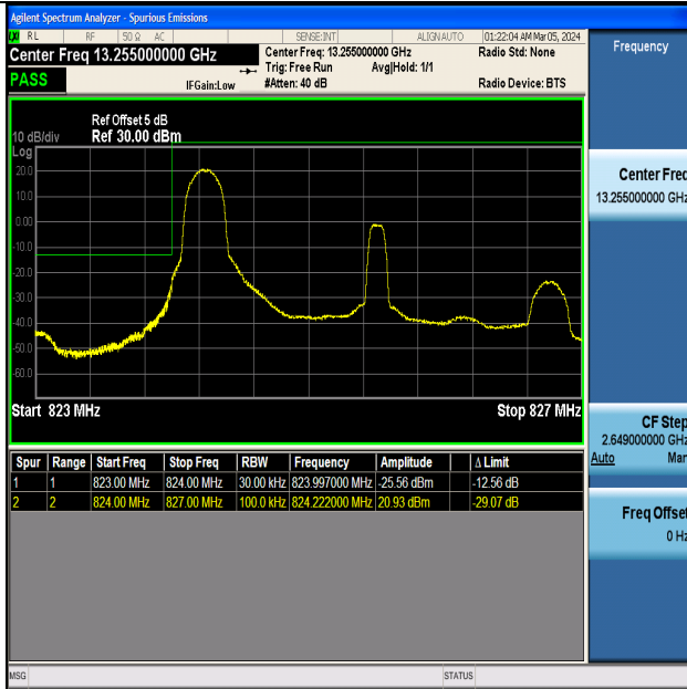
Band5_3MHz_QPSK_20415_1RB#0
