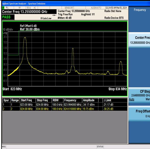
Band5_10MHz_16QAM_20450_1RB#0
