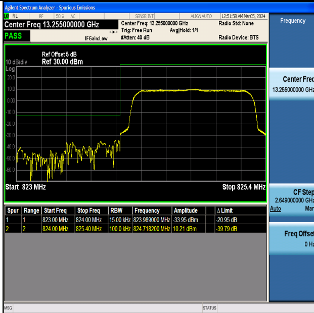
Band5_1.4MHz_16QAM_20407_6RB#0
