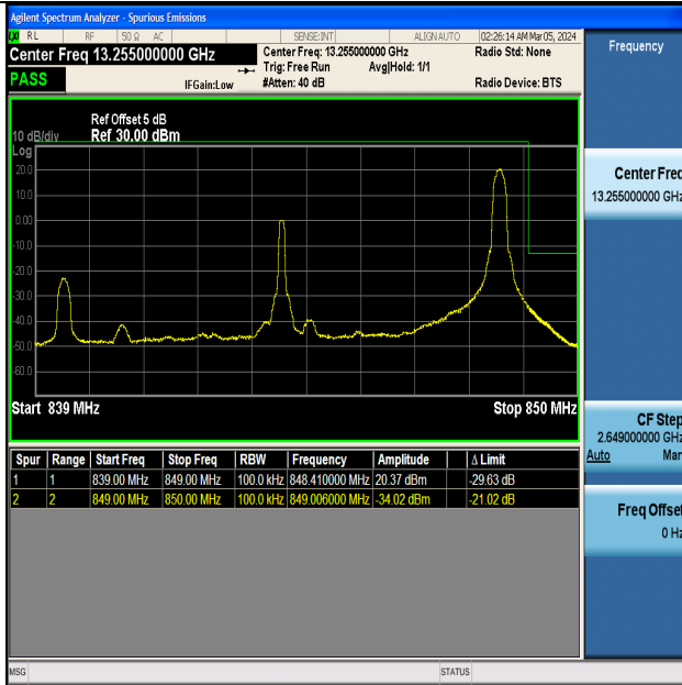
Band5_10MHz_QPSK_20600_1RB#49
