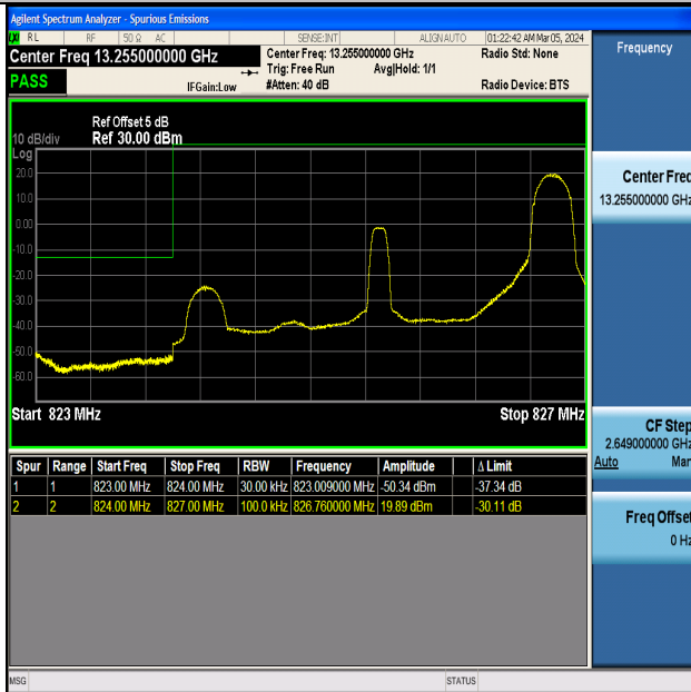
Band5_3MHz_16QAM_20415_1RB#14
