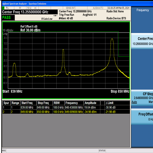
Band5_10MHz_16QAM_20600_1RB#49
