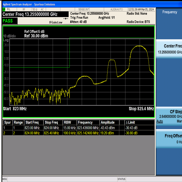
Band5_1.4MHz_16QAM_20407_1RB#5
