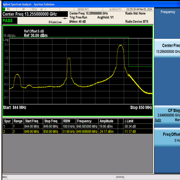
Band5_5MHz_16QAM_20625_1RB#24
