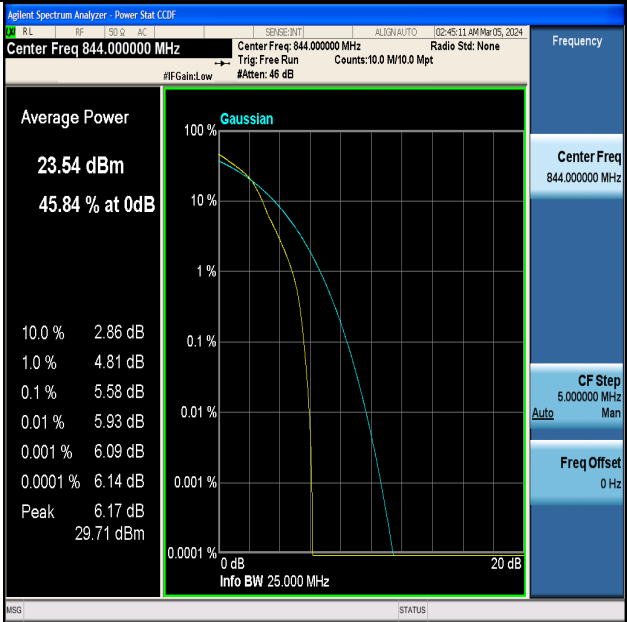
Band5-10MHz-16QAM-20600-1RB#0-PASS
