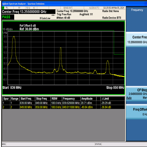
Band5_10MHz_QPSK_20600_1RB#0
