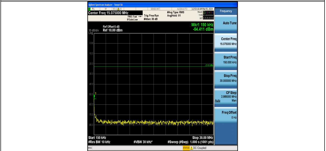
Band5_1.4MHz_QPSK_20407_1RB#0_0.15~30_0.15~30
