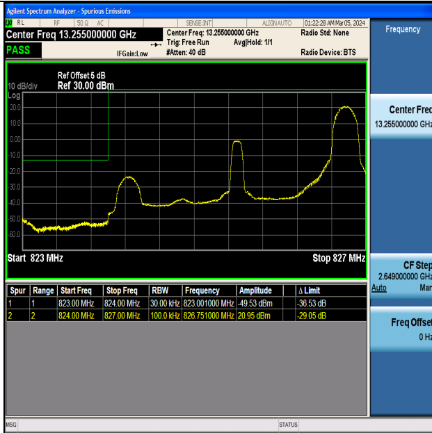
Band5_3MHz_QPSK_20415_1RB#14
