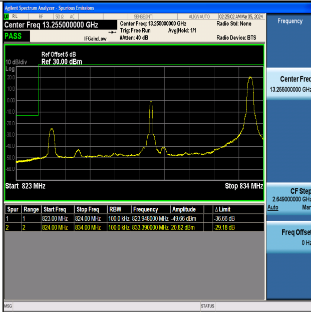
Band5_10MHz_QPSK_20450_1RB#49
