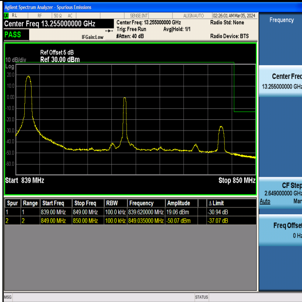
Band5_10MHz_16QAM_20600_1RB#0
