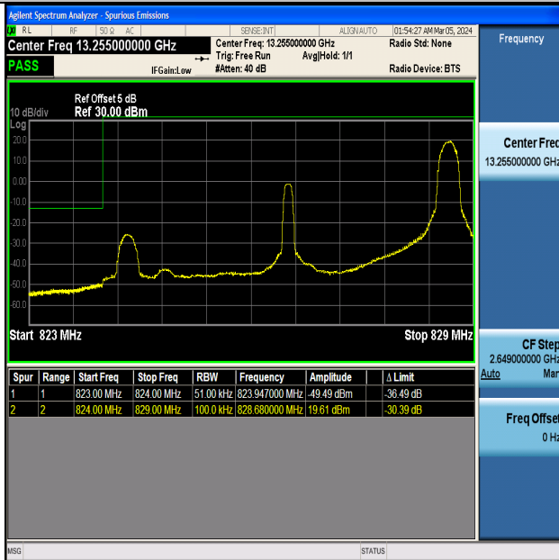
Band5_5MHz_16QAM_20425_1RB#24
