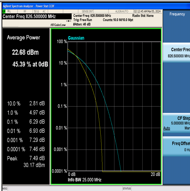
Band5-5MHz-16QAM-20425-25RB#0-PASS
