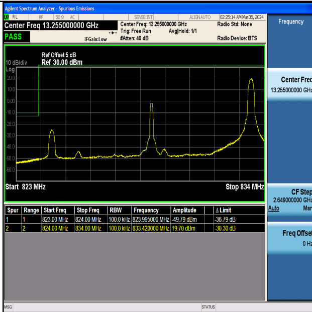
Band5_10MHz_16QAM_20450_1RB#49
