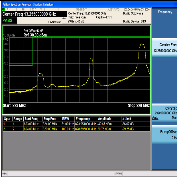
Band5_5MHz_QPSK_20425_1RB#24
