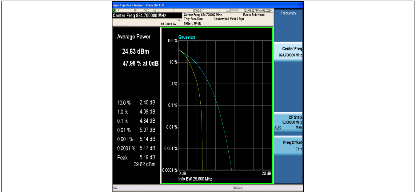
Band5-1.4MHz-QPSK-20407-1RB#0-PASS
