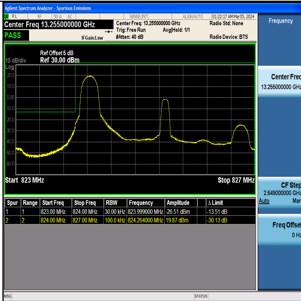
Band5_3MHz_16QAM_20415_1RB#0
