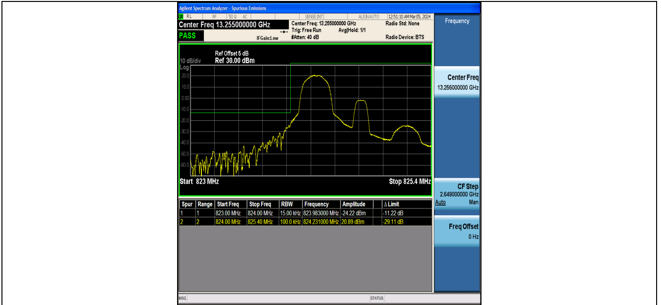
Band5_1.4MHz_QPSK_20407_1RB#0
