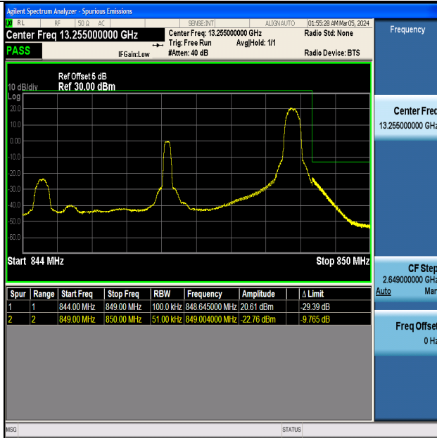
Band5_5MHz_QPSK_20625_1RB#24
