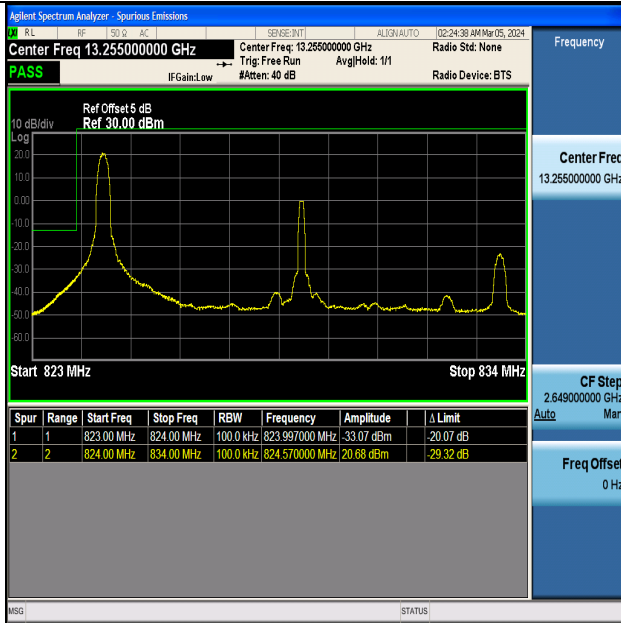
Band5_10MHz_QPSK_20450_1RB#0
