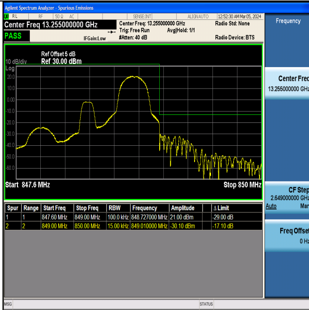
Band5_1.4MHz_QPSK_20643_1RB#5
