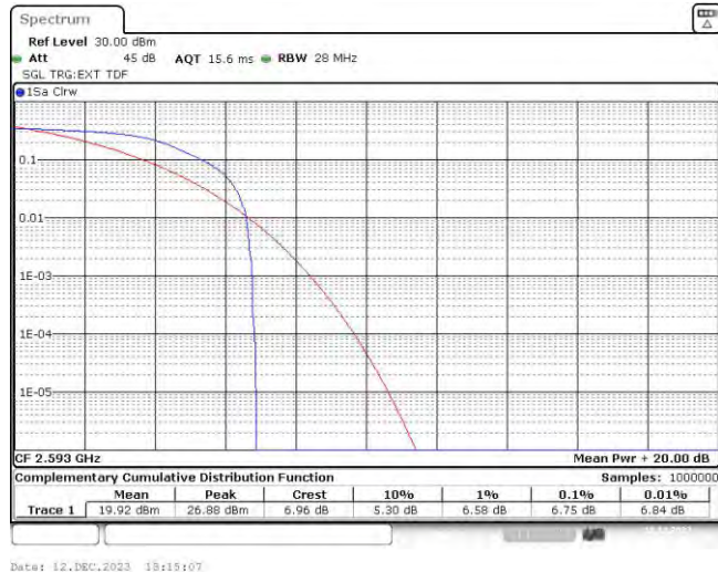
Band41-5MHz-QPSK-40620-25RB#0
