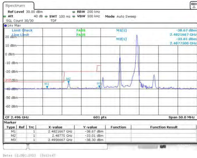
Band41-10MHz-16QAM-39700-50RB#0
