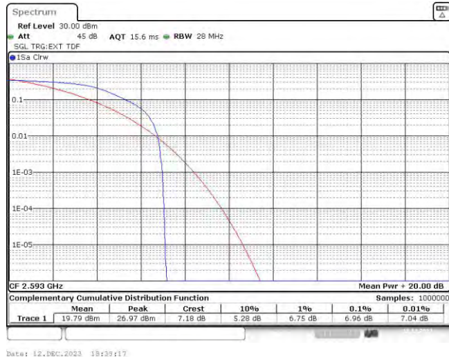
Band41-10MHz-QPSK-40620-50RB#0
