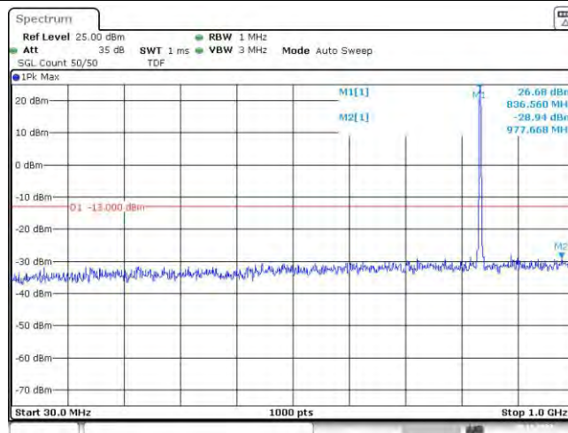
Band26-1.4MHz-QPSK-26915-6RB#0-Range1:30~1000MHz
