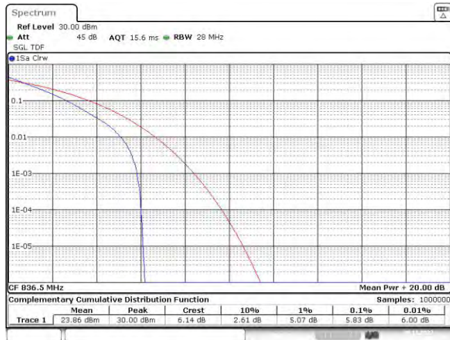
Band26-1.4MHz-QPSK-26915-6RB#0
