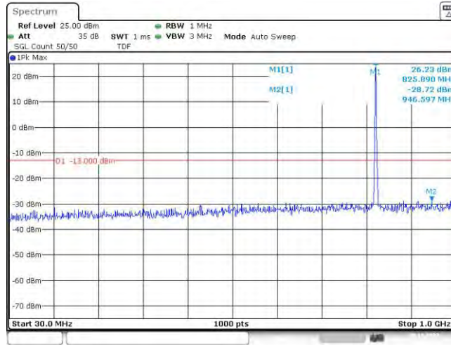
Band26-1.4MHz-QPSK-26797-6RB#0-Range1:30~1000MHz
