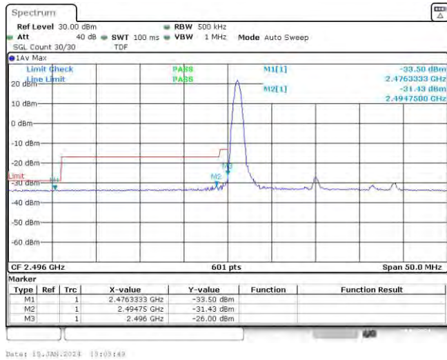
Band41-20MHz-16QAM-39750-1RB#99
