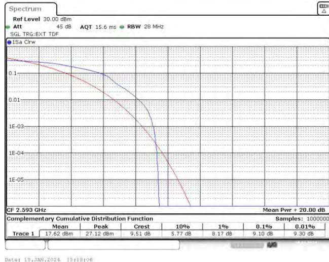
Band41-20MHz-16QAM-40620-100RB#0
