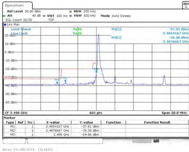
Band41-10MHz-16QAM-39700-1RB#49
