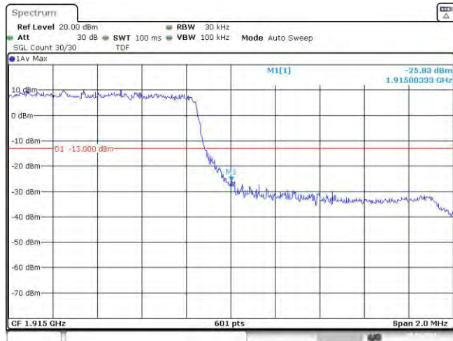
Band25-1.4MHz-QPSK-26683-6RB#0
