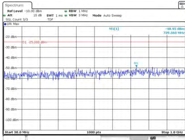
Band41-5MHz-QPSK-39675-1RB#0-Range1:30~1000MHz
