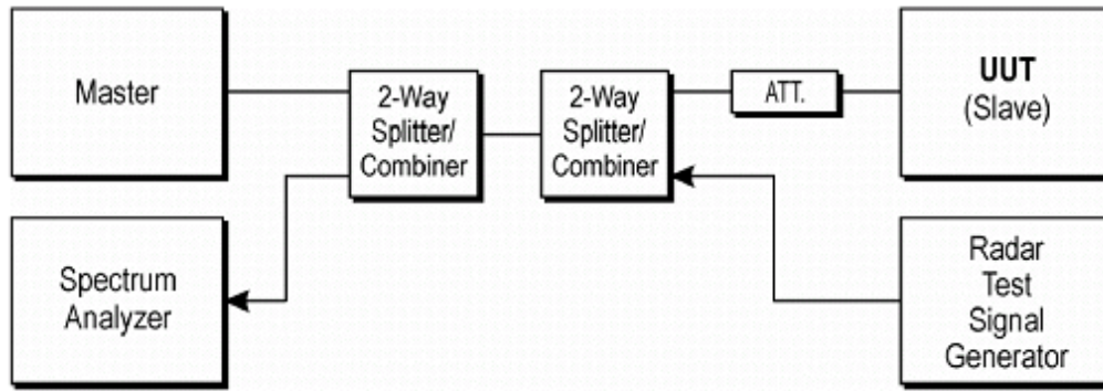
Figure 7-1. Test Setup
