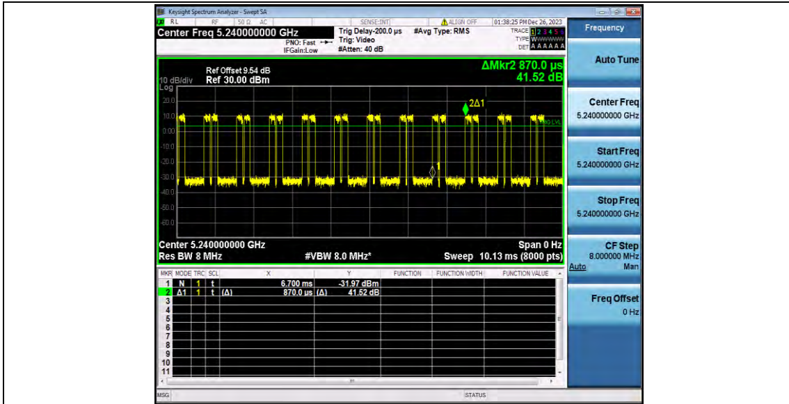
11AX20SISO_Ant1_5240
