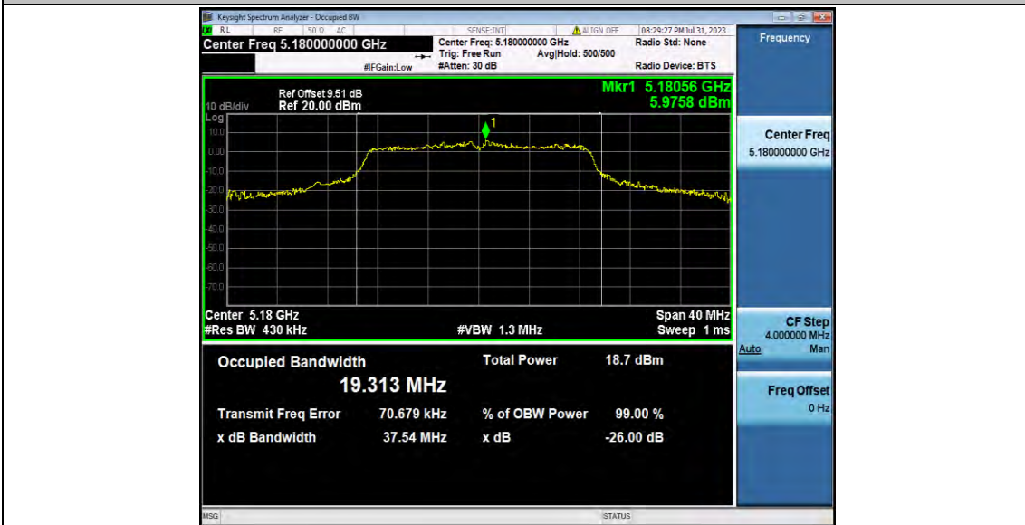
11A20SISO_Ant1_5180
