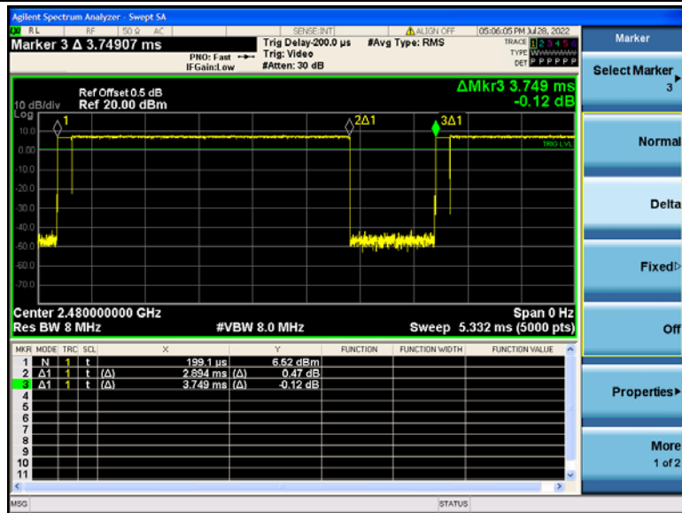
8-DPSK_2480
