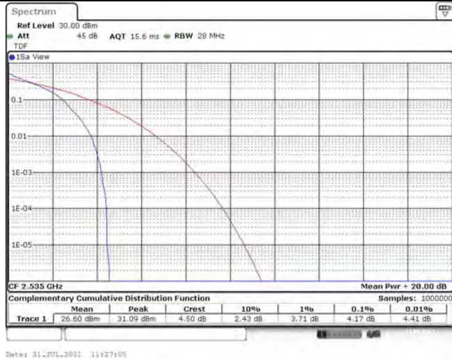
Band7-5MHz-QPSK-21100-1RB#0
