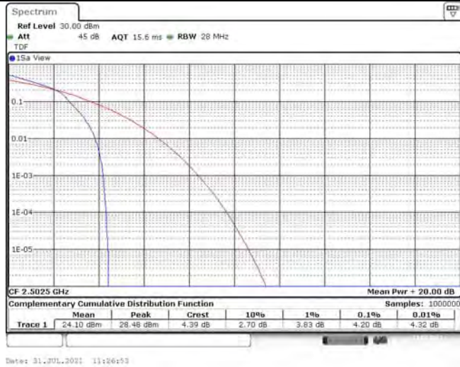
Band7-5MHz-16QAM-21100-1RB#0
