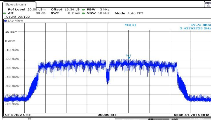
11N40SISO_Ant1_2422
