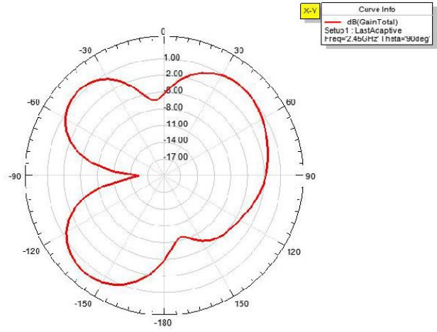
Radiation Pattern 2
