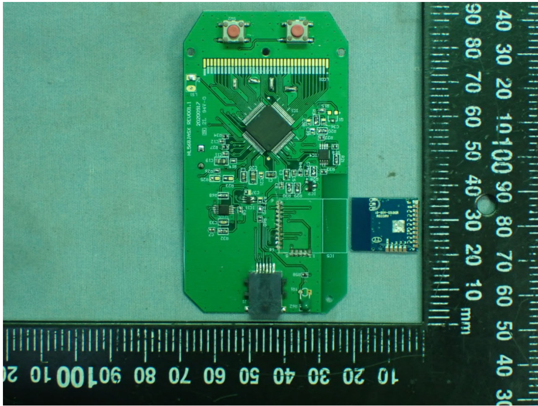
Figure 15 Main Board (Removed BLE Module)
