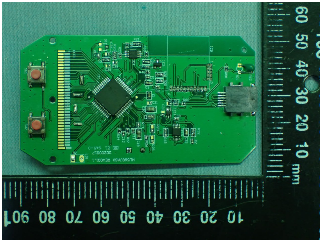
Figure 16 Main Board (without BLE Module), Front View
