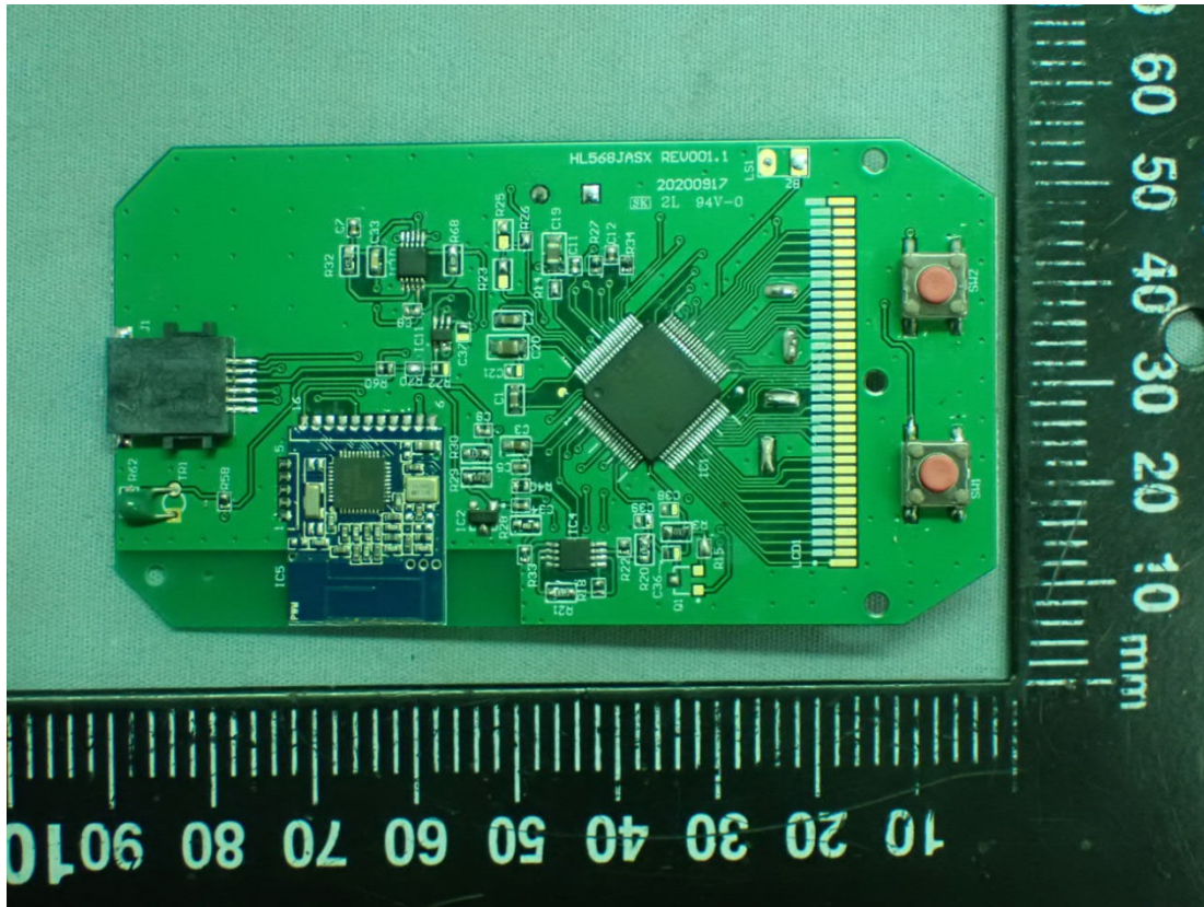
Figure 13 Main Board (with BLE Module), Front View
