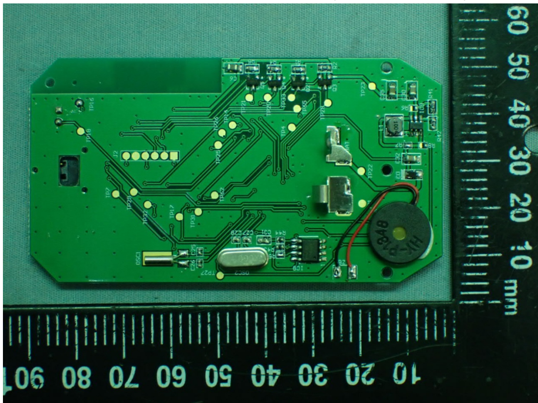
Figure 14 Main Board (with BLE Module), Back View
