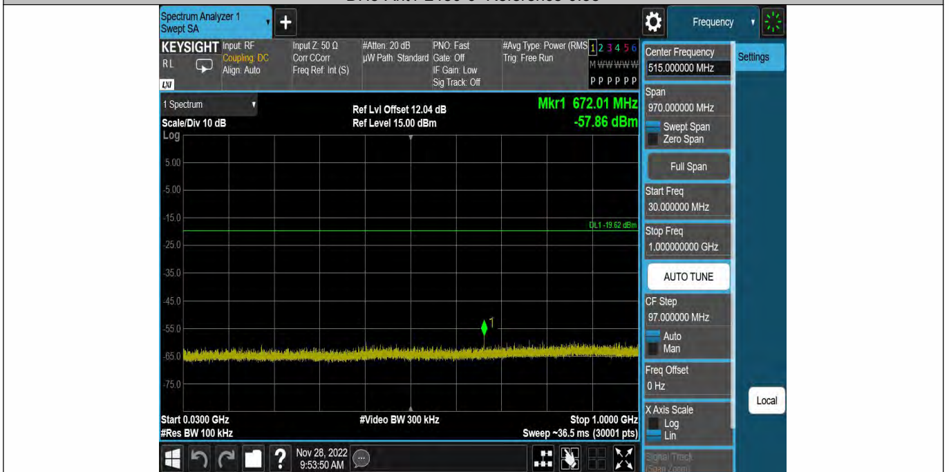
DH5-Ant1-2480-30~1000-0.38
