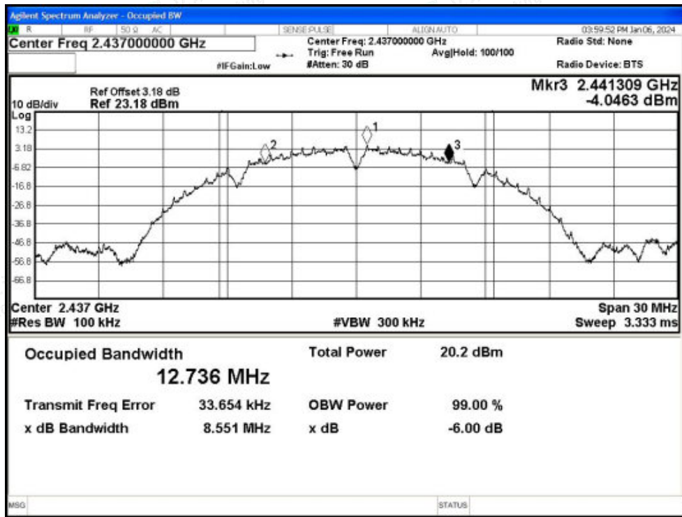
-6dB Bandwidth NVNT b 2437MHz Ant3
