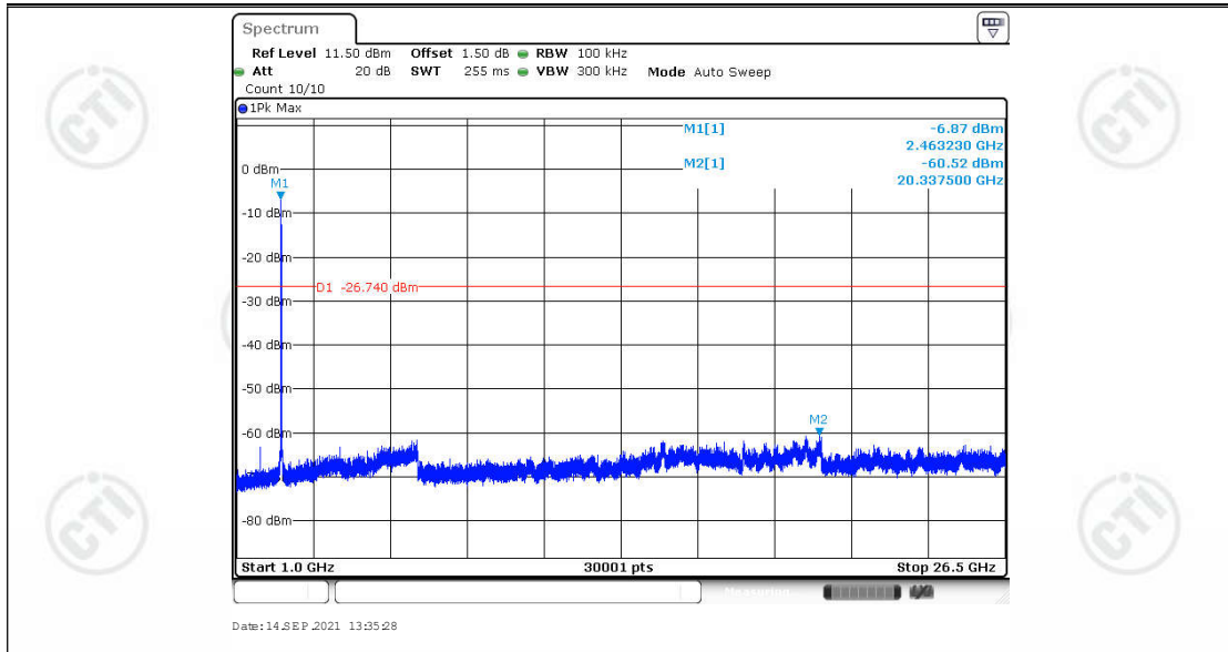
11N20SISO_Ant1_2462_1000~26500
