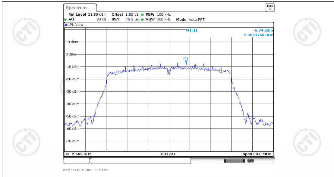
11N20SISO_Ant1_2462_0~Reference
