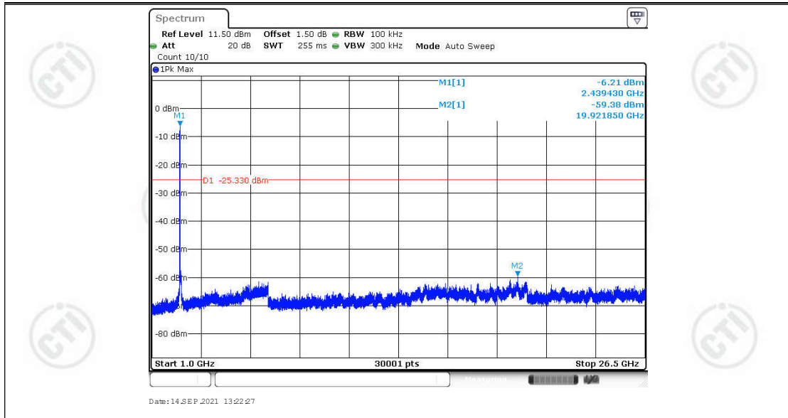
11G_Ant1_2437_1000~26500
