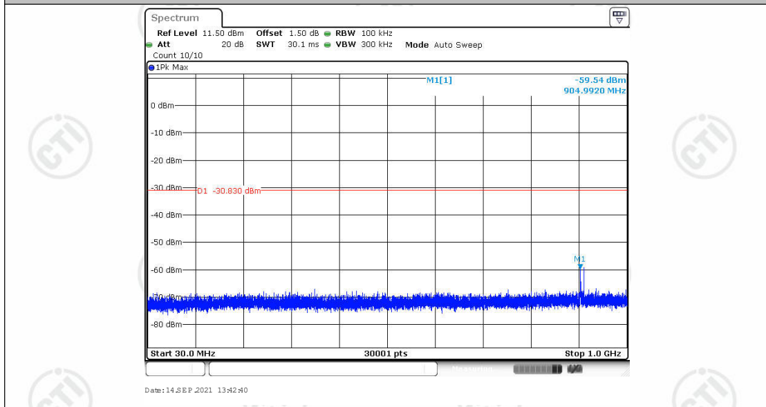
11N40SISO_Ant1_2437_30~1000
