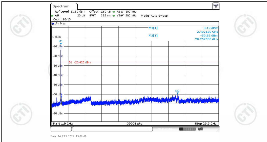
11N20SISO_Ant1_2412_1000~26500
