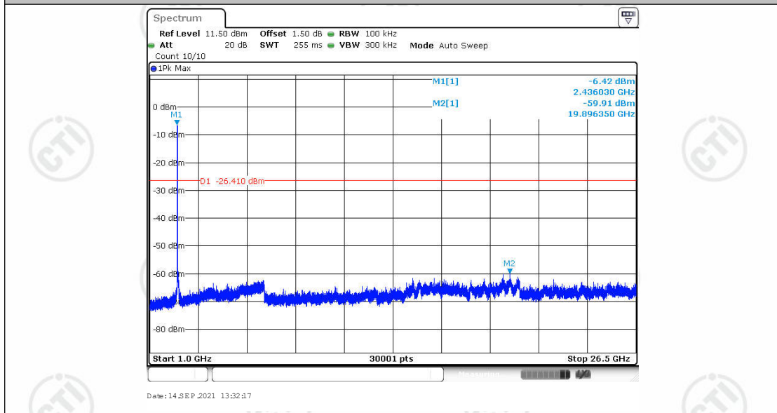
11N20SISO_Ant1_2437_1000~26500
