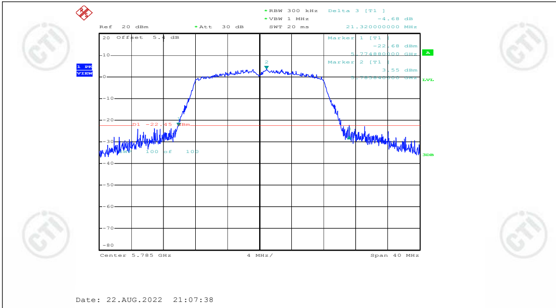
11A_Ant1_5785
