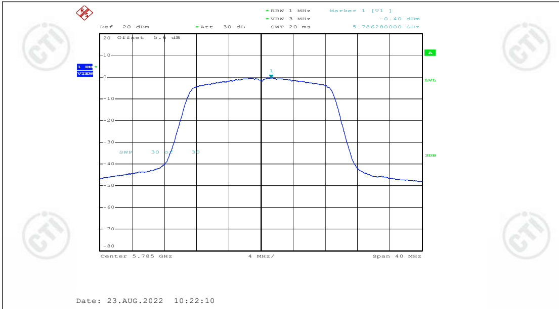
11AC20SISO_Ant1_5785
