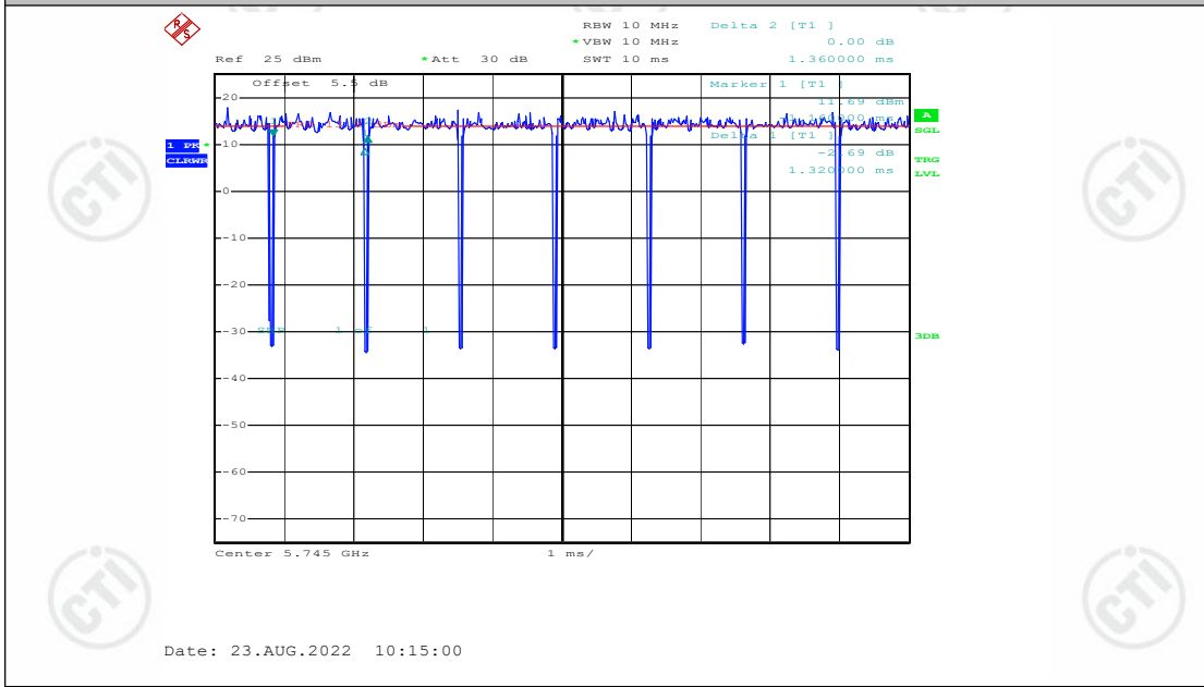
11AC20SISO_Ant1_5745
