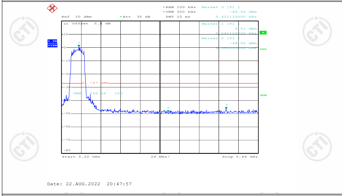
11A_Ant1_High_5240
