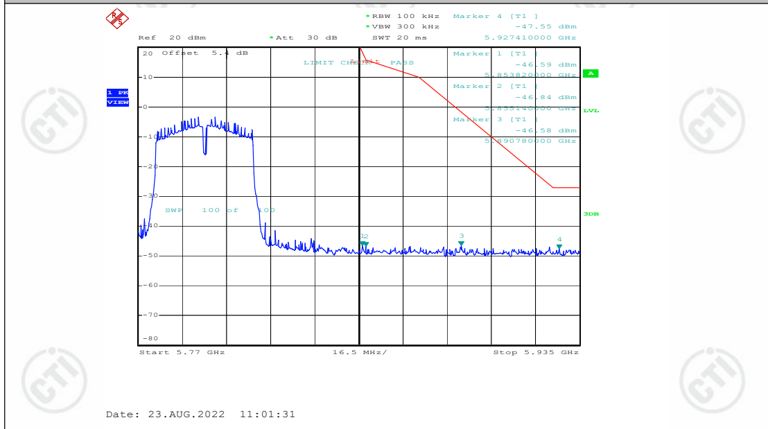
11AC40SISO_Ant1_High_5795
