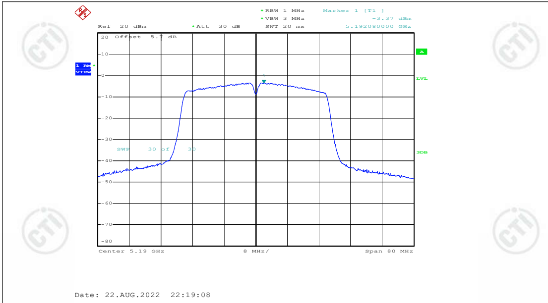
11N40SISO_Ant1_5190
