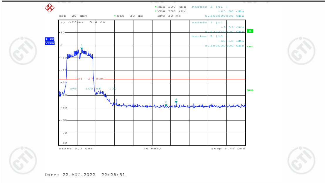
11N40SISO_Ant1_High_5230
