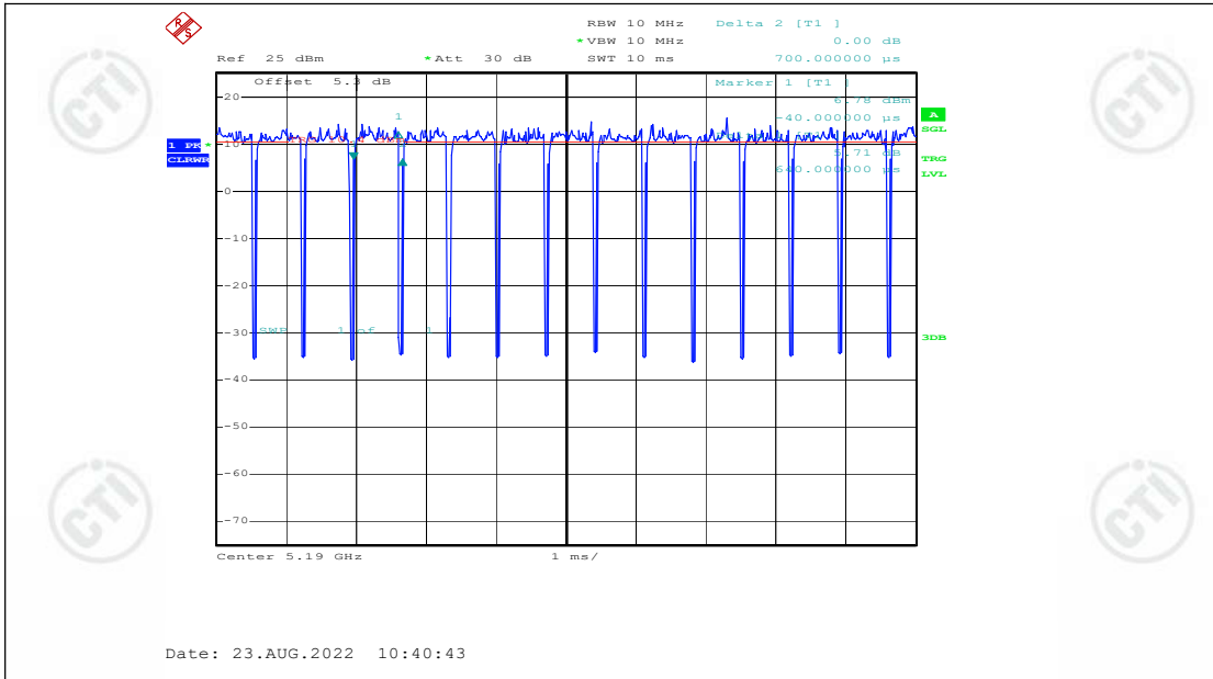
11AC40SISO_Ant1_5190
