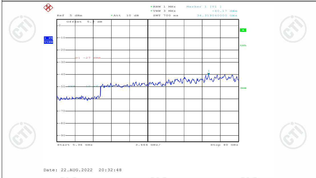
11A_Ant1_5180_5360~40000
