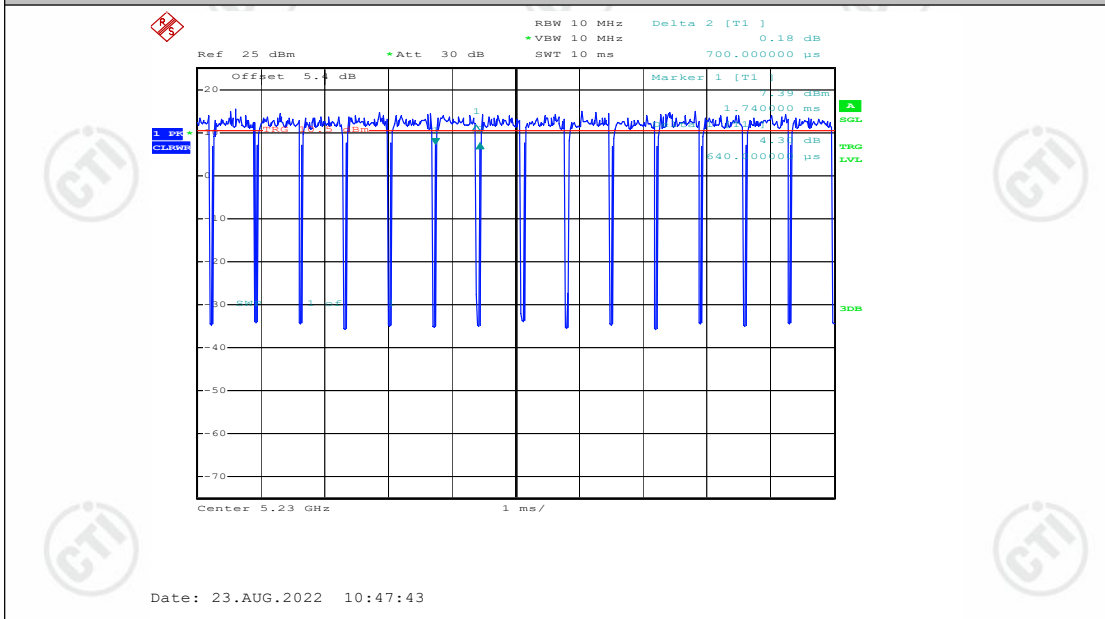
11AC40SISO_Ant1_5230
