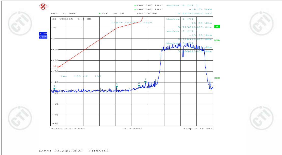
11AC40SISO_Ant1_Low_5755
