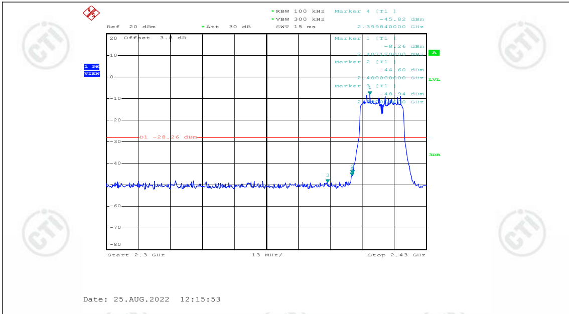
11N20SISO_Ant1_Low_2412
