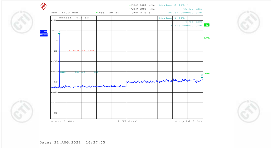
2DH5_Ant1_2441_1000~26500
